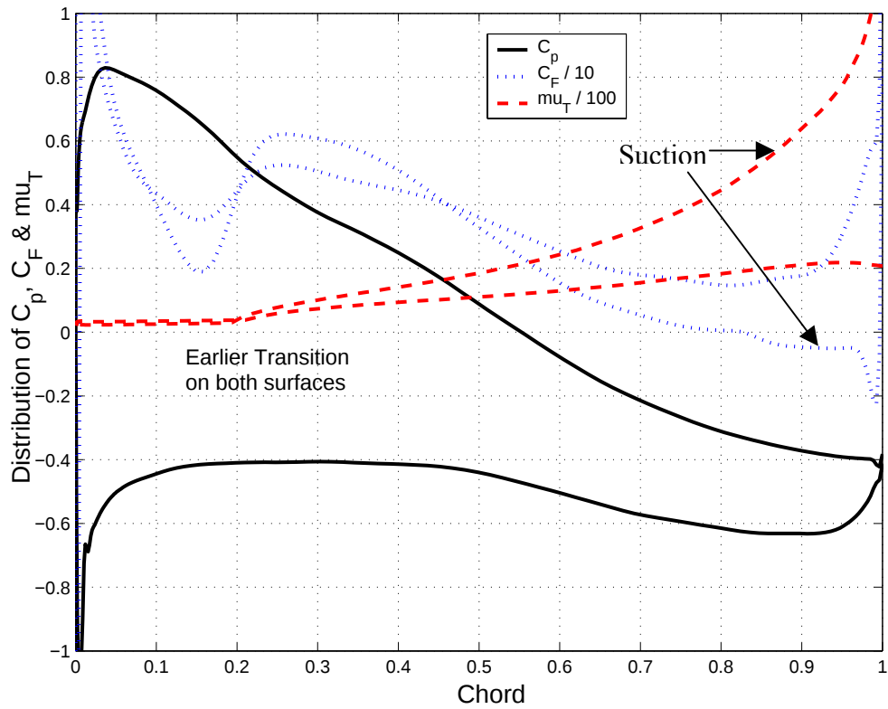
Figure 14. Separation / Transition Sensitivity Study: Distribution of Pressure Coefficient ( C_p ) Skin Friction ( C_F ) and Turbulent viscosity ( \mu_T or \mu_{u_T} ) - (Low Re/Low Tu)
