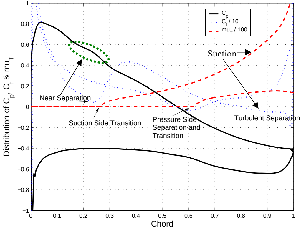
Figure 12. Separation / Transition Sensitivity Study: Distribution of Pressure Coefficient ( C_p ) Skin Friction ( C_f ) and Turbulent viscosity ( \mu_T or \mu_T ) - (Low Re/Low Tu)
