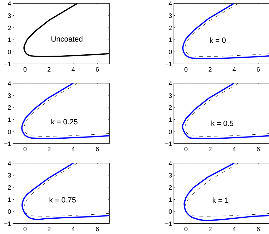
Figure 17. Leading Edge Profiles (scale is % chord).
