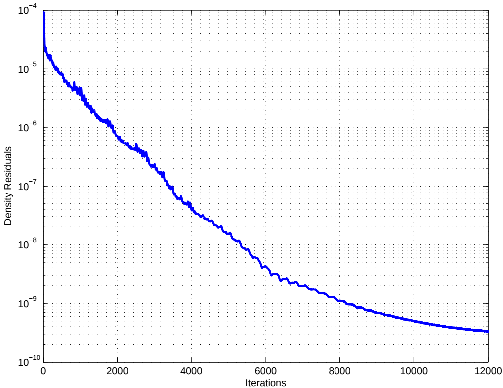
Figure 6. Typical Density Residual plot.
