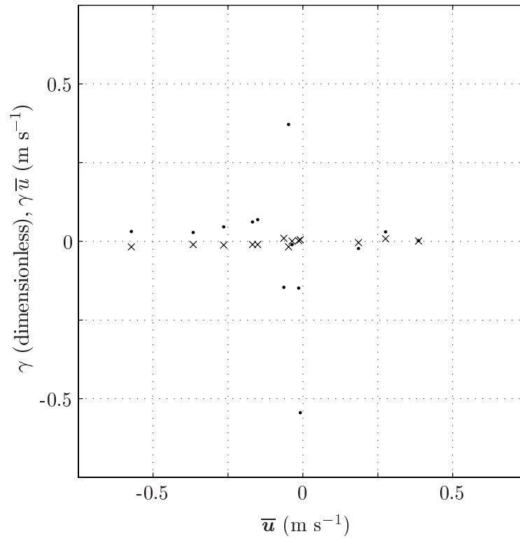
Figure 5.2: Velocity-conductivity covariance calculated from absolutely referenced geostrophic velocity profiles and hydrographic data (see section 4.4 for details). \gamma is shown by •, and \gamma \bar{u} = \overline{\sigma' u'} / \bar{\sigma} by ×.
