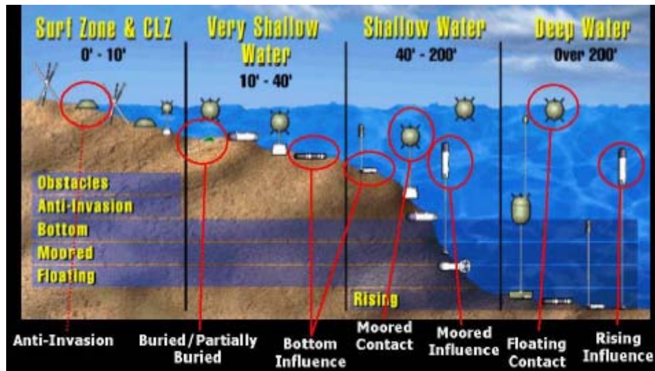
Figure 2. Mine Types Used in Various Situations (From Nawara)
