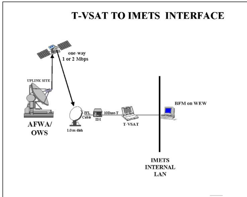
Figure 2. Data flow from AFWA OWS hub to IMETS, with Mbps rates for the continental U.S.
