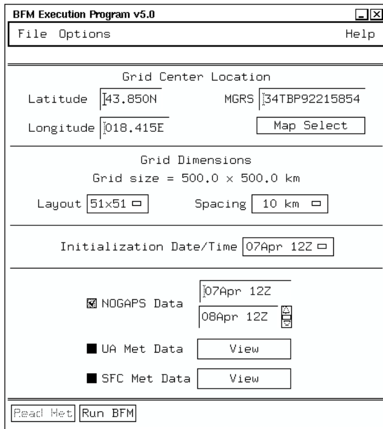
Figure 1. Sample GUI for the BFM execution used on IMETS.
