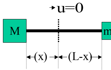
Figure 6. MiniCan modeled as a mass-loaded bar.
