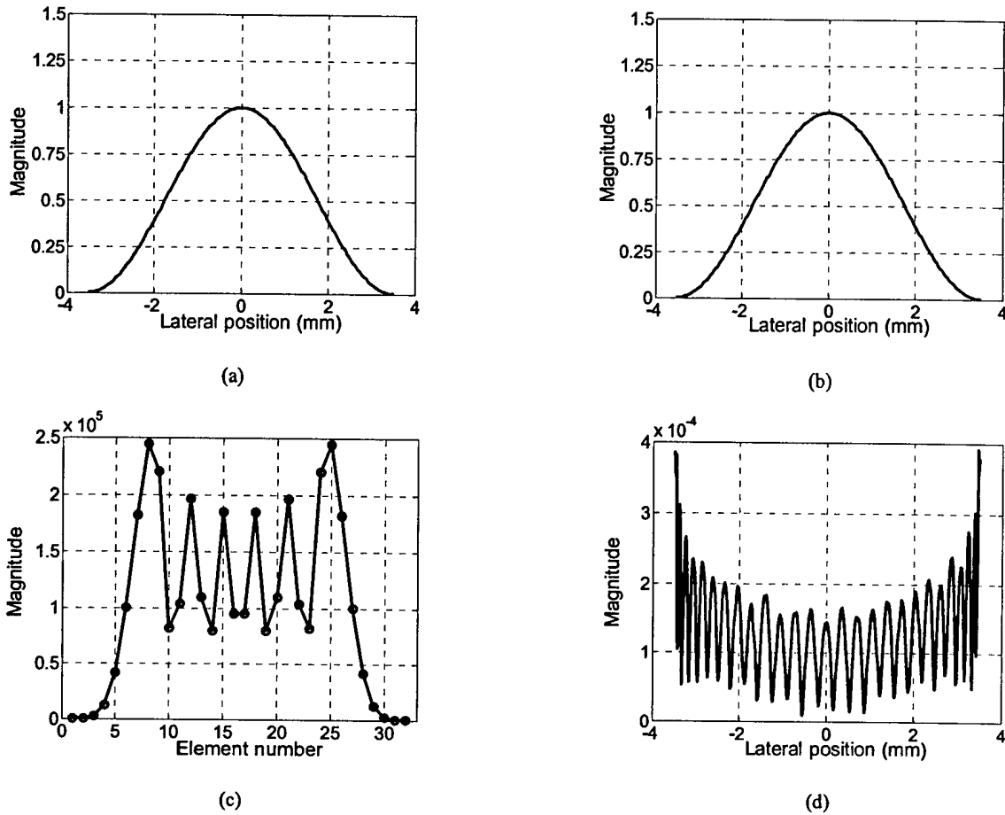
Figure 3. CW one-way design example showing (a) the goal psf as a function of lateral position, (b) the system psf obtained with the MSSE technique as a function of lateral position, (c) the calculated transmit weights as a function of element number, and (d) the error between the goal and the MSSE technique psfs as a function of lateral position.
