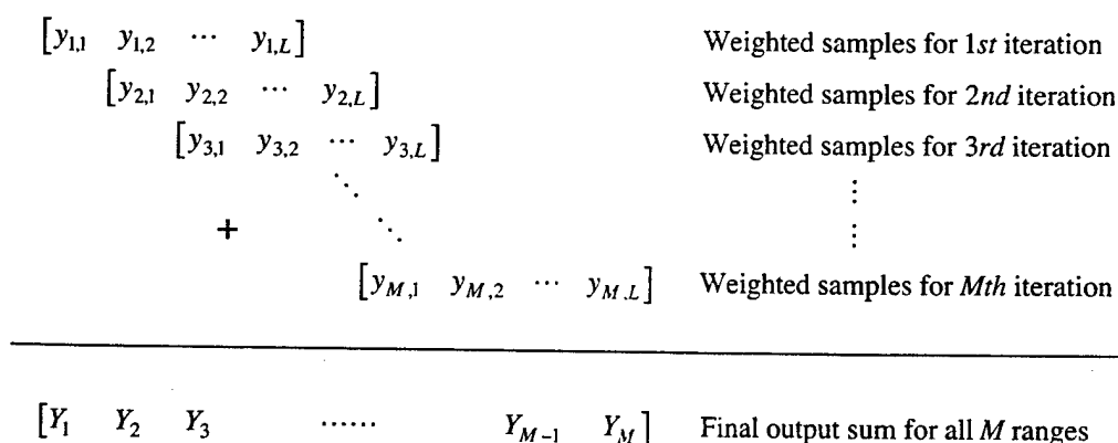
Figure 3. Representation of MI-CAB output for one full image line by overlap-add. Each row represents one iteration of the algorithm. M is the total number of ranges in the input RF data.
