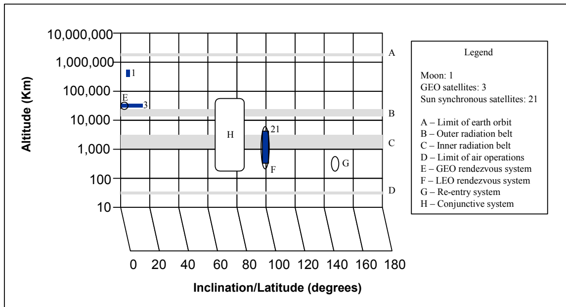
Figure 3. Spacecraft Performance Ranges
