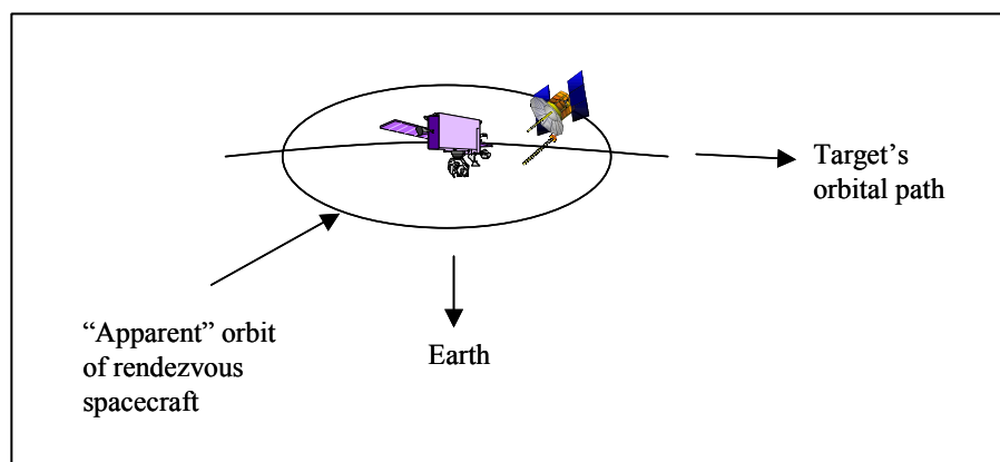
Figure 7. The Rondure
