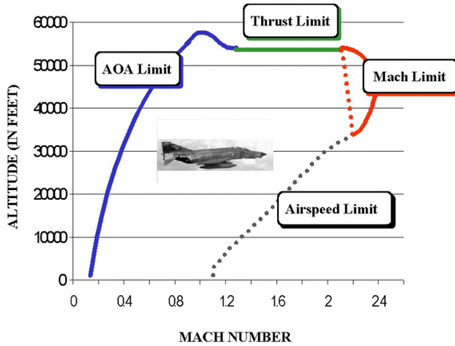
Figure 5. F-4 Flight Envelope
