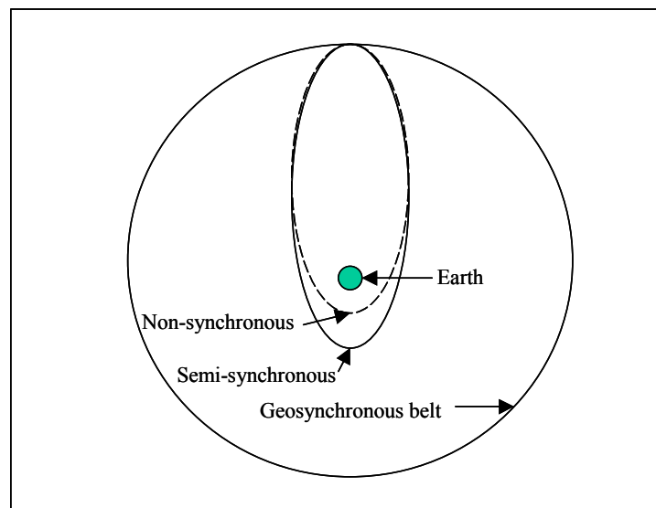
Figure 8. Osculatory Orbits
