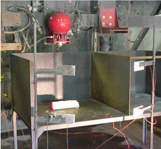
Figure 8: Suppression System and Table with M3 Propellant
