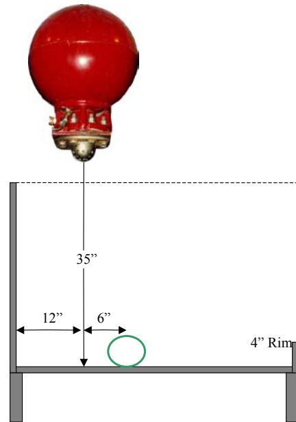
Figure 13: Tests 5-7 Setup
