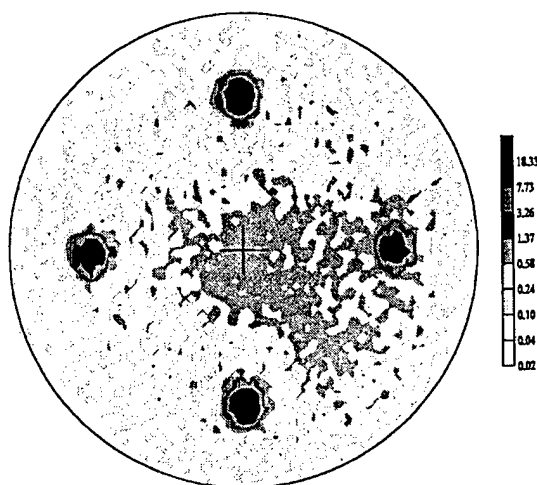
Fig.1. Y 2 O 3 (222) pole figure on log scale
