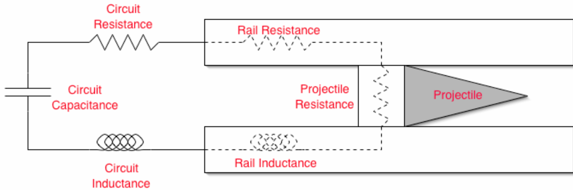
Figure 3.10. Capacitor Driven Railgun Circuit
