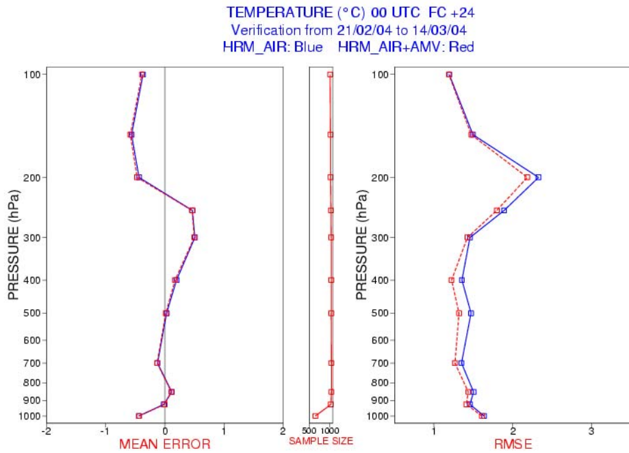
Figure 4.24 Temperature ME and RMSE of EUROHRM forecasts from CNMCA 3DVar analysis using aircraft observations with (red) and without (blue) the ingestion of AMV data verified against radiosoundings: T+12h (top) and T+24h (bottom).
