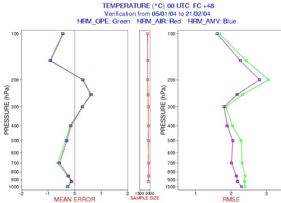
Figure 4.17 Temperature ME and RMSE of EUROHRM forecasts from CNMCA 3DVar analysis without (green) and with the ingestion of aircraft (red) or AMV (blue) data verified against radiosoundings: T+36h (top) and T+48h (bottom).
