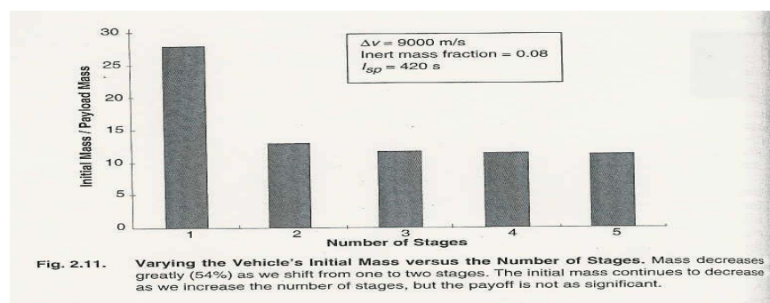
Figure 7 Staging Impact Upon Vehicle Mass 109
