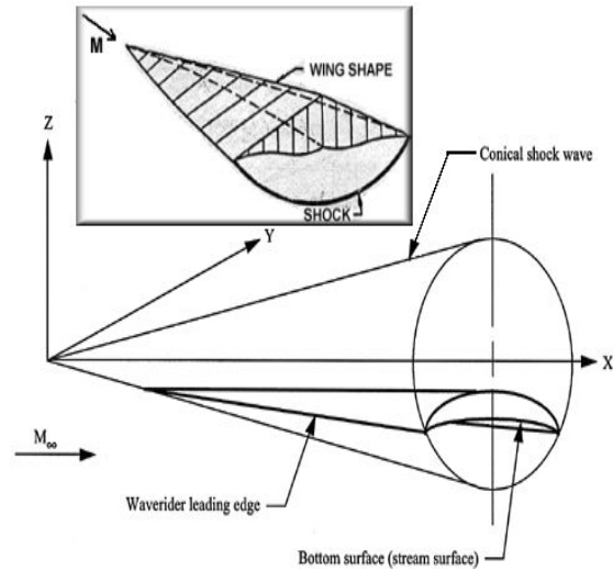
Figure 19 Construction of a Body “Waverider” Producing a Conical Shock 221
