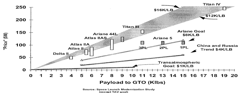
Figure 10 ELV Space Launch Cost Trendlines 142
