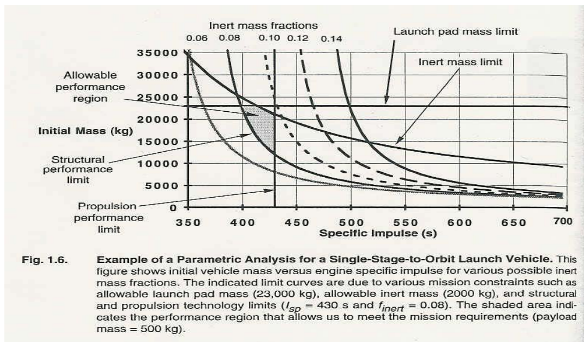
Figure 9 Parametric Analysis of a Single-Stage-to-Orbit Vehicle
