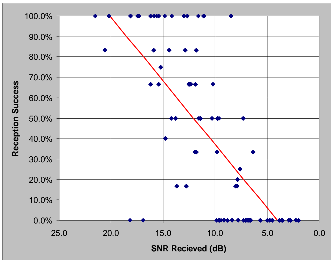
Figure 12. Reception success rate plotted against received SNR for each transmission. Data points are weighted according to number of subpackets sent. The red line is a linear regression of all 80 data points.
