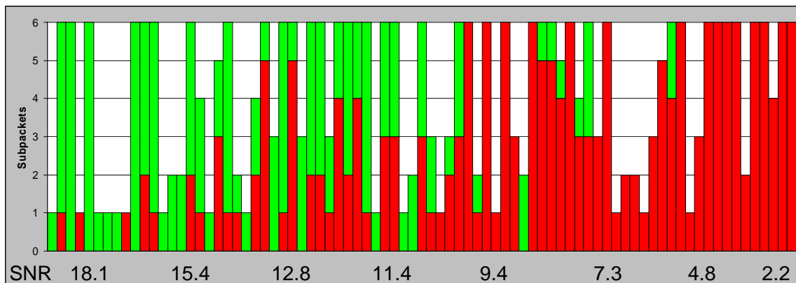
Figure 11. For all data at all three ranges, each independent transmission is displayed in order of decreasing SNR. Note that the plot is not linear with respect to SNR.
