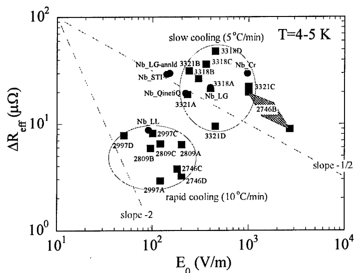
Figure 14. Parametric plot monitoring the dielectric loss tangent and the saturation field of MgO for T \sim 4 K. The plot contains data for YBCO films (red colour) as well as for Nb reference films (blue). The effect of slow cooling in terms of enhanced \Delta R_{\text{eff}} and tendentially increased E_0 is clearly visible. The dashed lines are guides to the eye (c.f., [6]).
