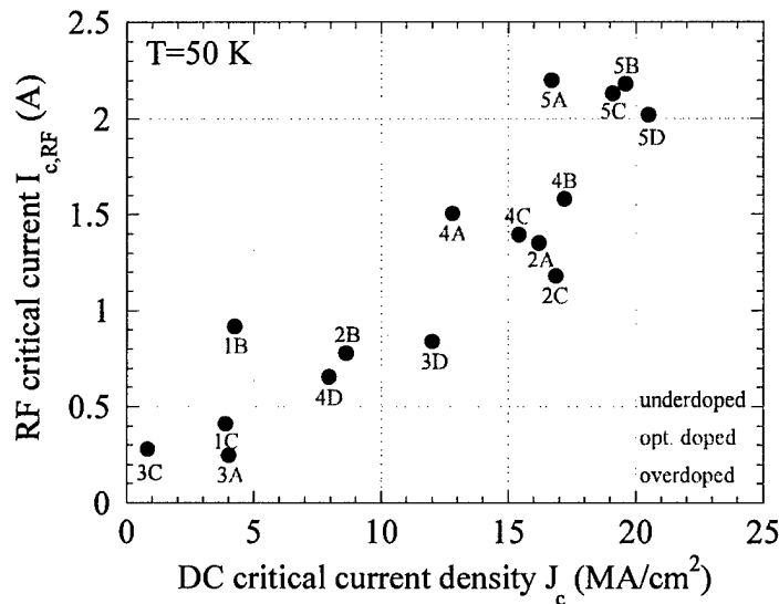
Figure 7. Correlation between the RF critical current and the DC critical current density for T = 50 K. I_{c,RF} increases almost linearly with J_c , with a slope \sim 0.1 \text{ A}/(\text{MA}/\text{cm}^2) . The four films of batch #5 (table I) display the highest critical parameters of all samples studied until now.
