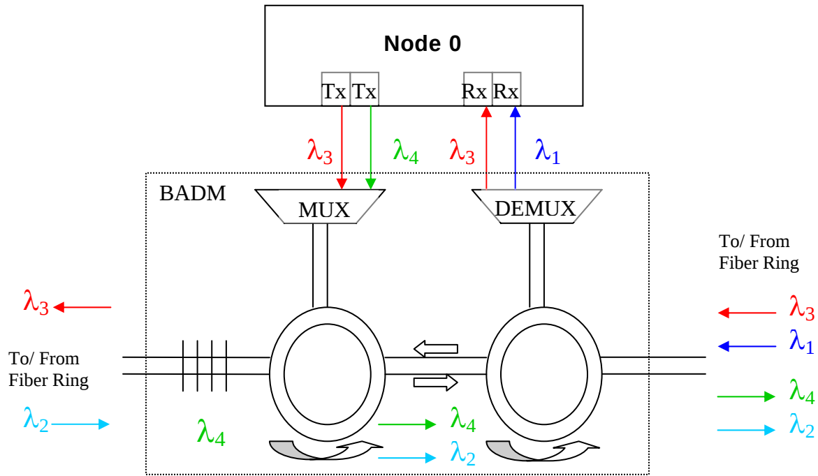
Figure 10: Design for a bi-directional, multi-wavelength ADM.
