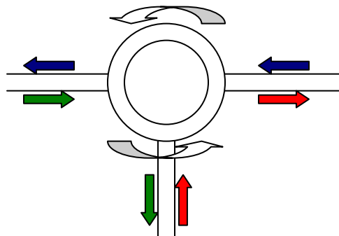
Figure 6: Three-port circulator
