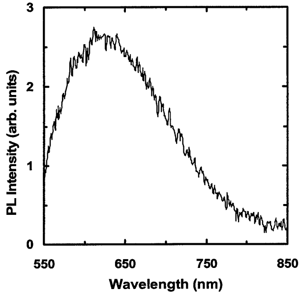
Figure 4.4. PL spectra of black silicon at 300 K.
