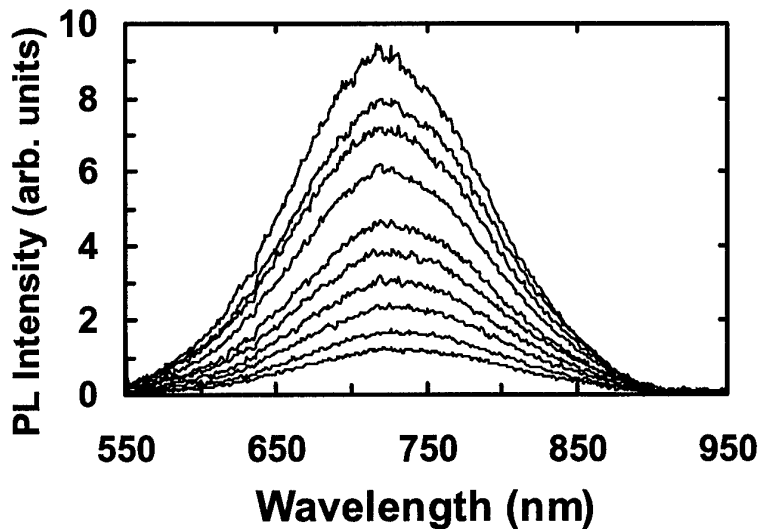
Figure 3.6. PL spectra of the porous silicon 1.4 – 5.75 W cm -2 laser intensity range at 10 K.
