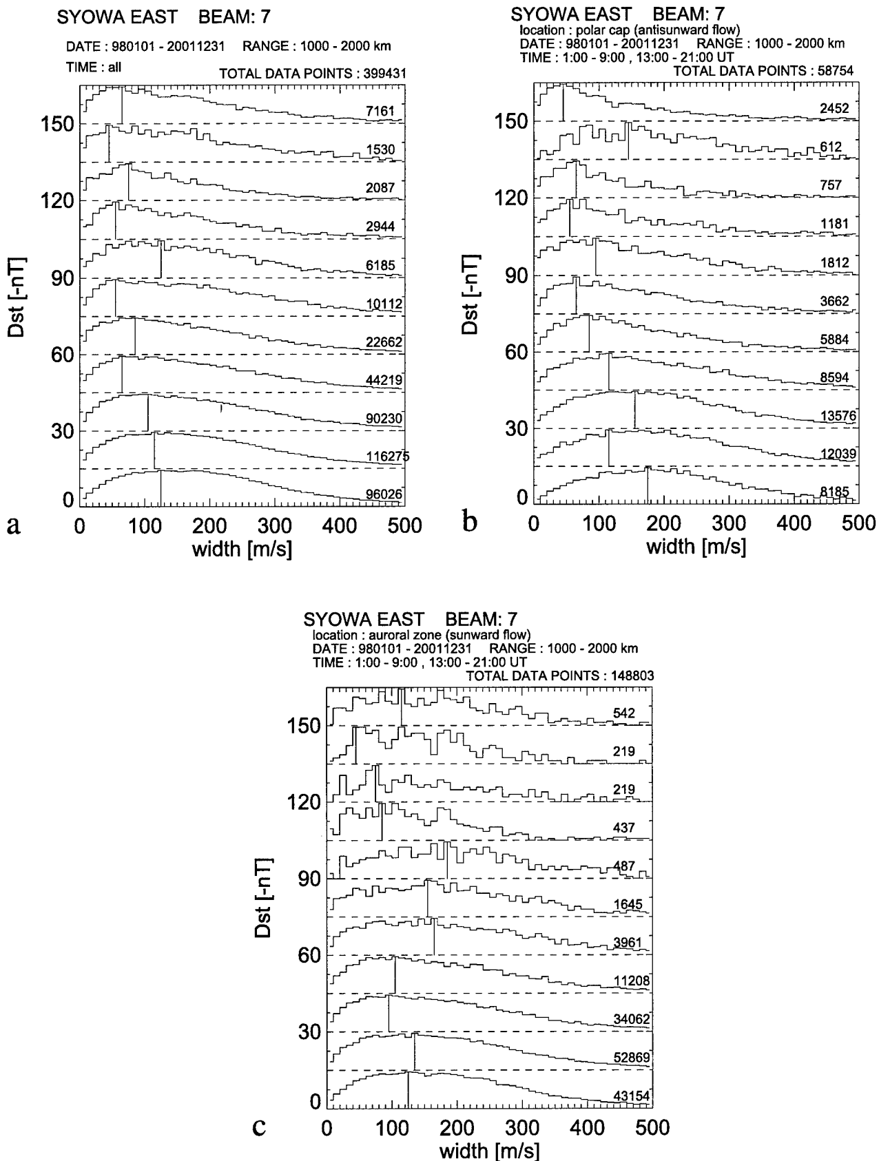
Figure 4. Distribution of the spectral width of ionospheric backscatter echoes for |vel| \geq 450 m/s, binned for Dst ranges every 15 nT, obtained by beam 7 of the Syowa East radar. The plots are shown for all the data (a), polar cap data corresponding to the antisunward flow (b), and auroral zone corresponding to the sunward flow (c). The peak value of each distribution is indicated by a vertical line.
