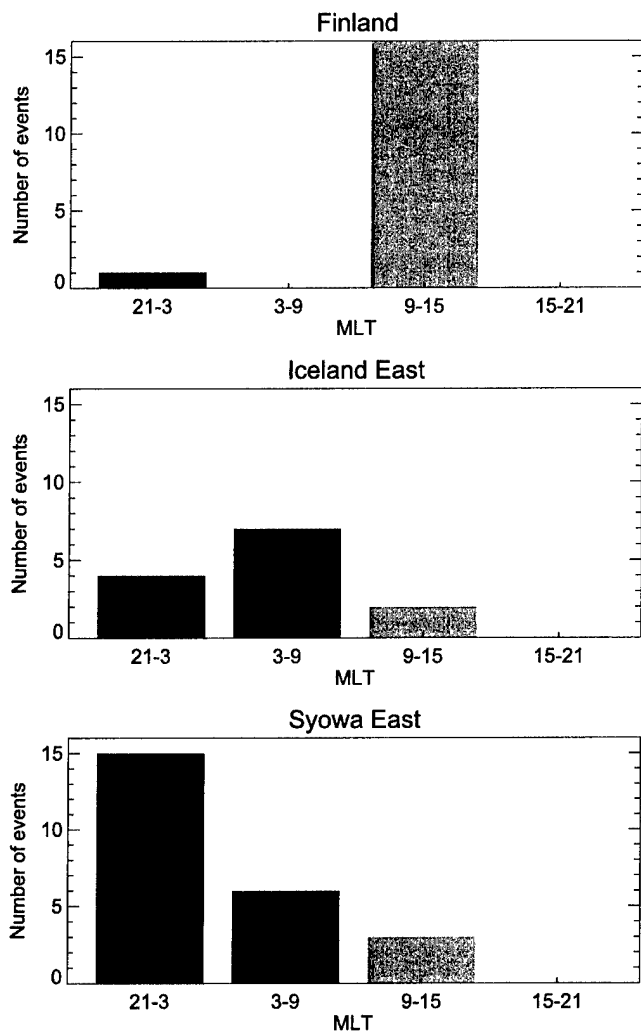
Figure 16. Distribution of MLT for the events of ionospheric echoes with high velocities ( >450 m/s) and very low spectral widths ( <60 m/s).
