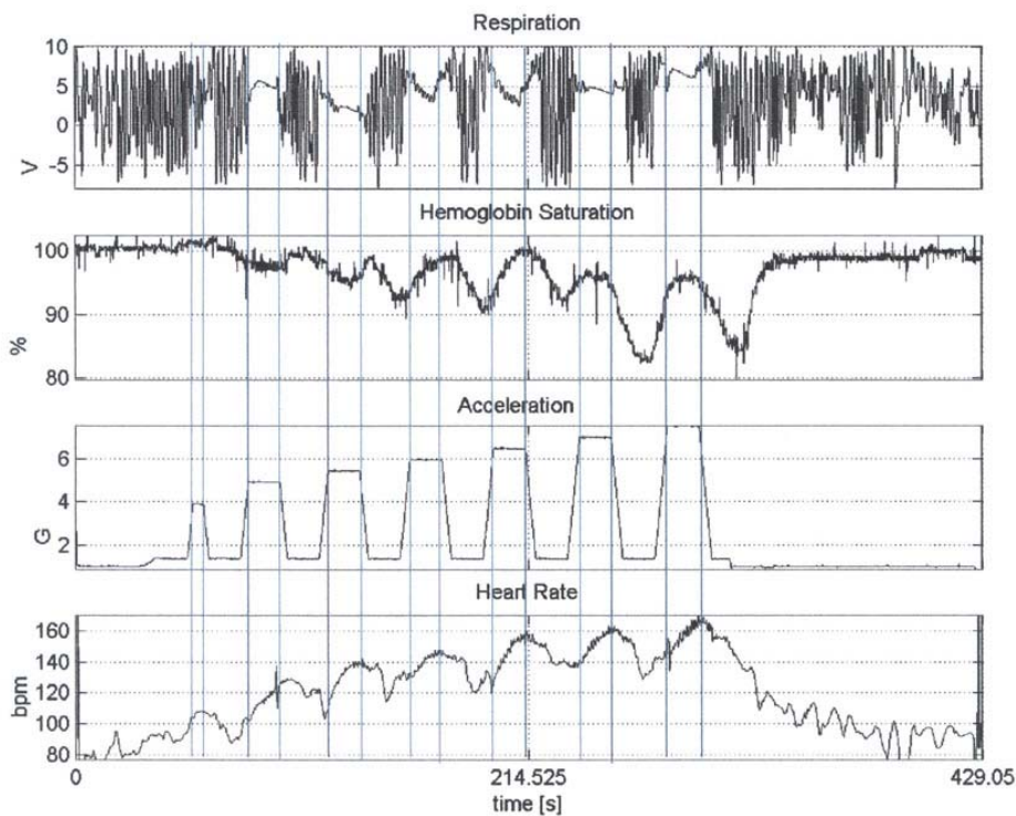
Fig. 14 Second examination of subject 1
