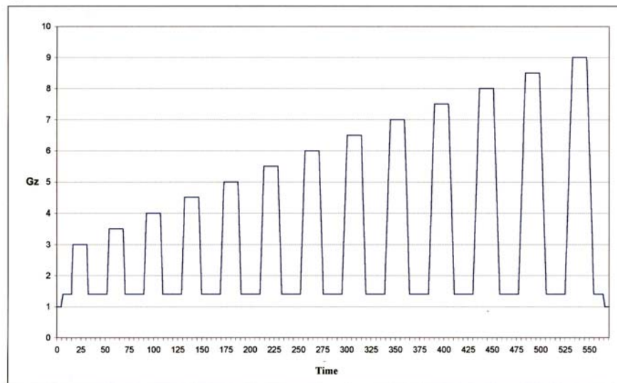
Fig 3 - Programs of GOR and ROR profiles
