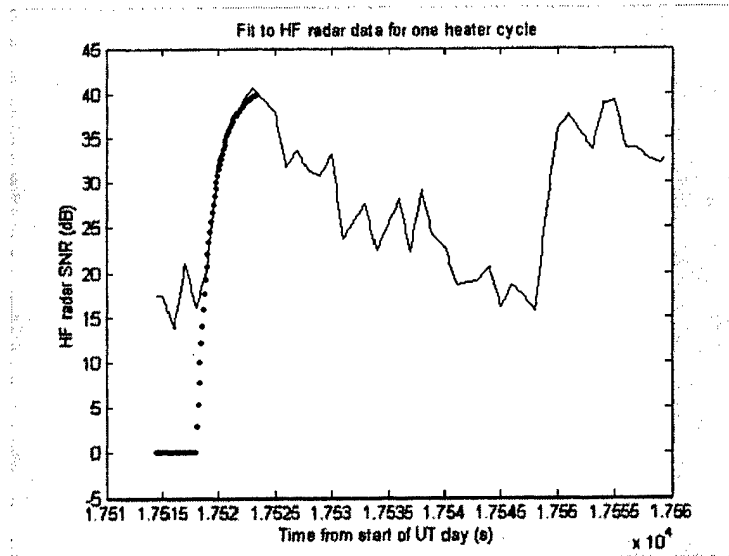
Figure 27. Optimal Non-linear Least-squares Fit an HF Radar Observation of a HAARP Heater Cycle. This Fit Corresponds to the Formation of FAI.
