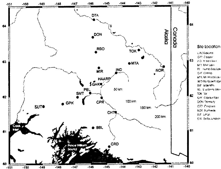
Figure 4. Remote Field Sites Used for Antenna Pattern Measurements, Plus the Gakona Reference Site (GAK) and the HAARP Location (HAARP). The Legend at the Right Refers the Site Designations to Their Names.
