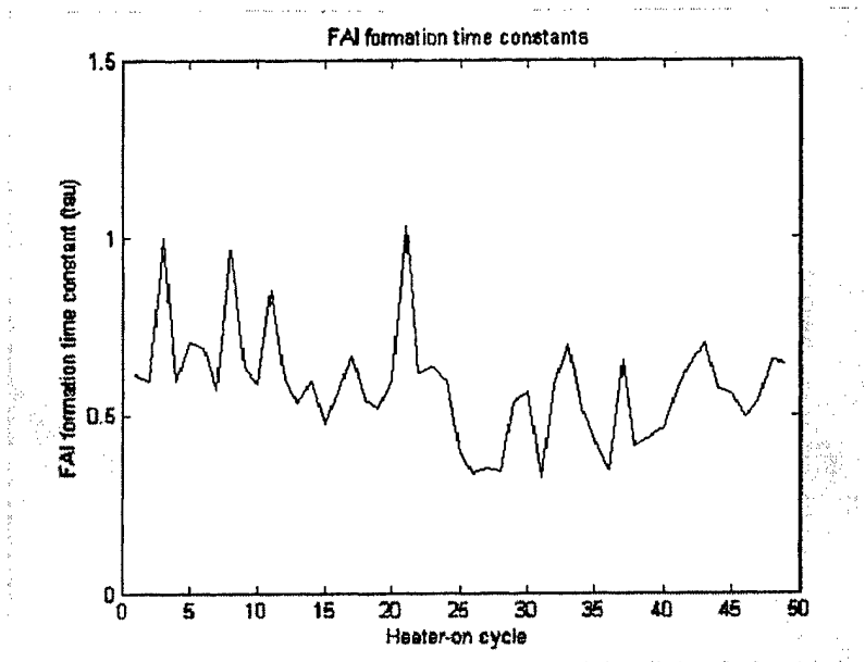
Figure 28. FAI Formation Time Constants for Each of the 50 Heater On-Off Cycles.
