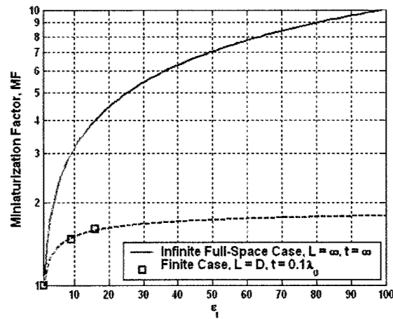
Figure 4.22 Miniaturization factor limitations as a function of dielectric constant for double-sided loading (thickness = 0.1\lambda_0 )
