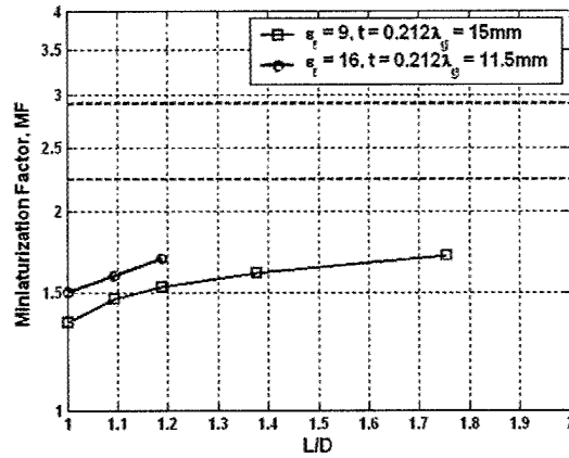
Figure 4.5 Impact of superstrate width on MF.
