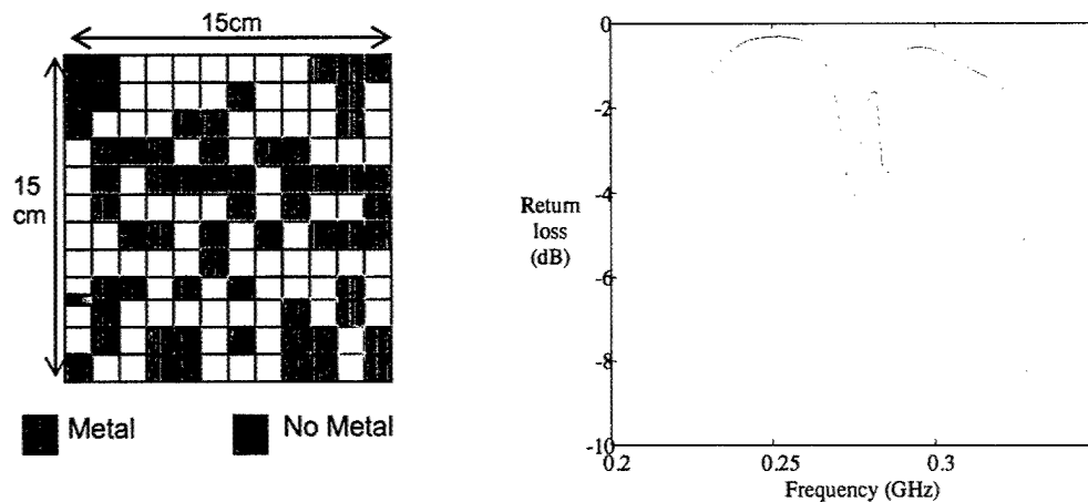
Figure 6.3 Initial antenna structure of 1 st design step: Horizontally fed strip antenna with fixed cavity size and material composition. Design variables correspond to on/off (1/0) conductor metallization pattern.
