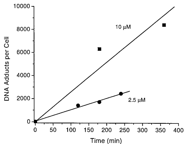
Figure 3 Formation of 11 \beta -DNA adducts in LNCaP cells treated with [ 14 C]-11 \beta (—■— 10 \mu M; —●— 2.5 \mu M)
