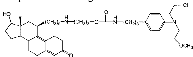
Figure 1 Monochloro 11 \beta
