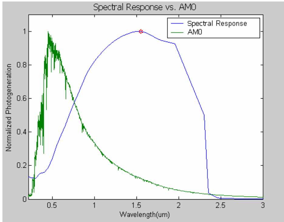
Figure 35. Spectral Response of InGaAs
