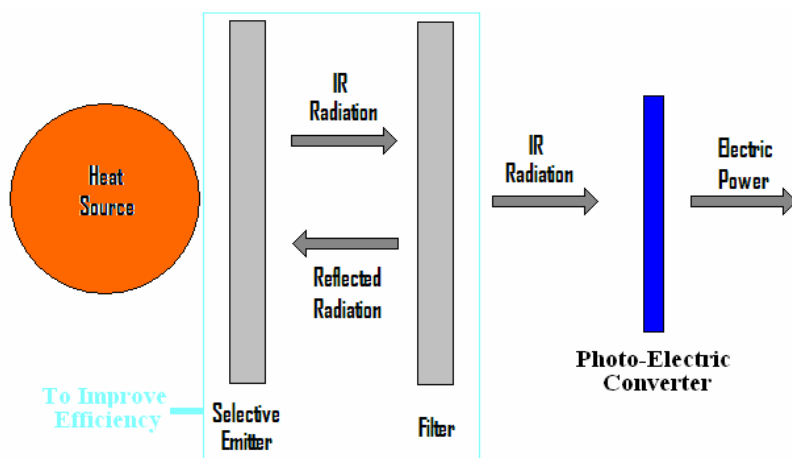
Figure 13. TPV System
