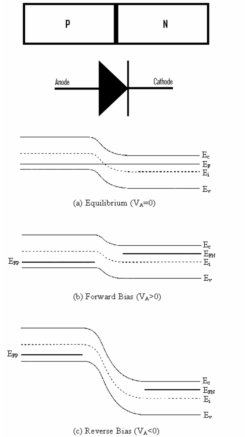
Figure 4. p-n Junction Under Bias [After Ref. 2.]
