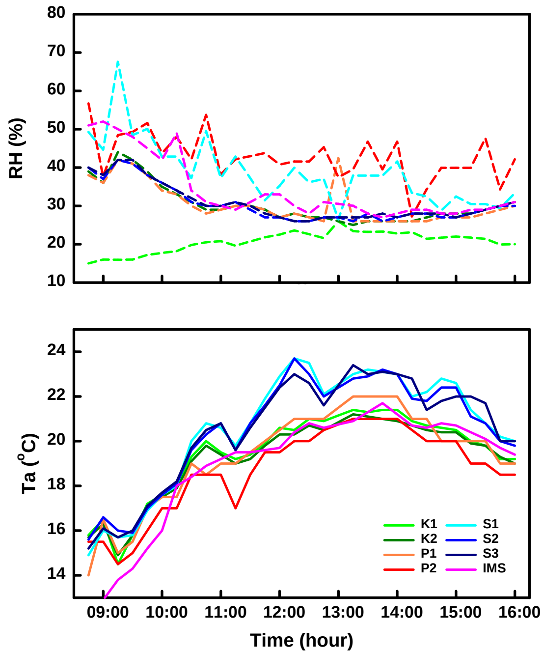
Figure 10. WAPEM's relative humidity (top) and ambient temperature (bottom) measurements ( S_1 , S_2 , S_3 ) compared with Kestrel ( K_1 , K_2 ), Psychrometer, and IMS measurements ( P_1 , P_2 ) from Yotveta (Negev Desert).
