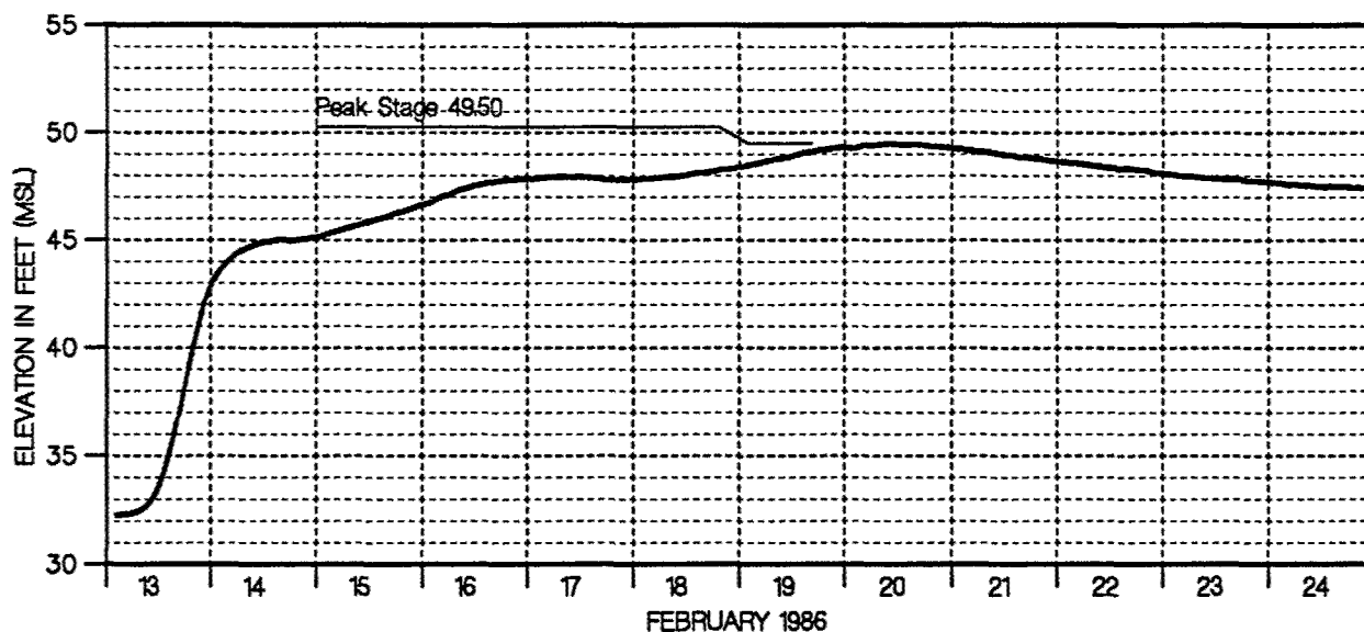
SACRAMENTO RIVER AT WILKINS SLOUGH
