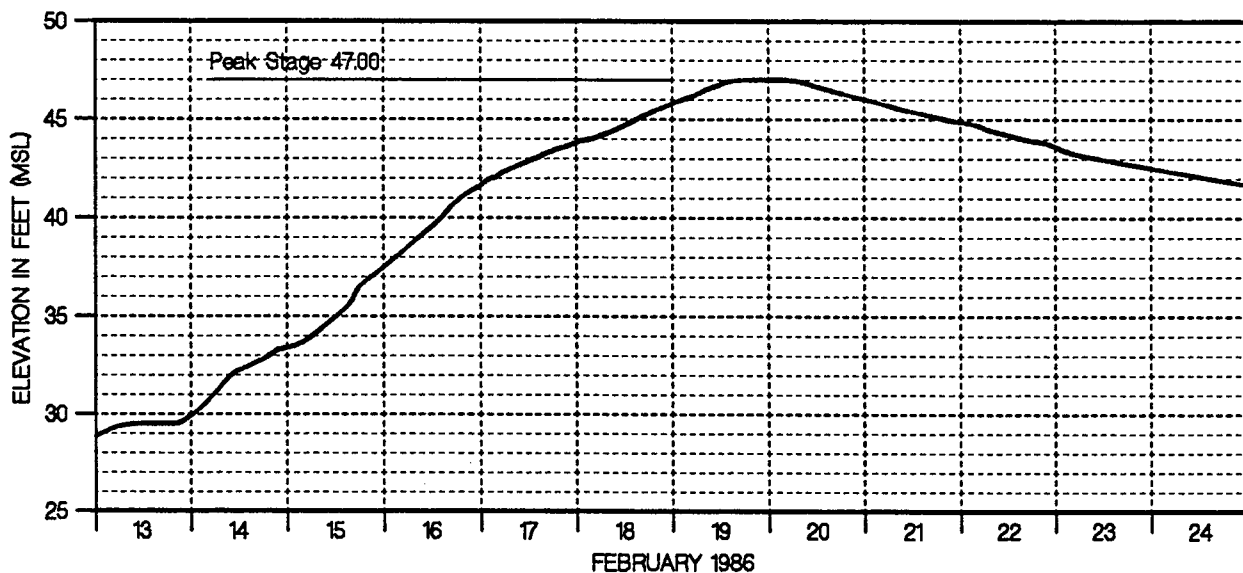
SUTTER BYPASS AT TISDALE BYPASS
