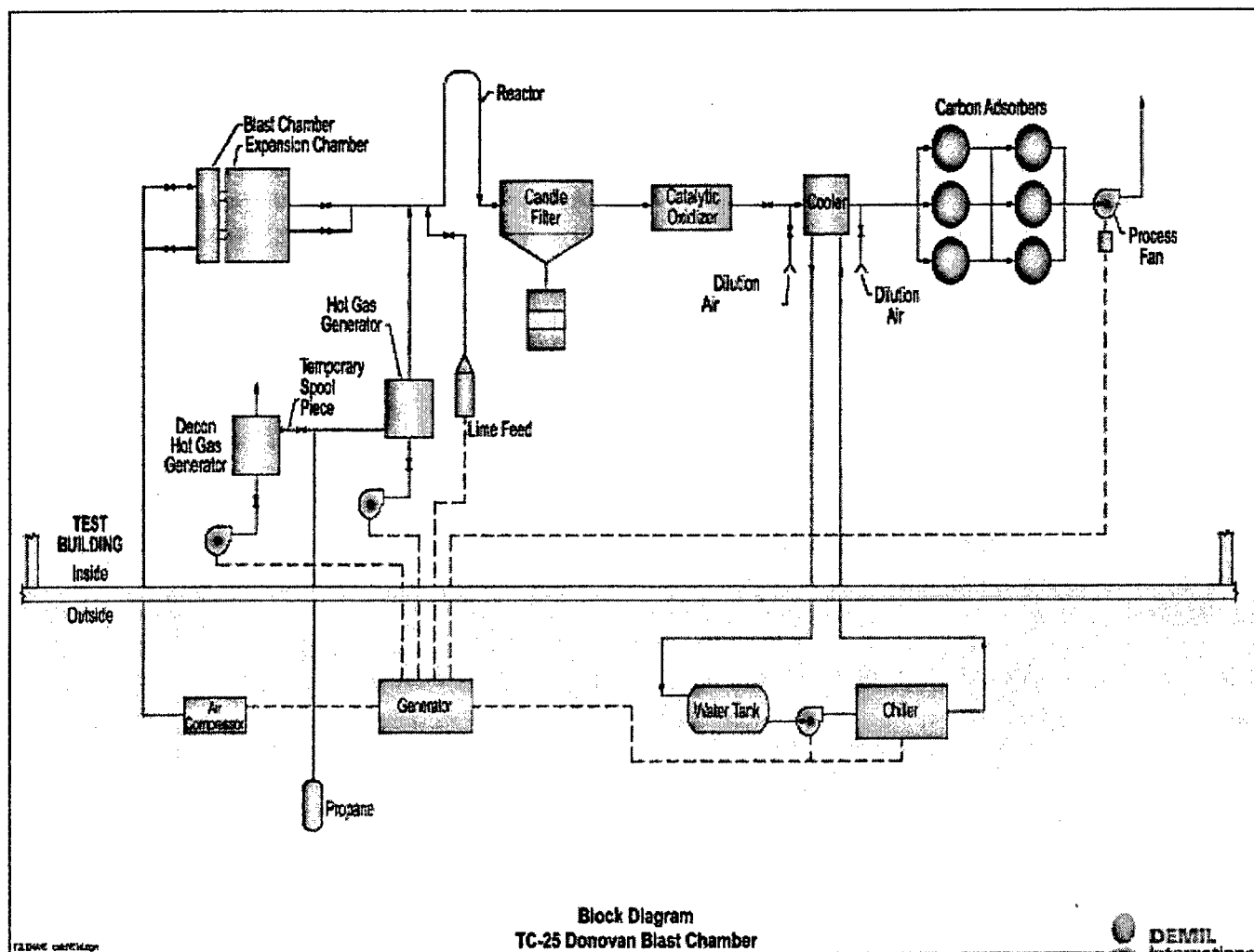
Figure 1. TC-25 DBC System Layout
