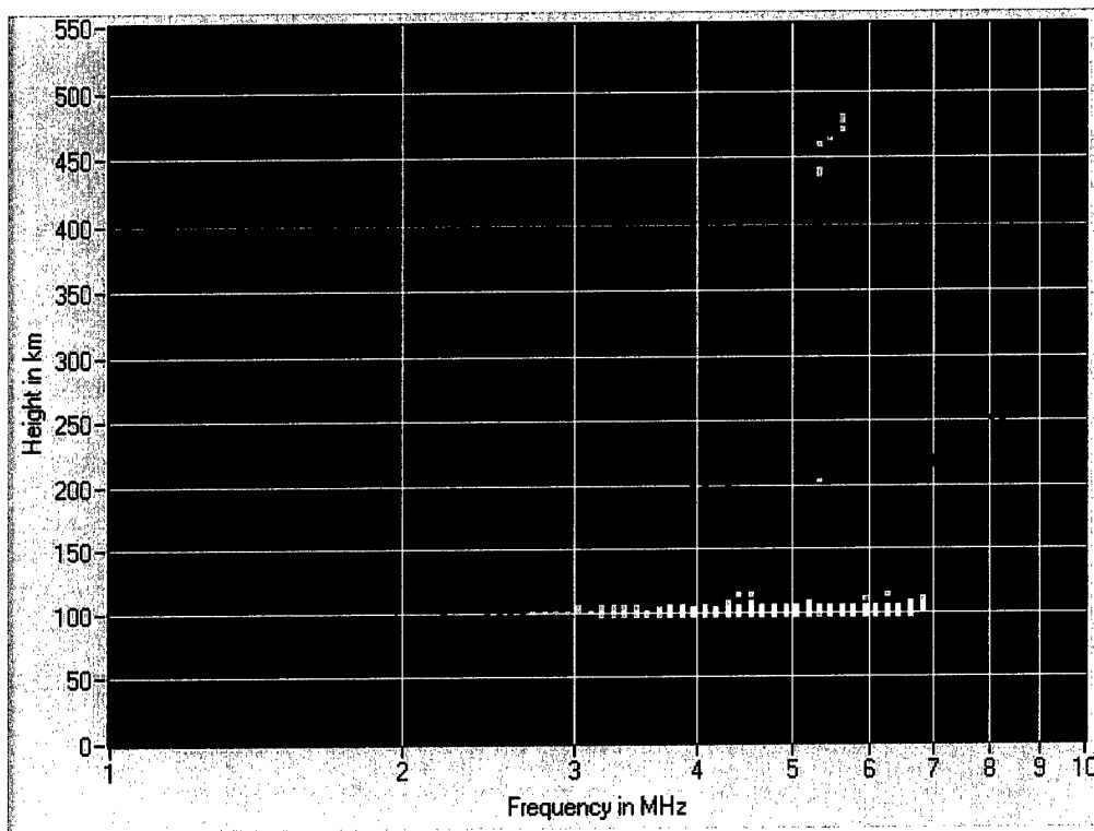
Figure 3: Thin sporadic-E blanketing; taken on August 29, 2000, hour 18:00 UT at Cape Race.
