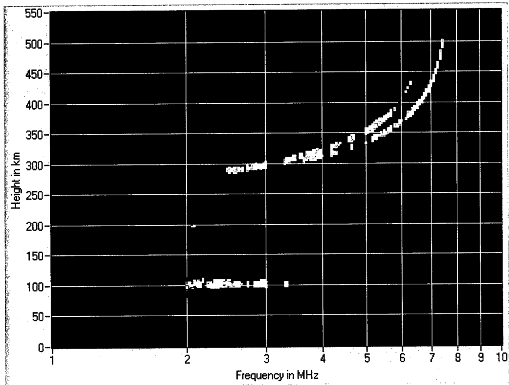
Figure 6: Ionogram comparison to HFSWR data. The ionogram taken on August 30, 2000, hour 02:00 UT at Cape Race.
