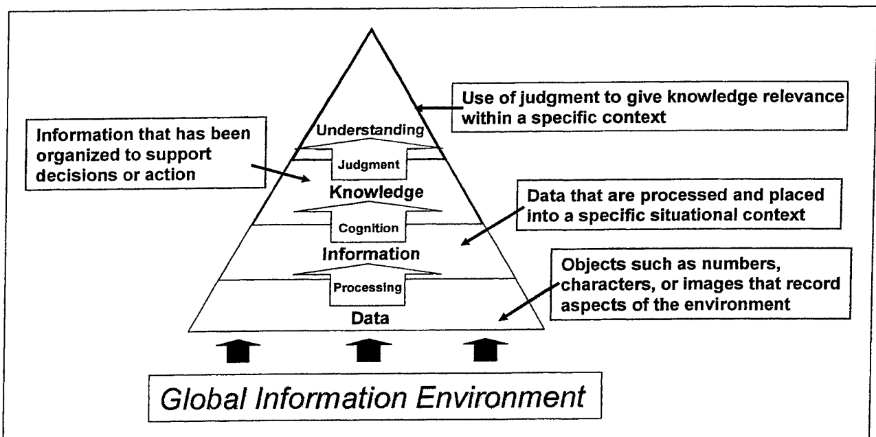
Figure 1. Cognitive hierarchy.
