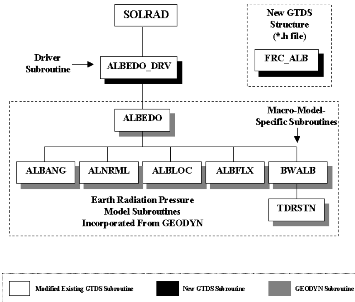
Figure 6-4 – Software Design Tree for Incorporation of GEODYN Earth Radiation Pressure Model (Earth Albedo and Earth IR) Subroutines into GTDS
