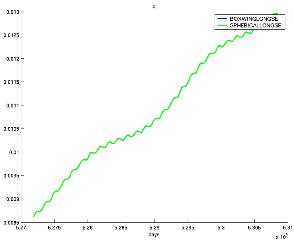
Figure A-9 – One-year Mean Element Plots of p and q (Vernal Equinox)
