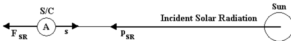
Figure 1-3 – Solar Radiation Pressure Acting on a Spherical Spacecraft Model
