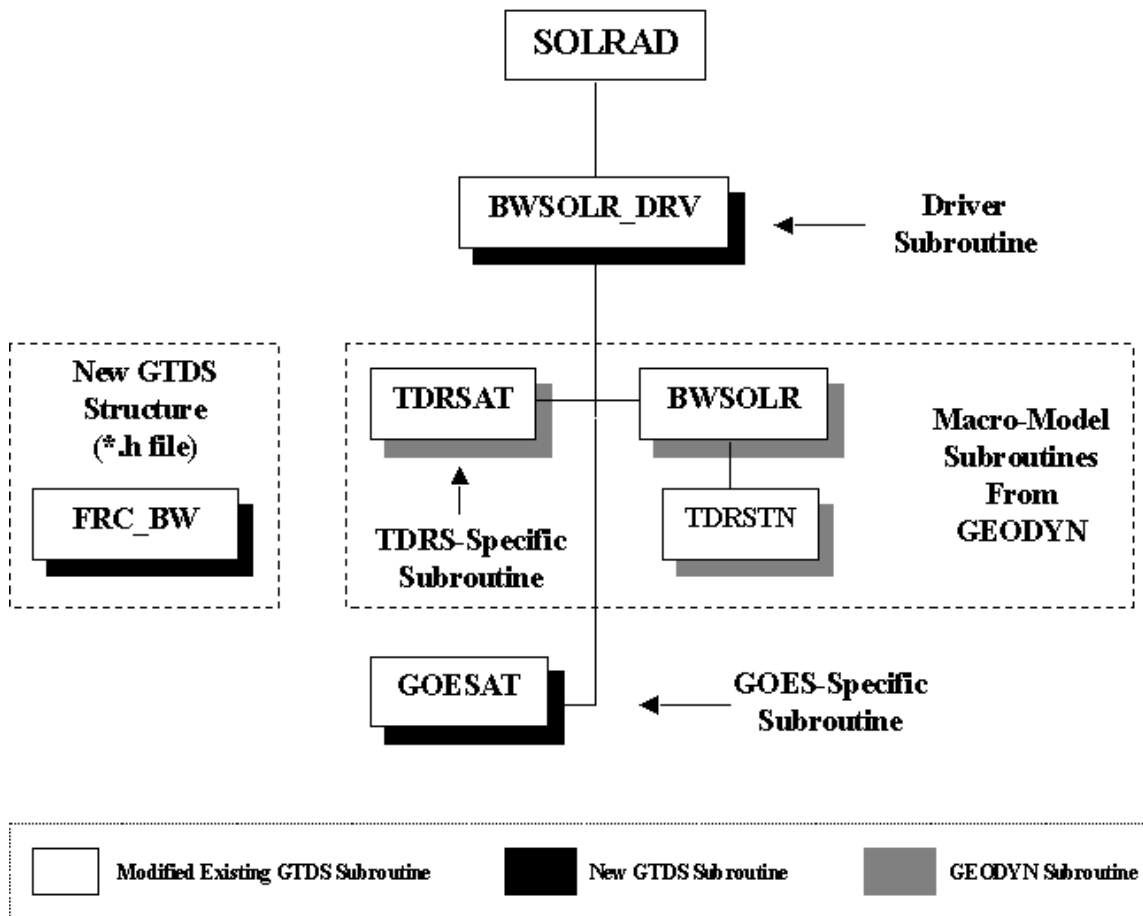
Figure 6-3 – Software Design Tree for Incorporation of GEODYN Solar Radiation Pressure Model Subroutines into GTDS
