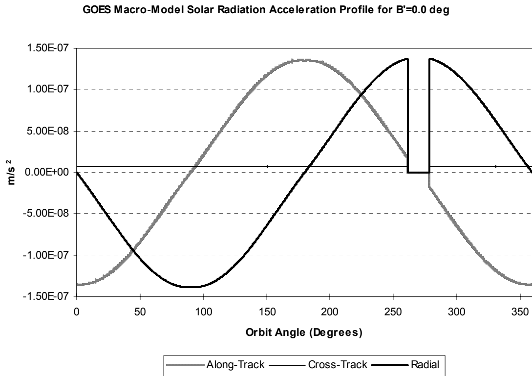
Figure 7-9 – UNIX GTDS GOES Macro-model Solar Radiation Acceleration Profile for \beta' = 0^\circ
