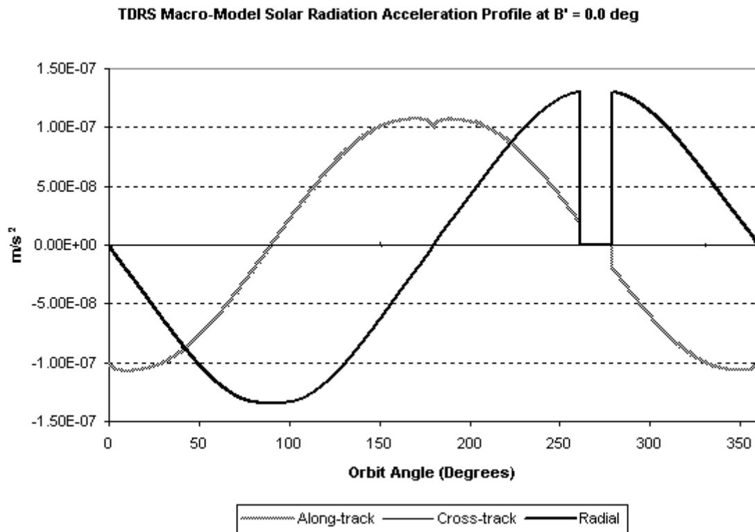
Figure 7-5 – UNIX GTDS TDRS Macro-model Solar Radiation Acceleration Profile for \beta' = 0^\circ
