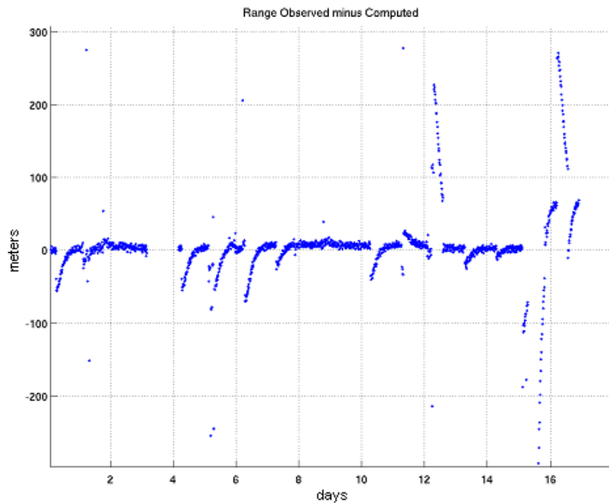
Figure 8-25 – GOES Station 6 Range Residuals vs Time using SSN and NOAA Ranging Data with Box-wing Model (ESKF)
