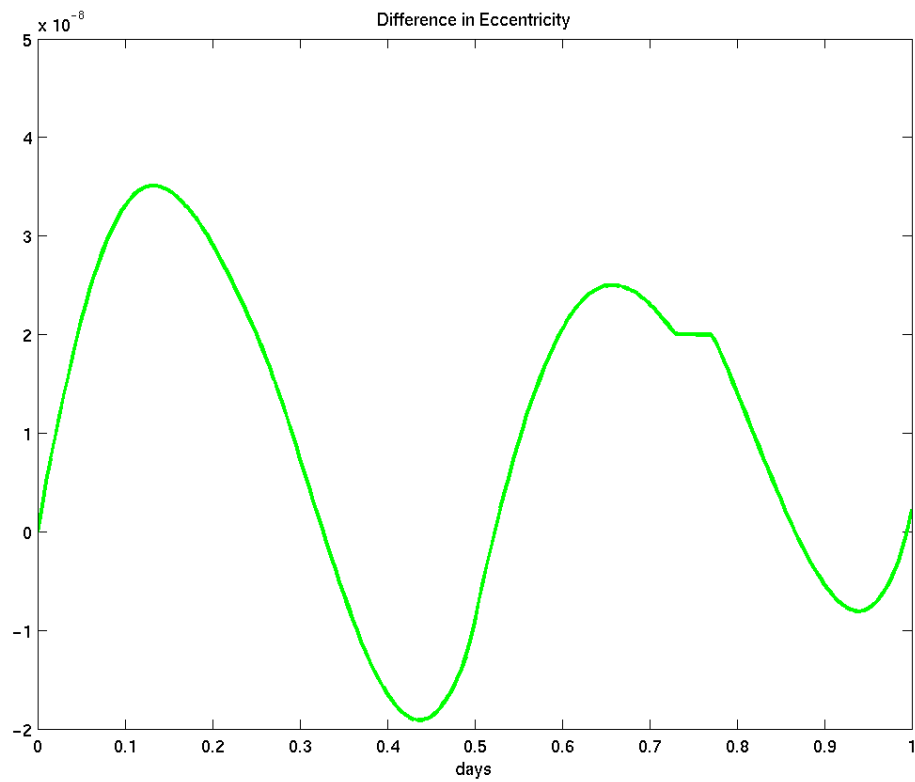
Figure A-4 – Box-wing – Spherical Difference in a and e (Autumnal Equinox Case)
