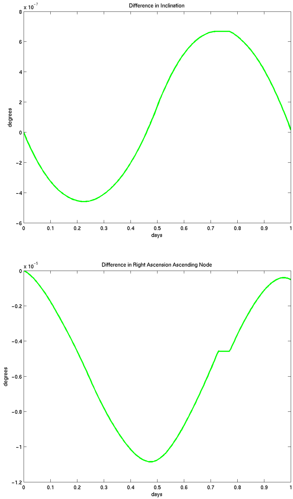
Figure A-5 – Box-wing – Spherical Difference in i and \Omega (Autumnal Equinox Case)
