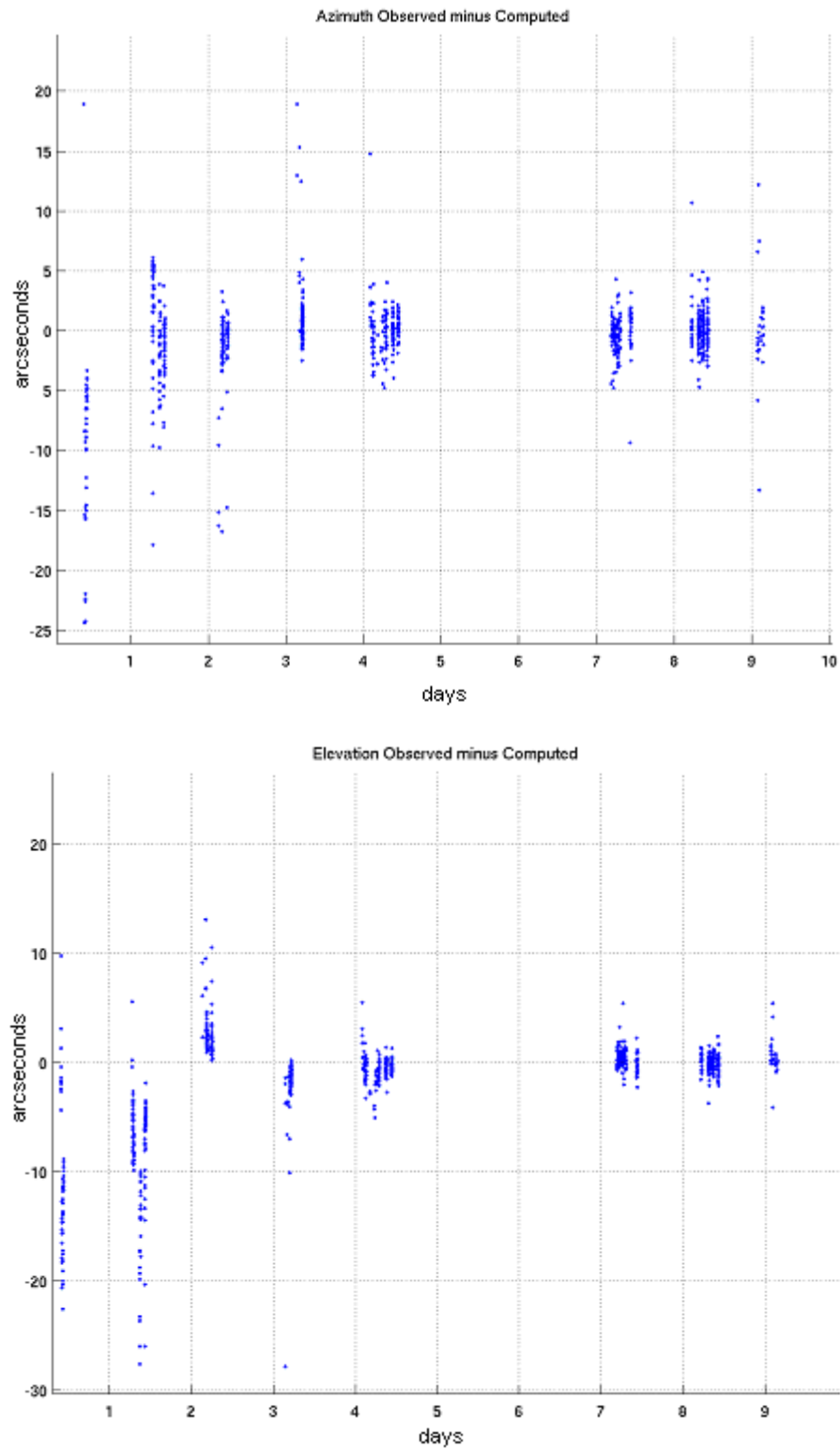
Figure 8-7 – HANDS Azimuth and Elevation Residuals vs Time using SSN and HANDS Data with Spherical Model (ESKF)
