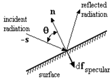
Figure 3-2 – Specular Reflection
