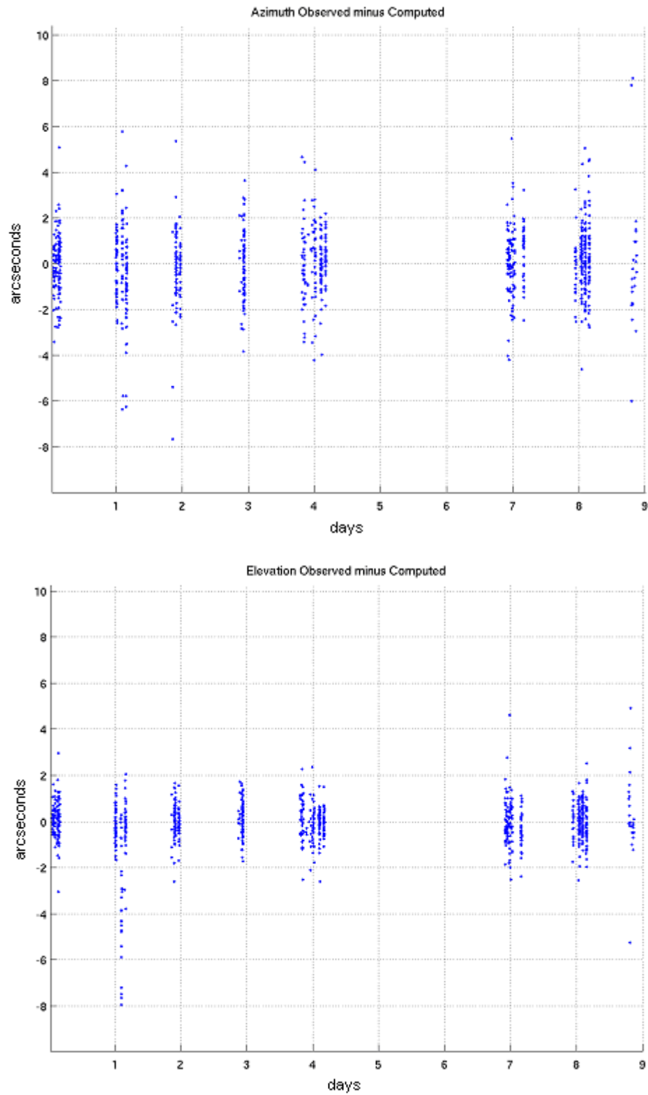
Figure 8-5 – HANDS Azimuth and Elevation Residuals vs Time using Only HANDS Data with Spherical Model (ESKF)
