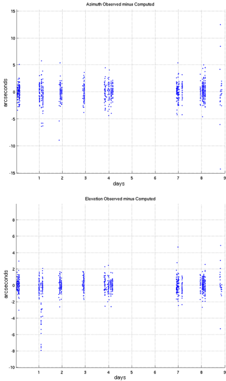
Figure 8-6 – HANDS Azimuth and Elevation Residuals vs Time using Only HANDS Data with Box-wing Model (ESKF)
