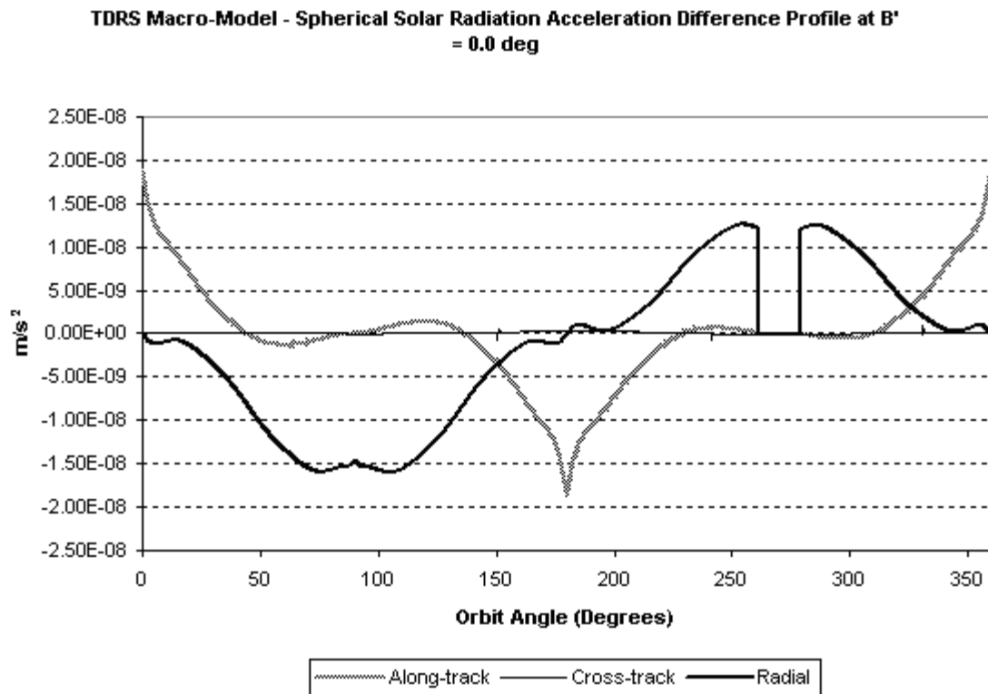
Figure 7-6 – UNIX GTDS TDRS Macro-model - Spherical Acceleration Difference Profile for \beta' = 0^\circ
