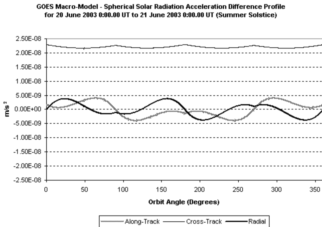
Figure 7-8 – UNIX GTDS GOES Macro-model-Spherical Acceleration Difference Profile at \beta' = 22.5^\circ
