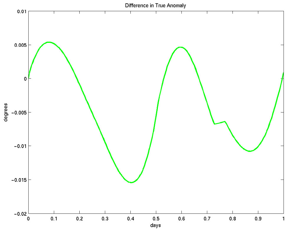
Figure A-6 – Box-wing – Spherical Difference in \omega and v (Autumnal Equinox Case)
