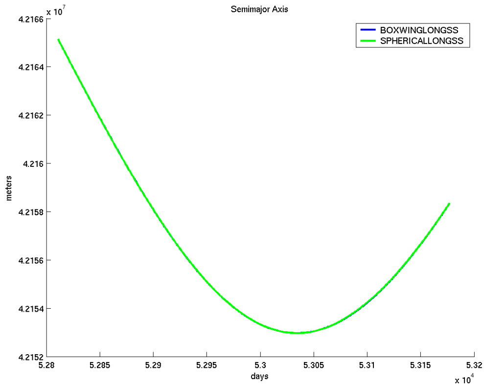
Figure A-10 – One-year Mean Element Plot of a (Summer Solstice)
