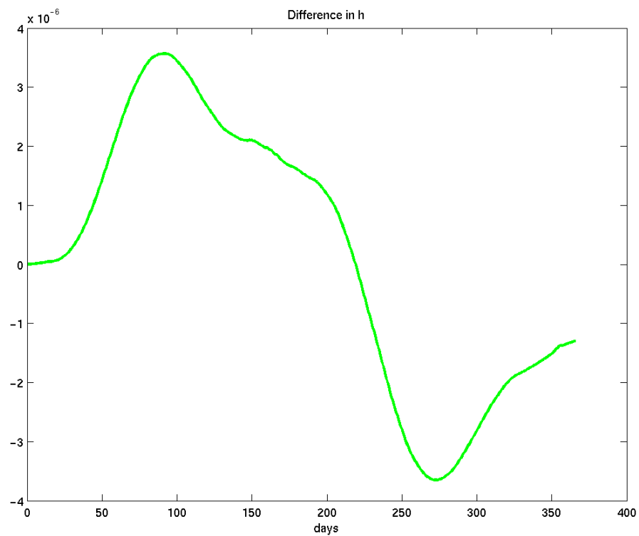
Figure 7-15 – Box-wing – Spherical Difference in h (Sep 03 – Sep 04 Case)
