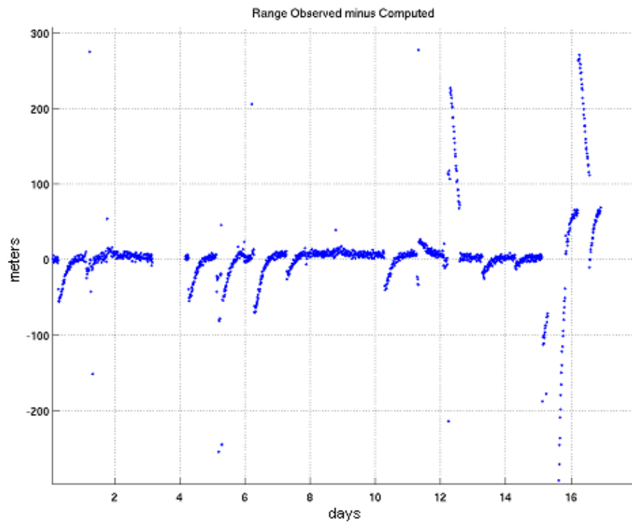
Figure 8-24 – GOES Station 6 Range Residuals vs Time using SSN and NOAA Ranging Data with Spherical Model (ESKF)
