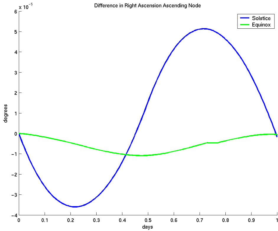
Figure 7-12 – Box-wing – Spherical Difference in i and \Omega
