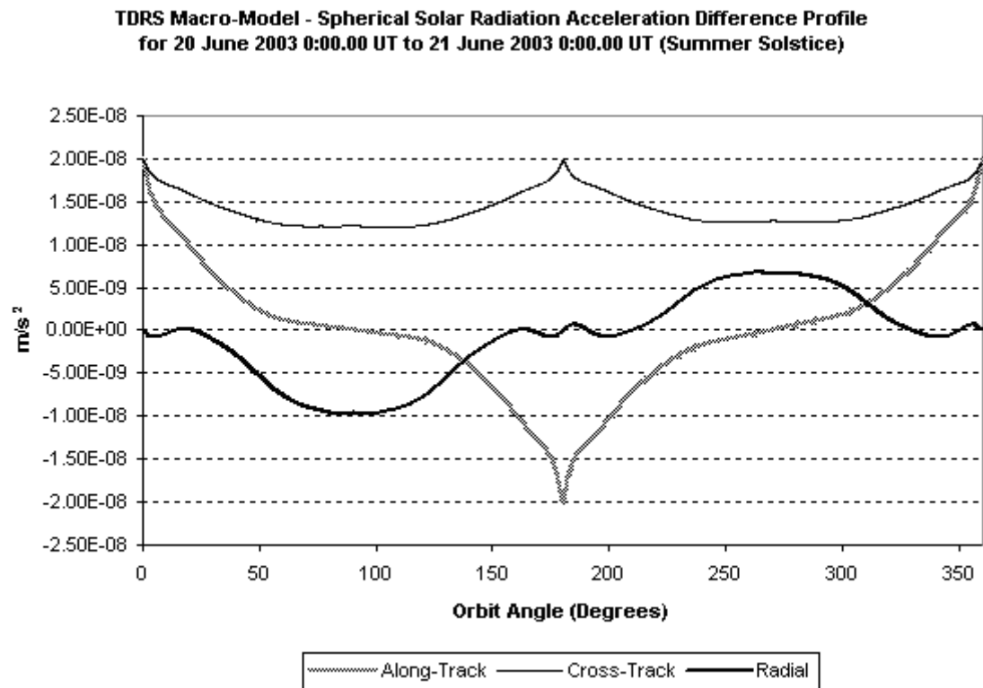
Figure 7-3 – UNIX GTDS TDRS Macro-model - Spherical Acceleration Diff. Profile at \beta' = 22.5
