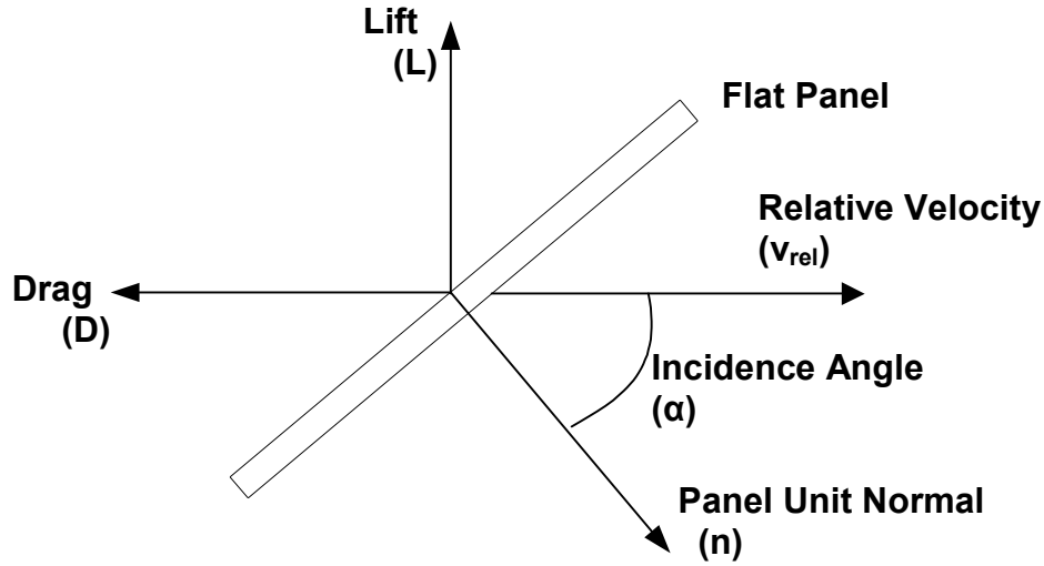
Figure E-1 – Flat Plate Aerodynamic Force Model
