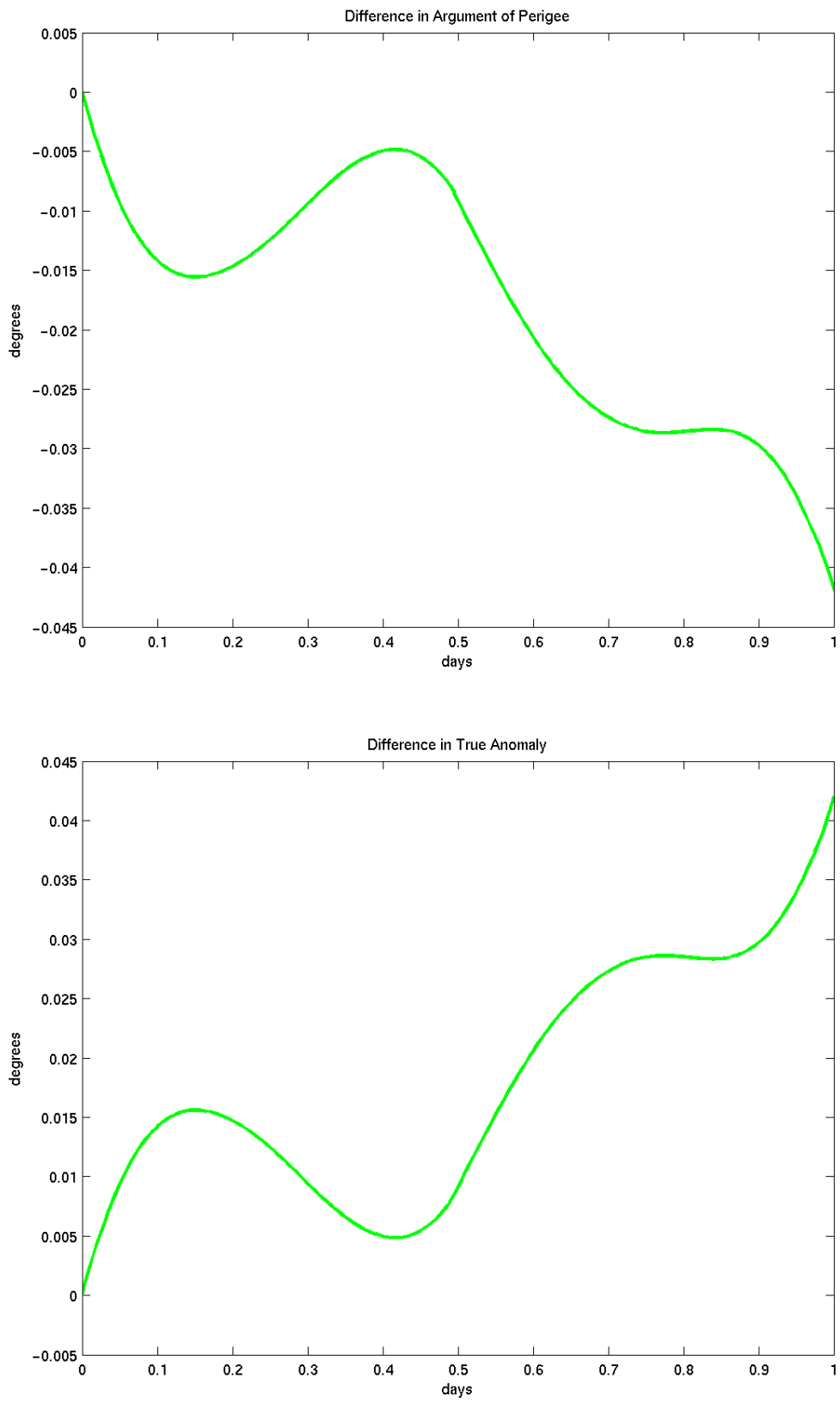
Figure A-3 – Box-wing – Spherical Difference in \omega and v (Summer Solstice Case)
