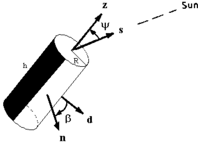
Figure 3-9 – Right Circular Cylinder Illuminated by the Sun
