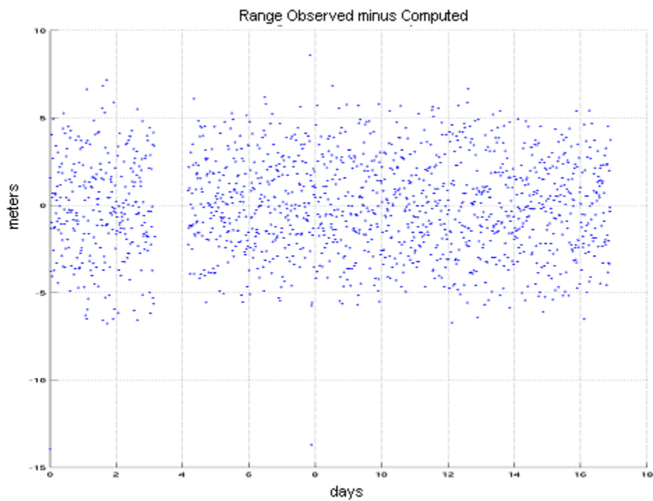
Figure 8-19 – GOES Station 6 Range Residuals vs Time using Only NOAA Ranging Data with Box-wing Model (ESKF)
