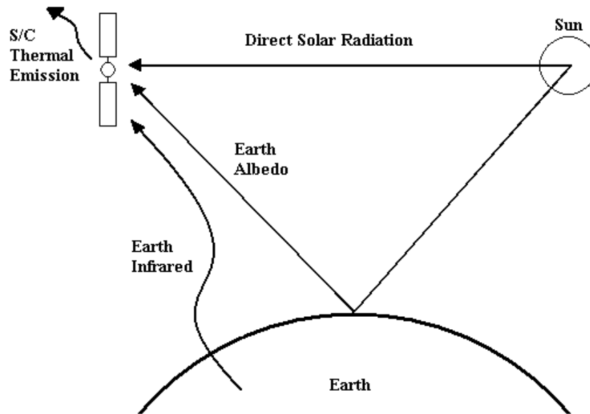
Figure 1-2 – Radiative Forces Acting on a Spacecraft
