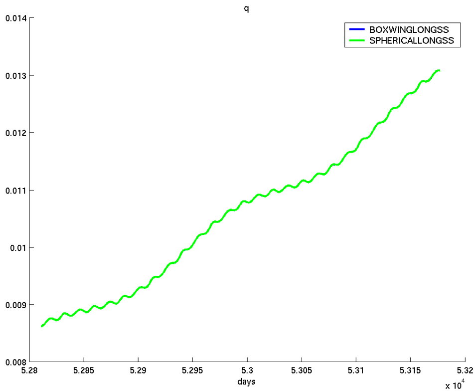
Figure A-12 – One-year Mean Element Plots of p and q (Summer Solstice)
