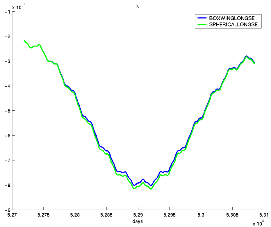
Figure A-8 – One-year Mean Element Plots of h and k (Vernal Equinox)
