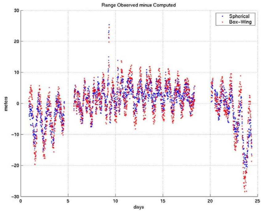
Figure 8-9– GOES Station 6 Range Residuals Using SSN Obs and NOAA Ranging Data – Semi-analytical Satellite Theory Fit (DC)
