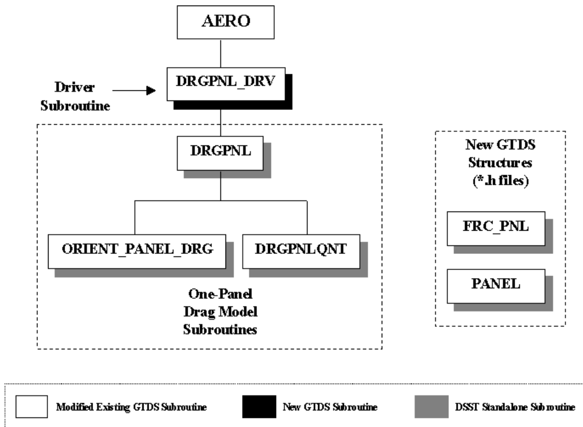
Figure E-2 – Software Design Tree for Incorporation of DSST Standalone One-panel Drag Model Subroutines into GTDS
