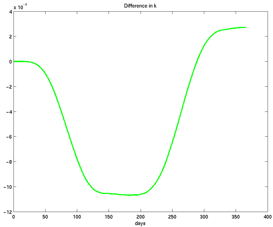
Figure 7-17 – Box-wing – Spherical Difference in k (Sep 03 – Sep 04 Case)
