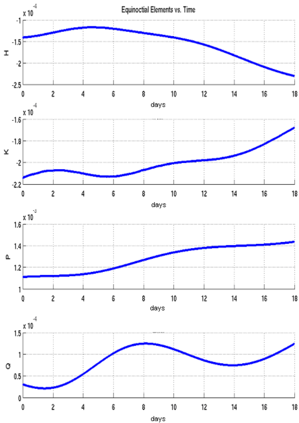
Figure 8-15 – Mean Equinoctial Elements vs Time using Only NOAA Ranging Data with Spherical Model (ESKF)
