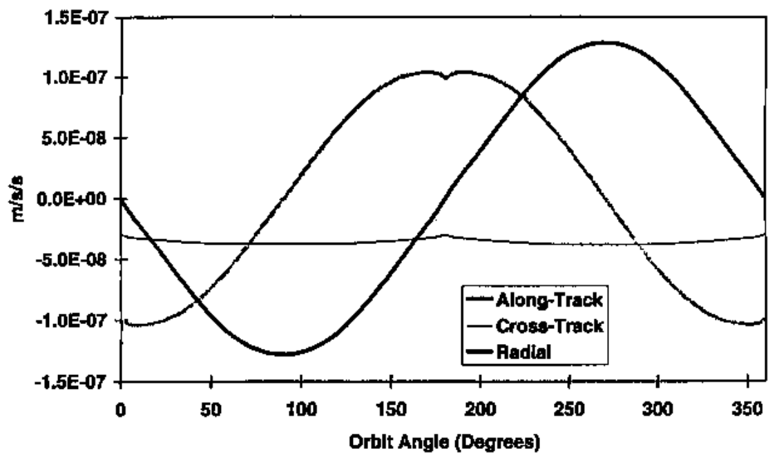
Figure 7-1 – UNIX GTDS TDRS Macro-model Solar Radiation Acceleration Profile at \beta' = 22.5
