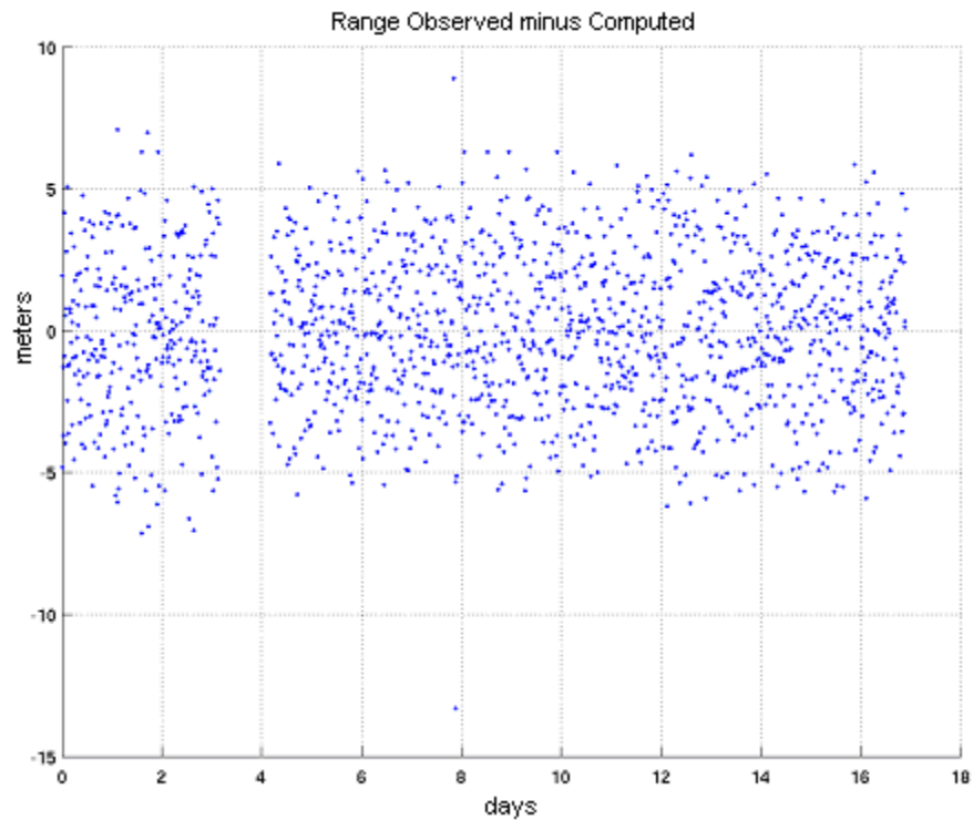
Figure 8-18 – GOES Station 6 Range Residuals vs Time using Only NOAA Ranging Data with Spherical Model (ESKF)
