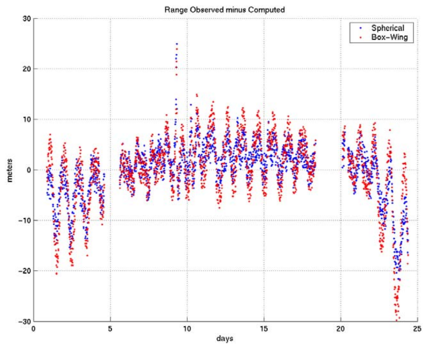
Figure 8-10–GOES Station 6 Range Residuals Using SSN Obs and NOAA Ranging Data – Cowell Theory Fit (DC)
