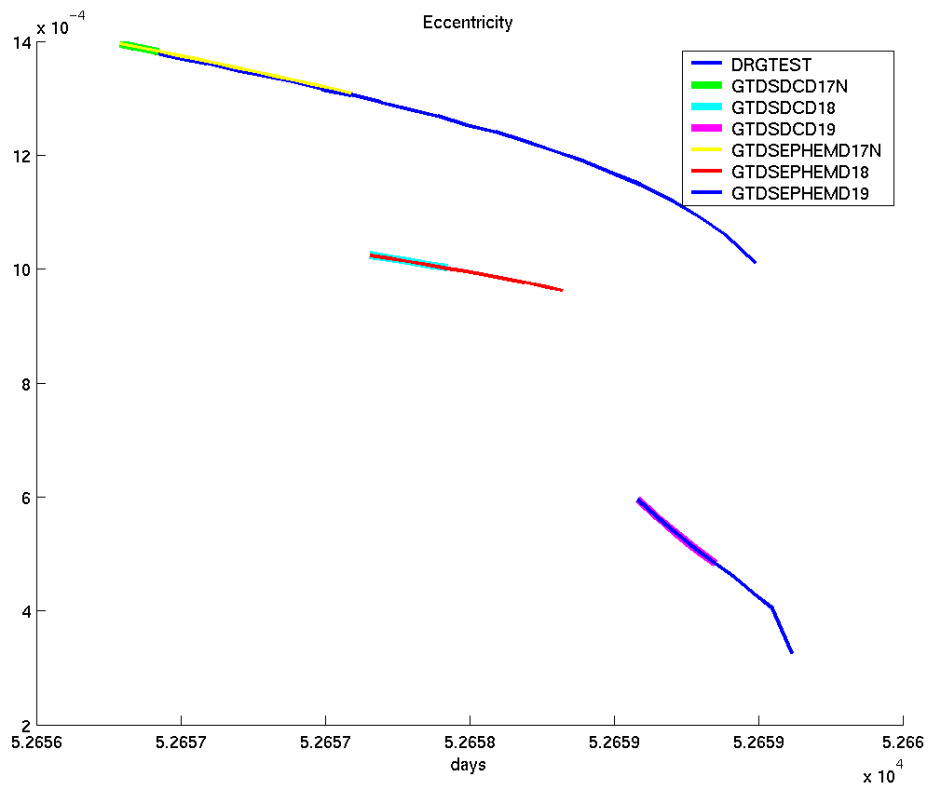
Figure E-4 – Semimajor Axis and Eccentricity Behavior Using the Spherical Model
