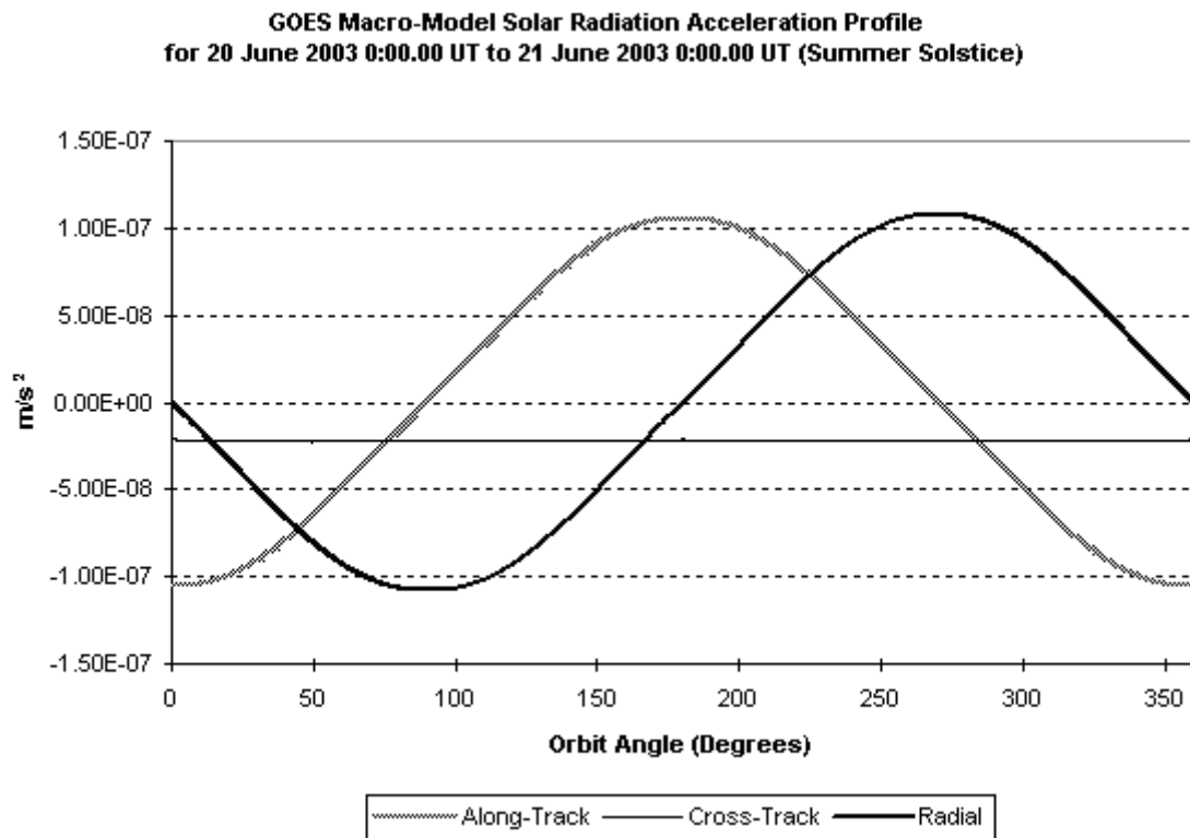
Figure 7-7 – UNIX GTDS GOES Macro-model Solar Radiation Acceleration Profile at \beta' = 22.5^\circ
