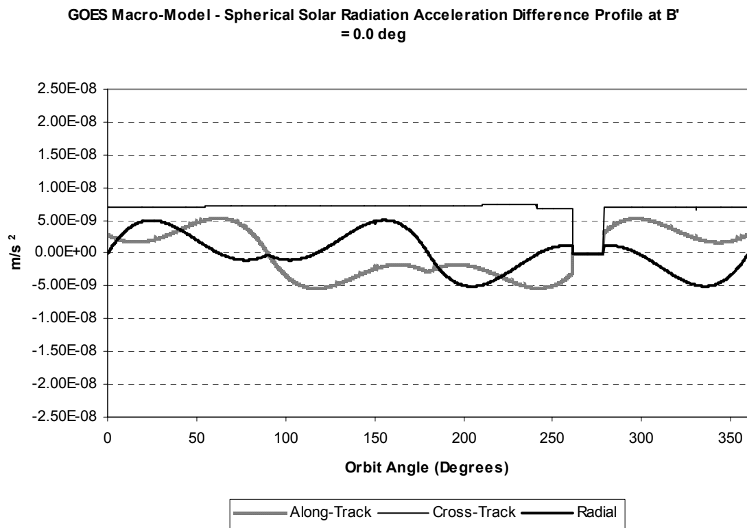
Figure 7-10 – UNIX GTDS GOES Macro-model-Spherical Acceleration Difference Profile for \beta' = 0^\circ
