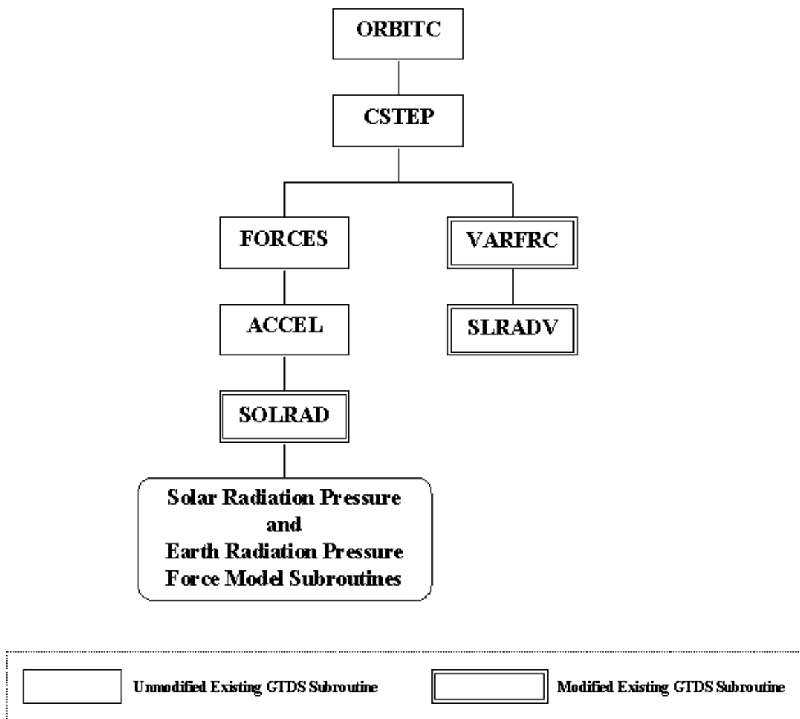
Figure 6-6 – Software Design Tree for GTDS Cowell Theory DC
