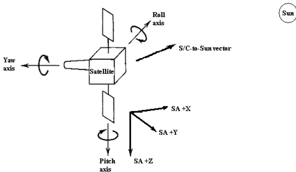
Figure 2-9 – Solar Array (SA) Coordinate Frame
