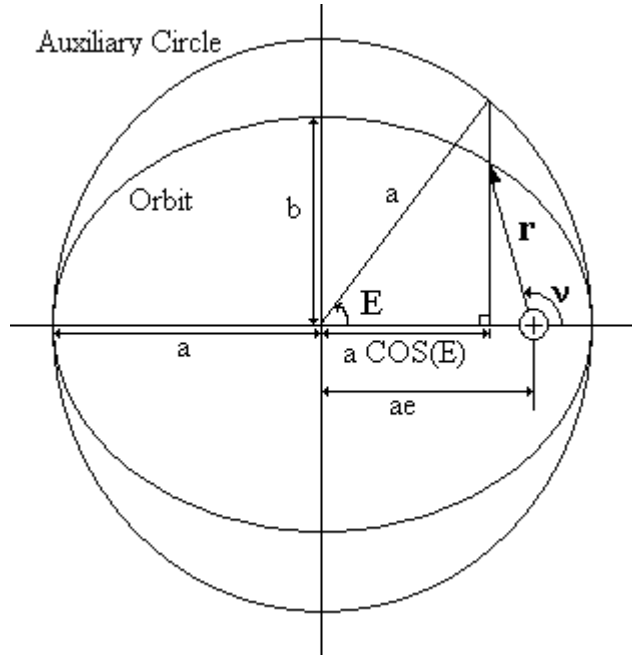
Figure 2-2 – Orbital Anomalies for Elliptic Motion
