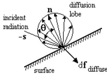
Figure 3-3 – Diffuse Reflection
