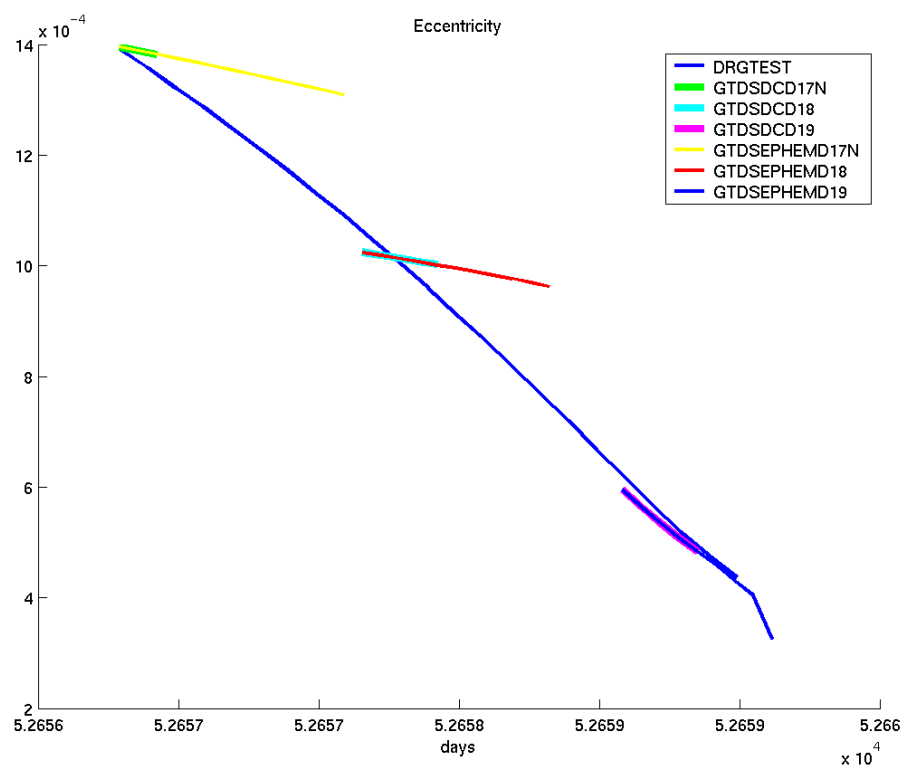
Figure E-5 – Semimajor Axis and Eccentricity Behavior Using the One-panel Model
