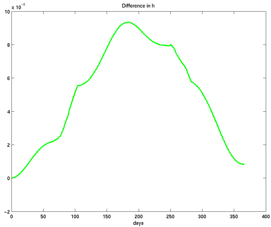
Figure 7-14 – Box-wing – Spherical Difference in h (Jun 03 – Jun 04 Case)
