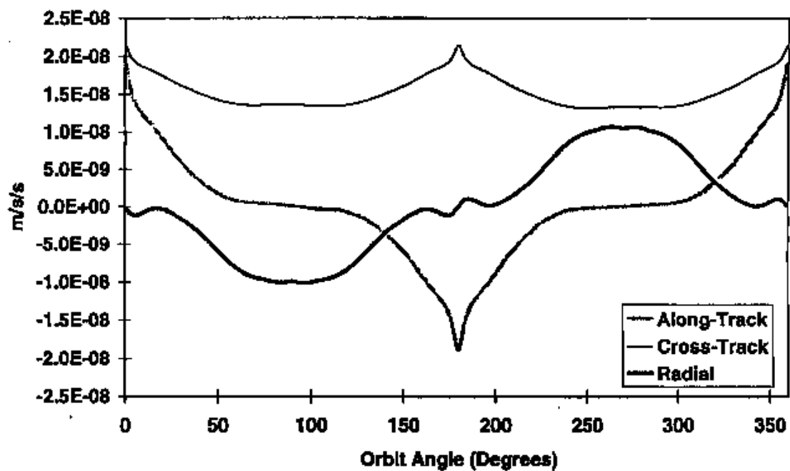
Figure 7-4 – GEODYN TDRS Macro-model - Spherical Acceleration Difference Profile at \beta' = 23.4
