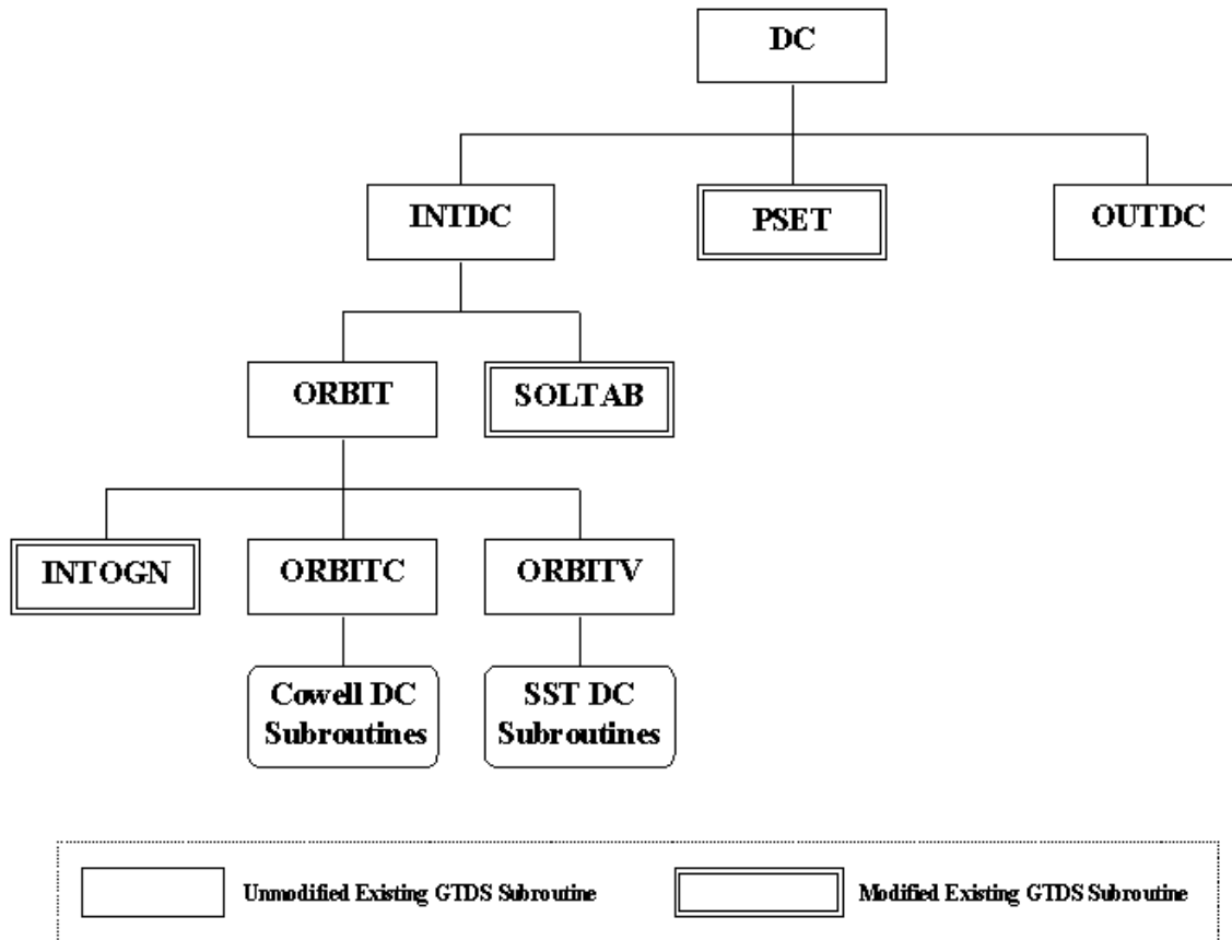
Figure 6-5 – Software Design Tree for GTDS Differential Correction Program
