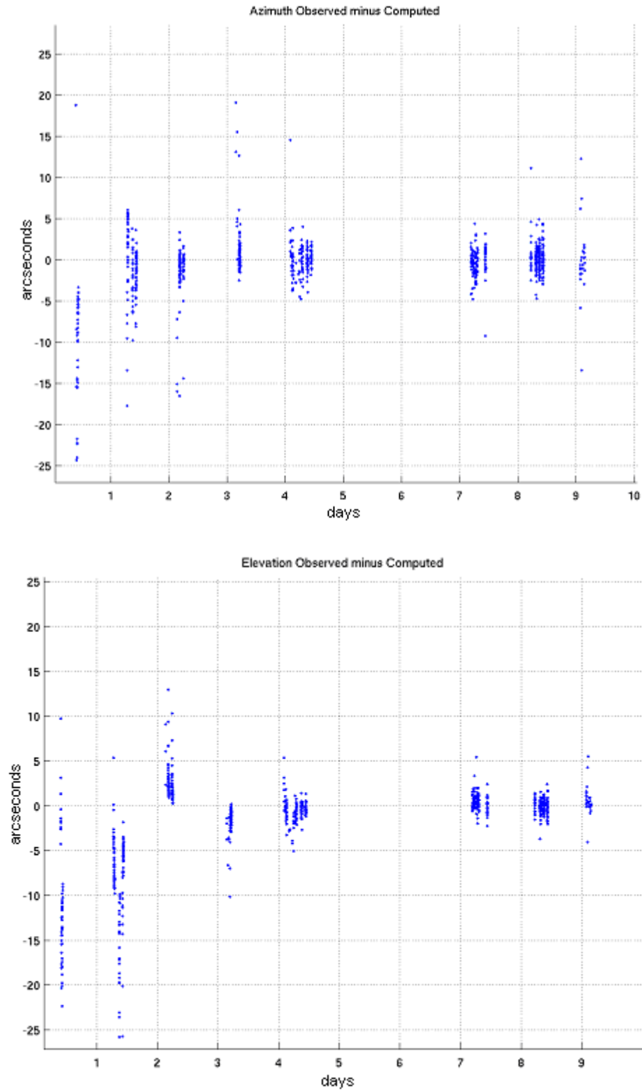
Figure 8-8 – HANDS Azimuth and Elevation Residuals vs Time using SSN and HANDS Data with Box-wing Model (ESKF)
