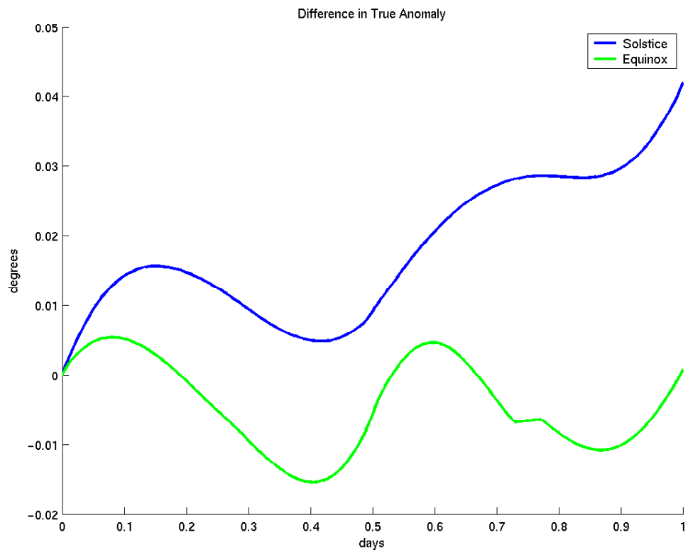
Figure 7-13 – Box-wing – Spherical Difference in \omega and \nu
