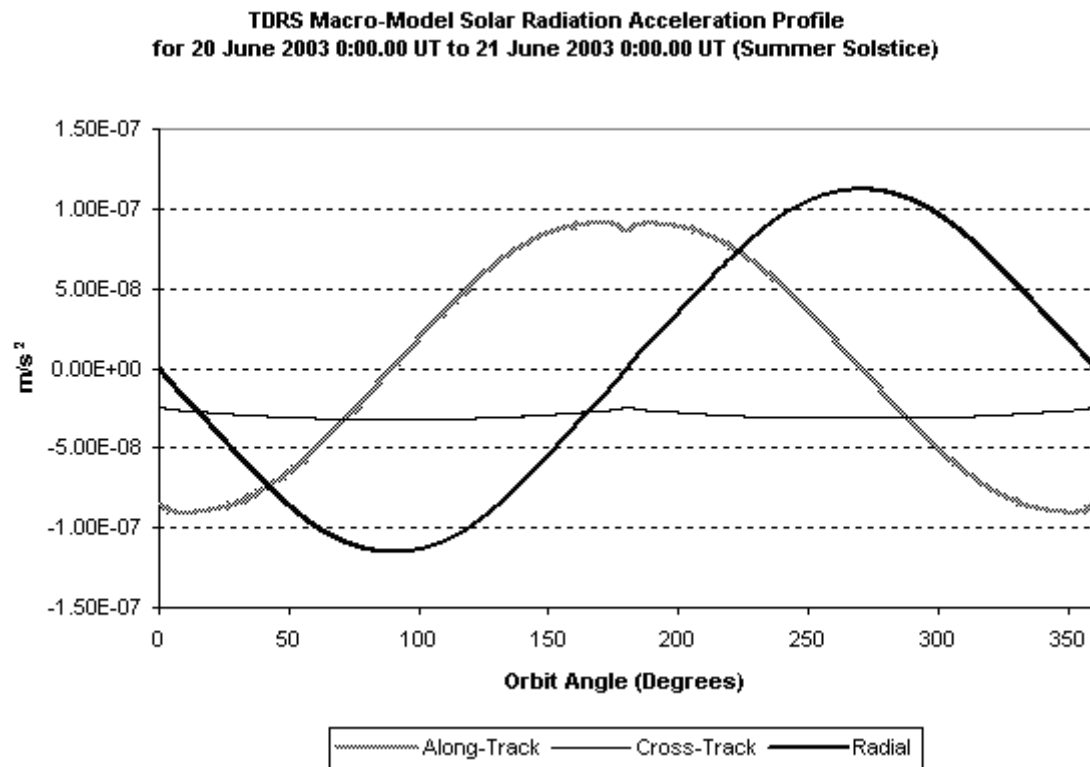
Figure 7-1 – UNIX GTDS TDRS Macro-model Solar Radiation Acceleration Profile at \beta' = 22.5
