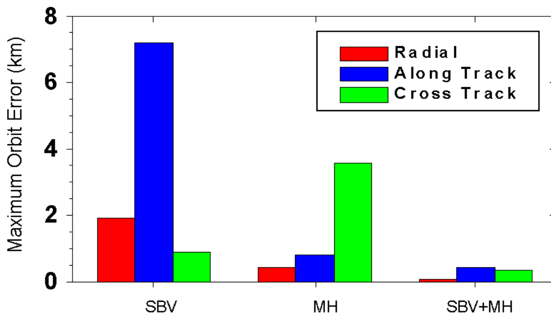
Figure 1-5 – GMWS Orbit Accuracy for TDRS-4 Using Various Data Sources
