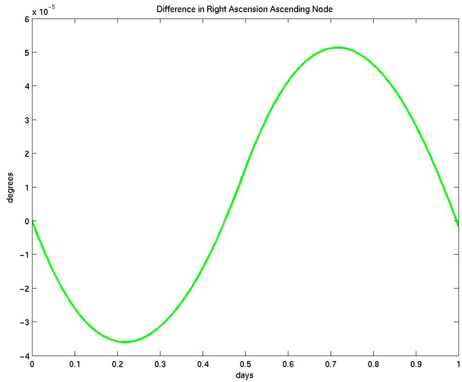
Figure A-2 – Box-wing – Spherical Difference in i and \Omega (Summer Solstice Case)
