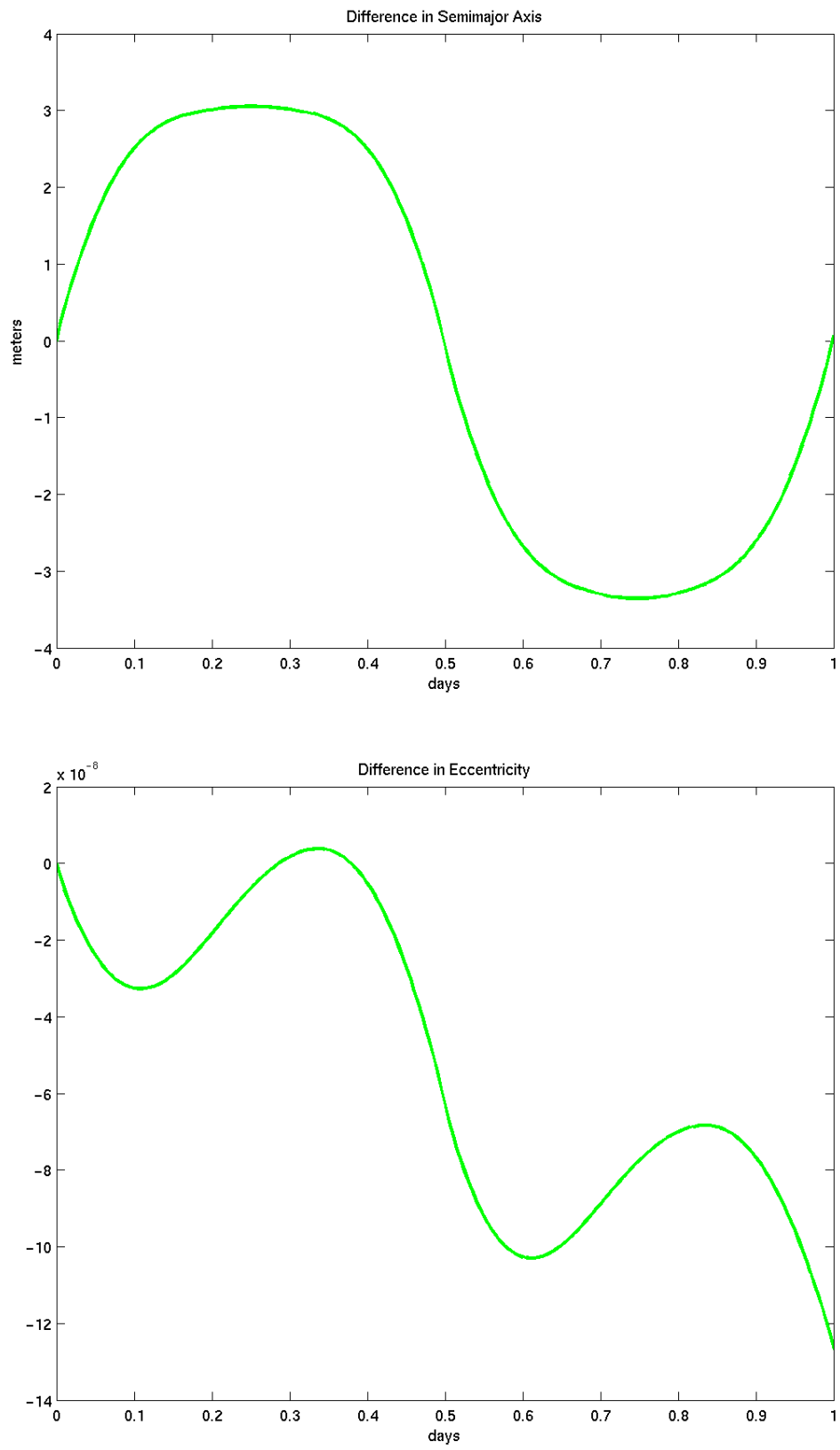
Figure A-1 – Box-wing – Spherical Difference in a and e (Summer Solstice Case)
