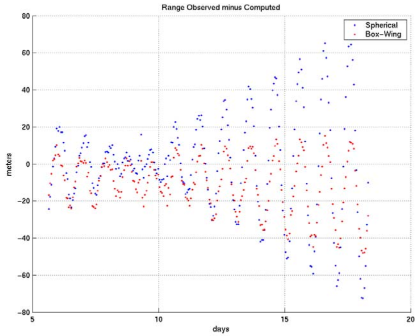
Figure 8-11– GOES Station 6 Range Residuals Using SSN Obs and Thinned/Deweighted NOAA Ranging Data, Spherical Range Bias (DC)
