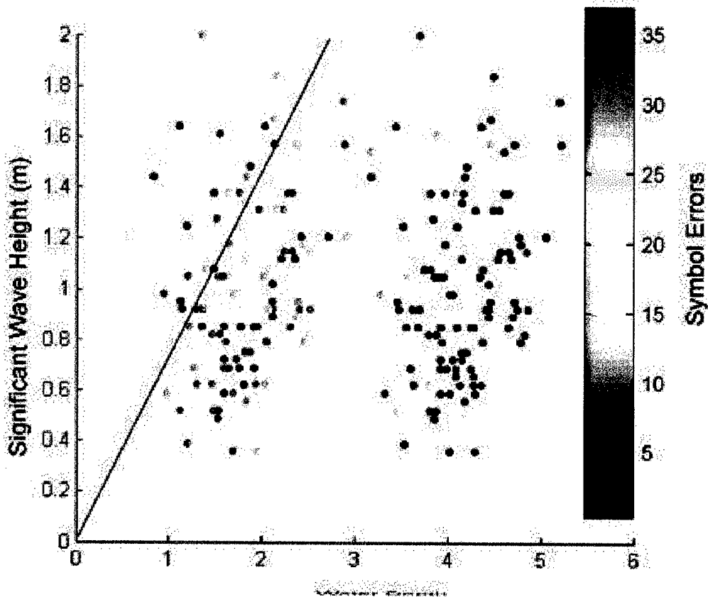
Figure 1. The figure, taken with permission from Commander et. al. , shows symbol errors as a function of water depth and significant wave height. The solid line in the figure shows the significant wave height at which wave breaking begins for a given water depth, as established by the McCowan breaking criterion. The data show that communications errors increase in the region predicted by the McCowan breaking criterion.
