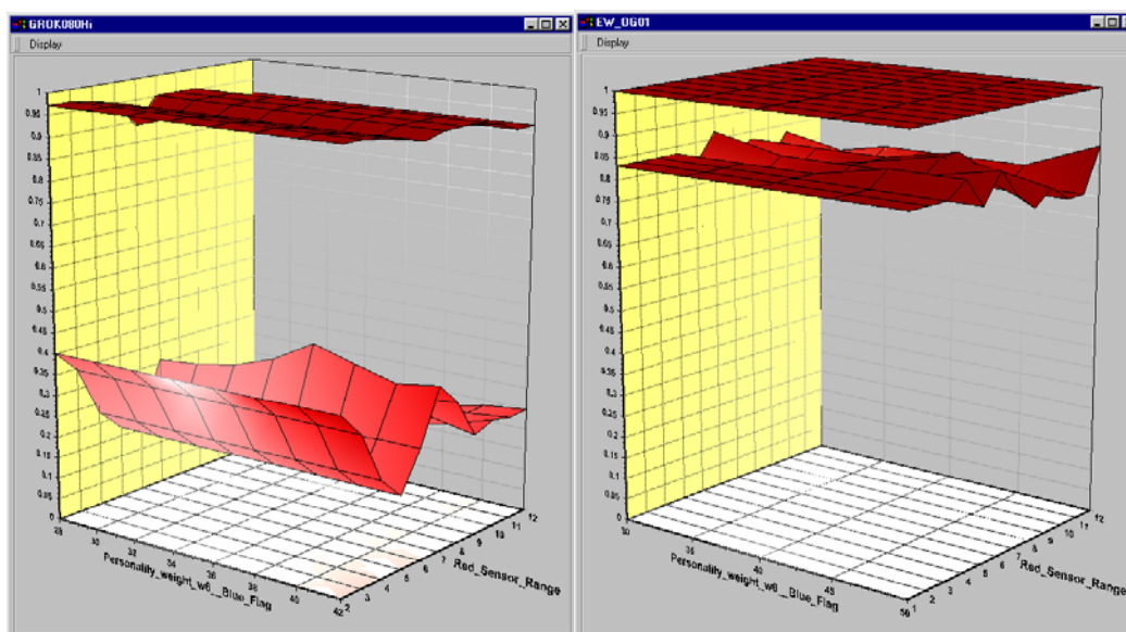
Figure 4: ISAAC Scenario 1 and 2 – Blue Sensor Range = 6.
