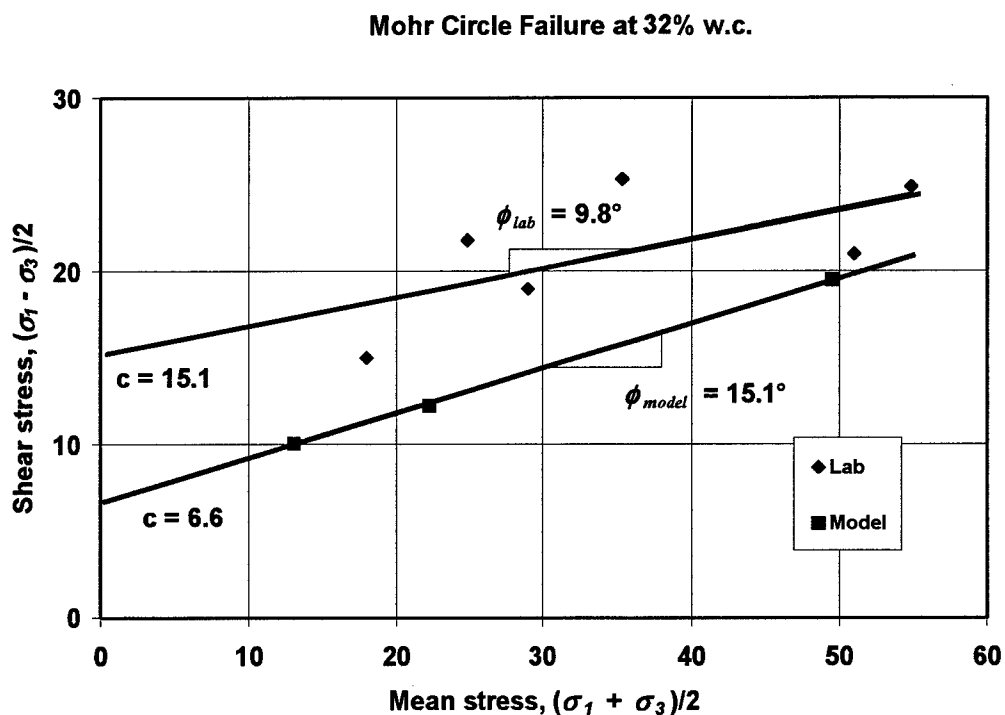
Figure 8-36: Comparison of Laboratory Mohr circle failure envelope with PS-MMM at 32% water content
