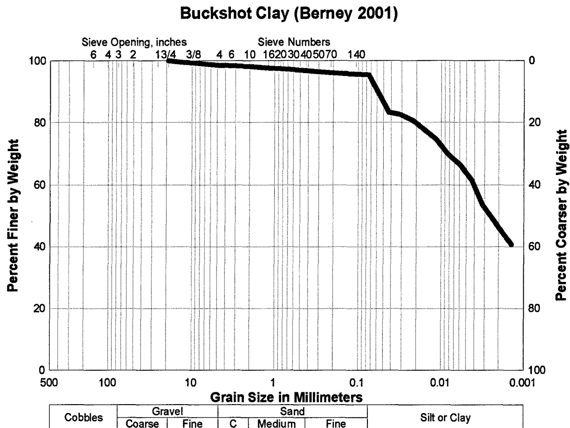
Figure 6-1: Grain Size Distribution for Buckshot Clay
