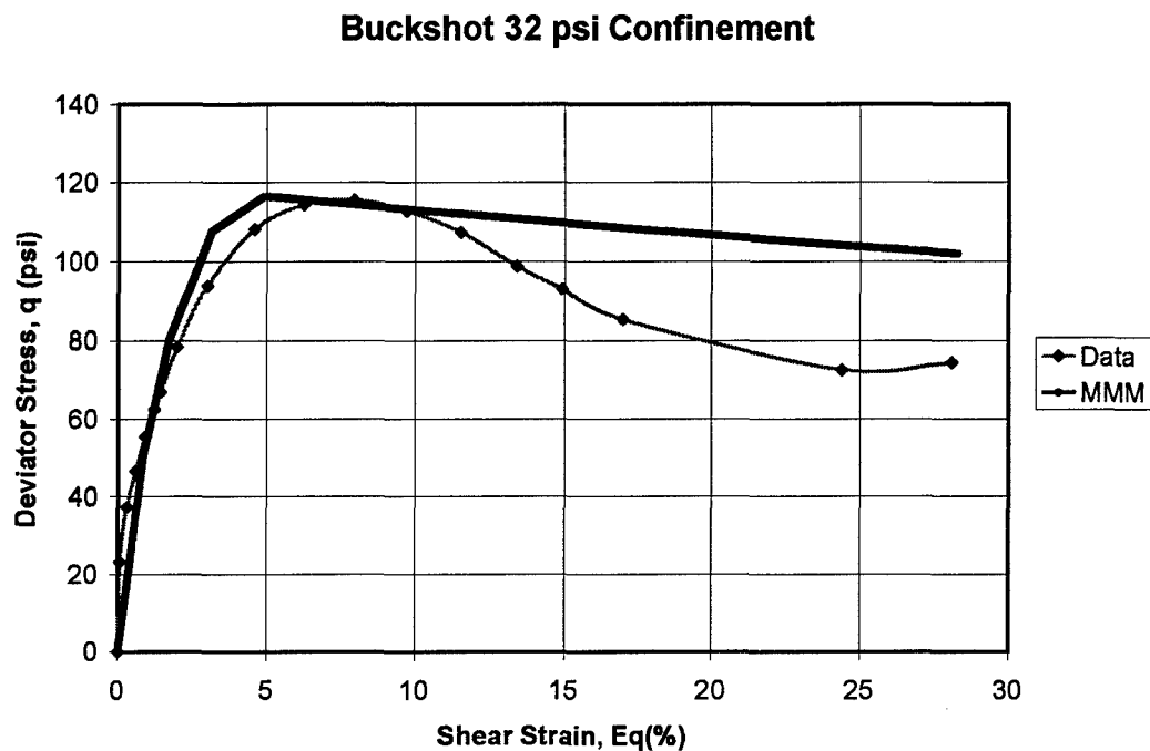
Figure 8-21: MMM simulation of shear stress-shear strain response of 32 psi confined CD triaxial specimen
