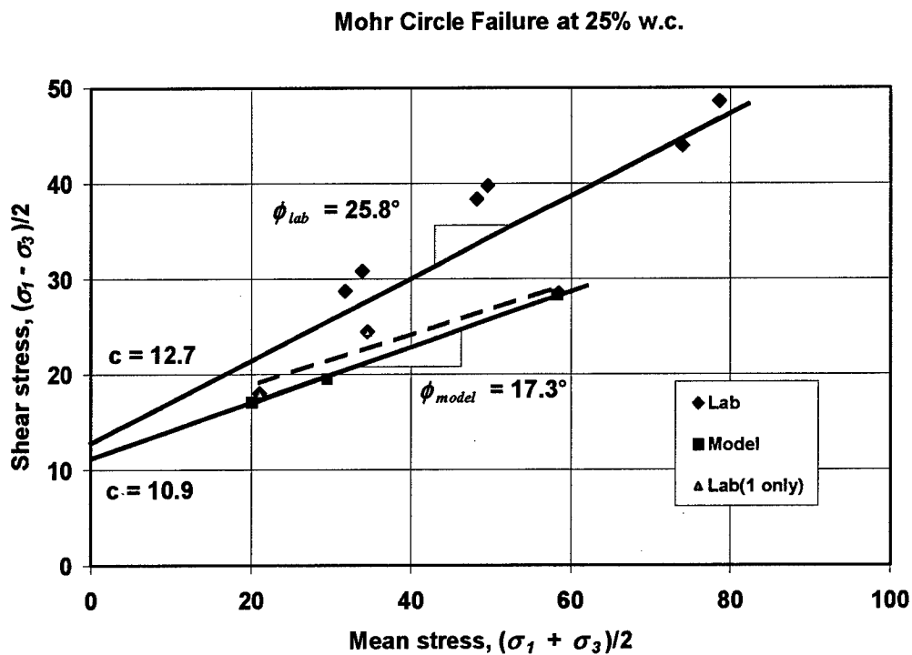
Figure 8-35: Comparison of Laboratory Mohr circle failure envelope with PS-MMM at 25% water content
