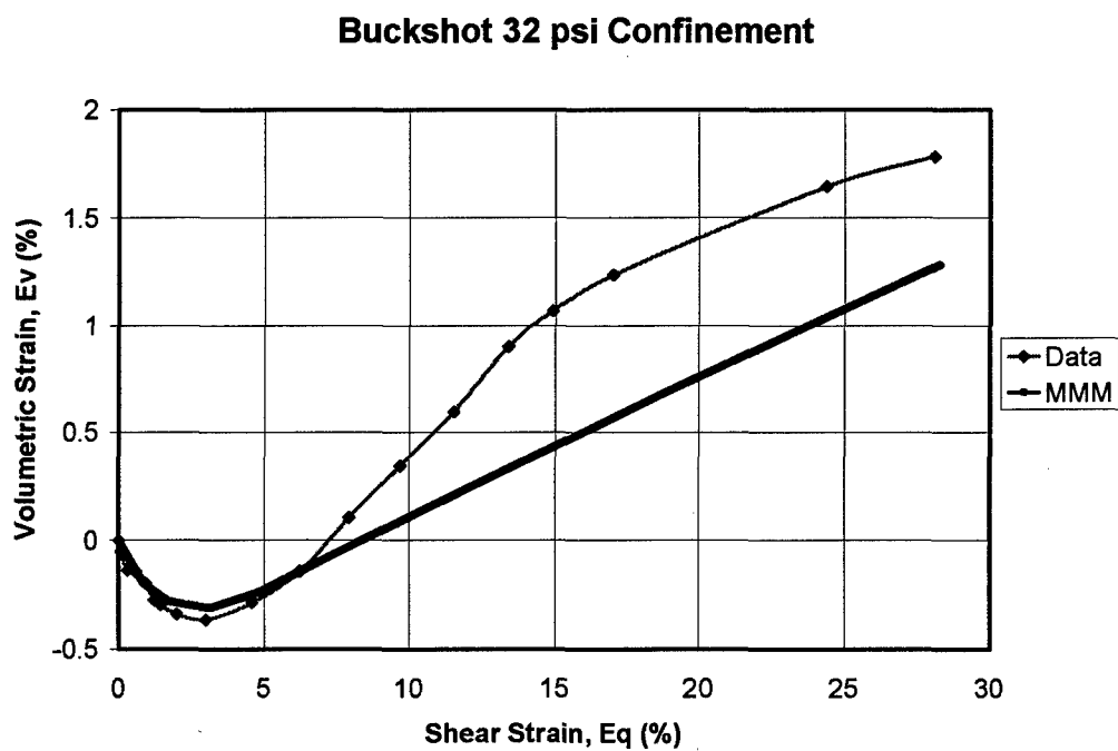
Figure 8-22: MMM simulation of volumetric strain response of 32 psi confined CD triaxial specimen (from Peters)
