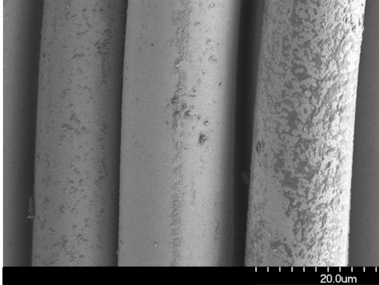
Figure 2. SEM image of E-glass fiber surface treated with hybrid sizing after acetone rinse.
