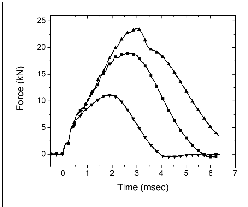
Figure 14. Representative force-vs.-time curves for flat S-2 Glass composite panel treated with epoxy compatible sizing during impact testing. (▼) E_{impact} = 37 J, (■) E_{impact} = 80 J, (▲) E_{impact} = 124 J, V_{impact} = 4.5 m/s.
