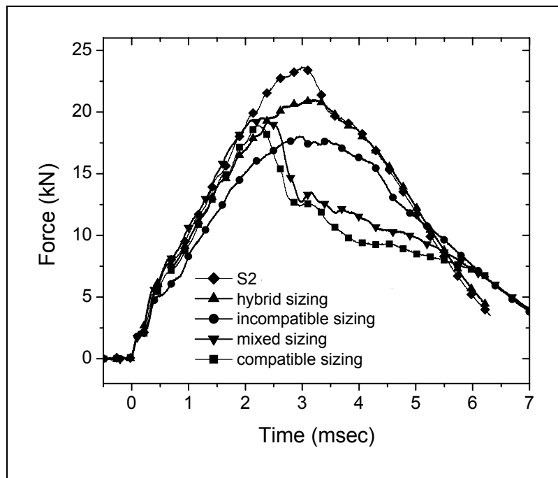
Figure 15. Comparison of composite panel impact response for E-glass fibers treated with hybrid, compatible, mixed, and incompatible fiber sizings. S-2 Glass is also shown. E_{impact} = 124 J, V_{impact} = 4.5 m/s.
