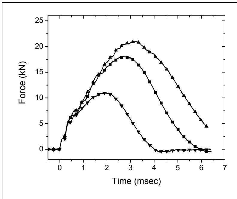
Figure 13. Representative force-vs.-time curves for flat E-glass composite panel treated with hybrid sizing during impact testing. ( \blacktriangledown ) E_{impact} = 37 J, ( \blacksquare ) E_{impact} = 80 J, ( \blacktriangle ) E_{impact} = 124 J, V_{impact} = 4.5 m/s.
