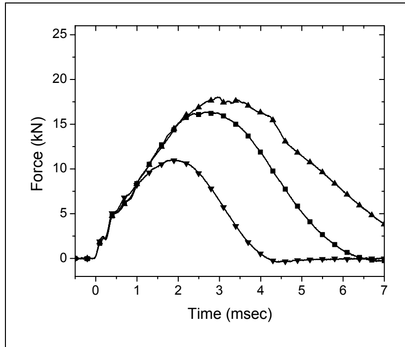
Figure 11. Representative force-vs.-time curves for flat E-glass composite panel treated with incompatible sizing during impact testing. ( \blacktriangledown ) E_{impact} = 37 J, ( \blacksquare ) E_{impact} = 80 J, ( \blacktriangle ) E_{impact} = 124 J, V_{impact} = 4.5 m/s.
