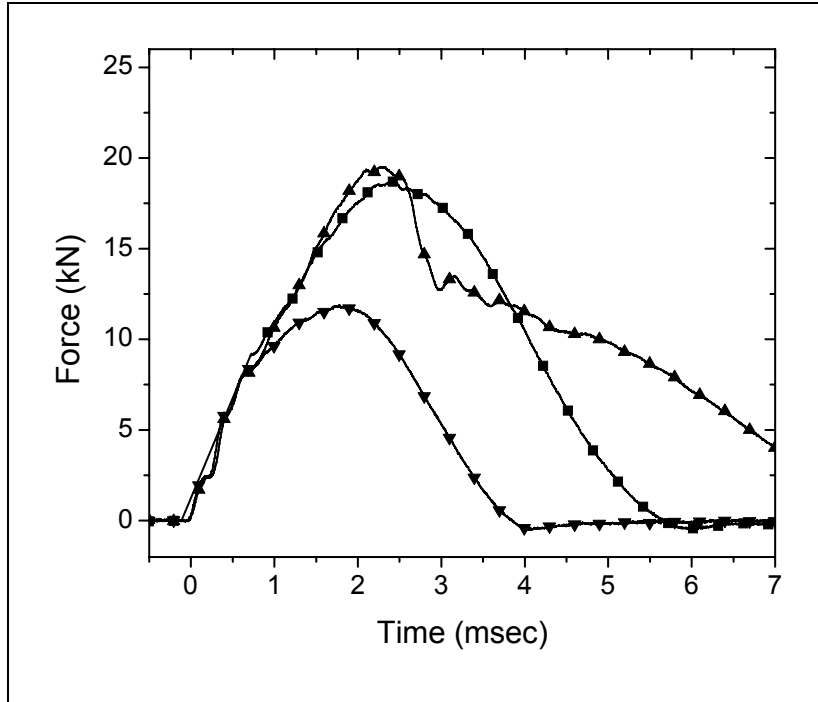
Figure 12. Representative force-vs.-time curves for flat E-glass composite panel treated with mixed sizing during impact testing. ( \blacktriangledown ) E_{impact} = 37 J, ( \blacksquare ) E_{impact} = 80 J, ( \blacktriangle ) E_{impact} = 124 J, V_{impact} = 4.5 m/s.
