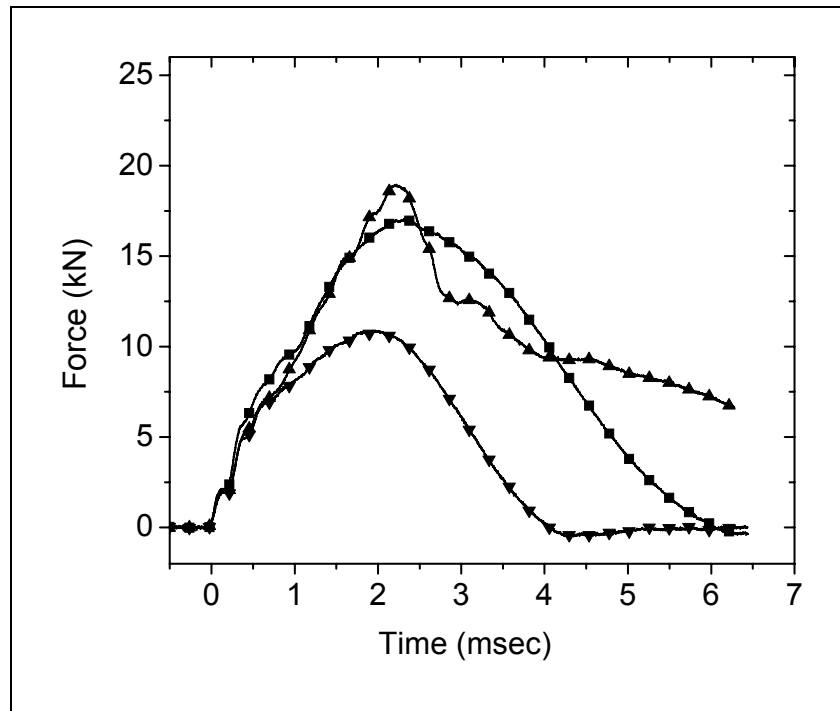
Figure 10. Representative force-vs.-time curves for flat E-glass composite panel treated with compatible sizing during impact testing. ( \blacktriangledown ) E_{impact} = 37 J, ( \blacksquare ) E_{impact} = 80 J, ( \blacktriangle ) E_{impact} = 124 J, V_{impact} = 4.5 m/s.
