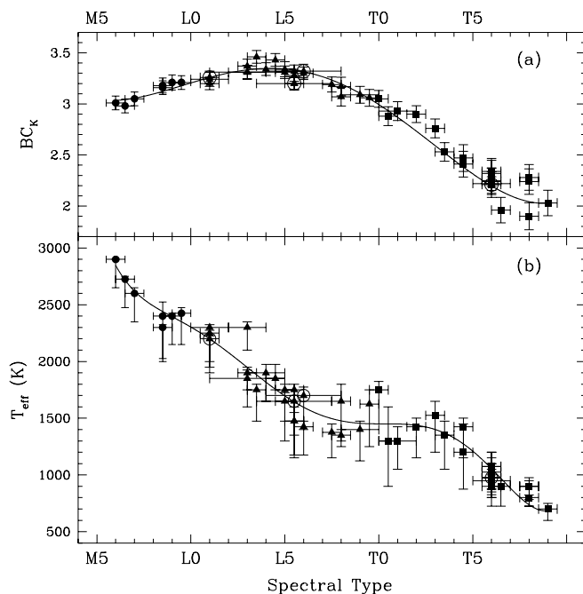
FIG. 6.—Diagrams of (a) BC_K and (b) T_{\text{eff}} vs. spectral type for ultracool dwarfs listed in Table 6. All symbols are described in Fig. 1. The plotted values of T_{\text{eff}} are those listed in col. (7) of Table 6 for a mean age of 3 Gyr, unless otherwise noted. The error bars for these values reflect the full ranges of T_{\text{eff}} listed in col. (6) of Table 6. The curves are (a) fourth-order and (b) sixth-order polynomial fits to the weighted data except those representing known close-binary systems (encircled points). The datum for the T6 dwarf 2MASS J0937+2931 ( BC_K = 1.51 ) is not shown in (a), but it is included in the polynomial fit. The fit in (b) is fixed at type T9 to avoid an unrealistic upturn in T_{\text{eff}} between types T8 and T9.
