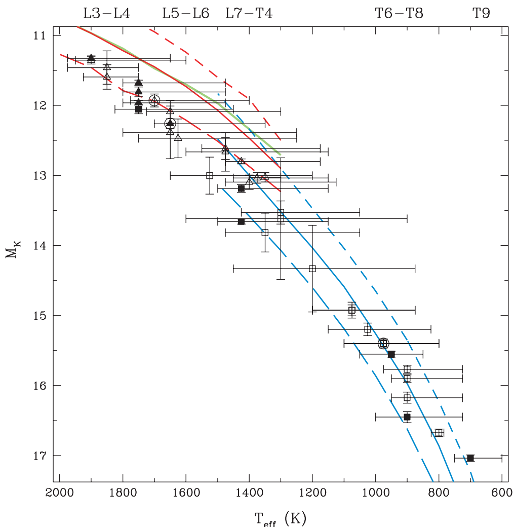
FIG. 8.—Diagram of M_K vs. T_{\text{eff}} for L3–T9 dwarfs listed in Table 6. The plotted values of T_{\text{eff}} are those listed in col. (7) of Table 6 for a mean age of \sim 3 Gyr, unless otherwise noted. The error bars for these values reflect the full ranges of T_{\text{eff}} listed in col. (6) of Table 6. L dwarfs are represented by triangles and T dwarfs are represented by squares. Filled symbols denote those dwarfs for which we have M' photometric data (Fig. 10). The measured values of M_K for close binaries (encircled points) have been increased by 0.75 mag to represent one component of the presumed uneclipsed, equal-luminosity systems. The curves are the predicted relationships from the models of Marley et al. (2002) for brown dwarfs with f_{\text{sed}} = 3 (green), f_{\text{sed}} = 5 (red), and cloud-free atmospheres (blue), and surface gravities of \log g = 4.5 (short-dash), 5.0 (solid), and 5.5 (long-dash).
