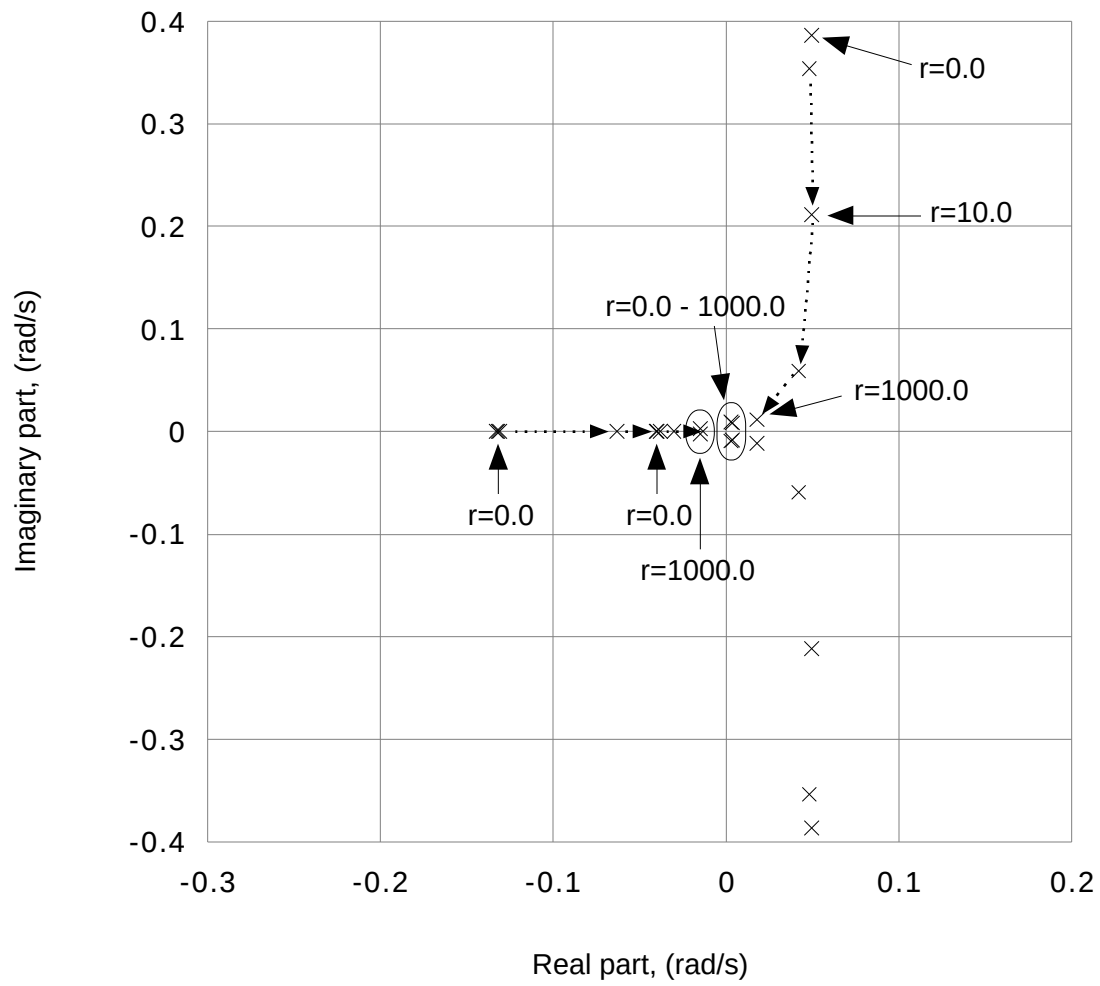
Figure 4.6: Root-locus of controller eigenvalues of LTI closed-loop system, V=80 kts.
