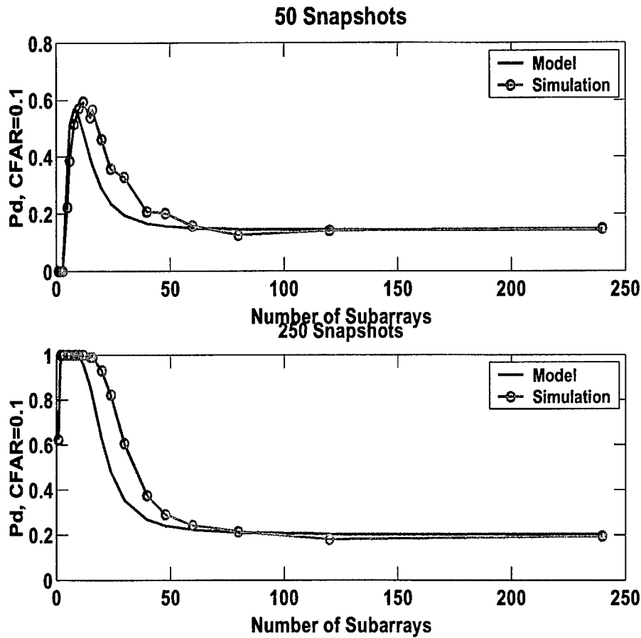
Figure 4-18: Detection performance vs. number of subarrays. The target is coherent and the interferer has a coherence length of 2500 elements ( >10 array lengths).
