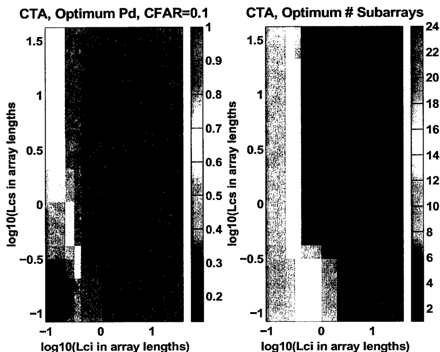
Figure 5-30: Pd vs coherence (a) and optimal subarray configuration adaptive degrees of freedom vs coherence for the CTA algorithm.
