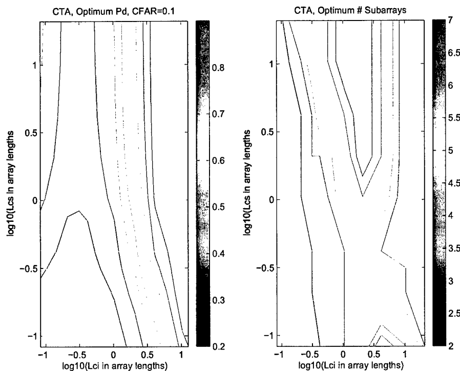
Figure 5-17: Detection performance and optimum subarray configuration of the CTA algorithm as a function of interferer and target coherence for a loud in-beam interferer.
