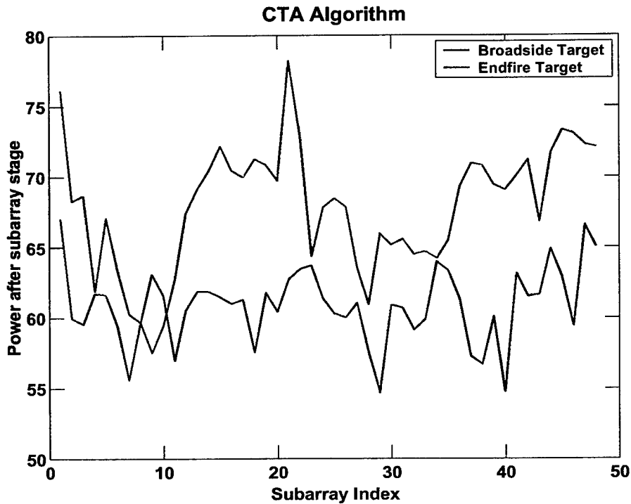
Figure 5-34: Power on each subarray after the first stage of processing for the CTA algorithm, broadside target and endfire target.
