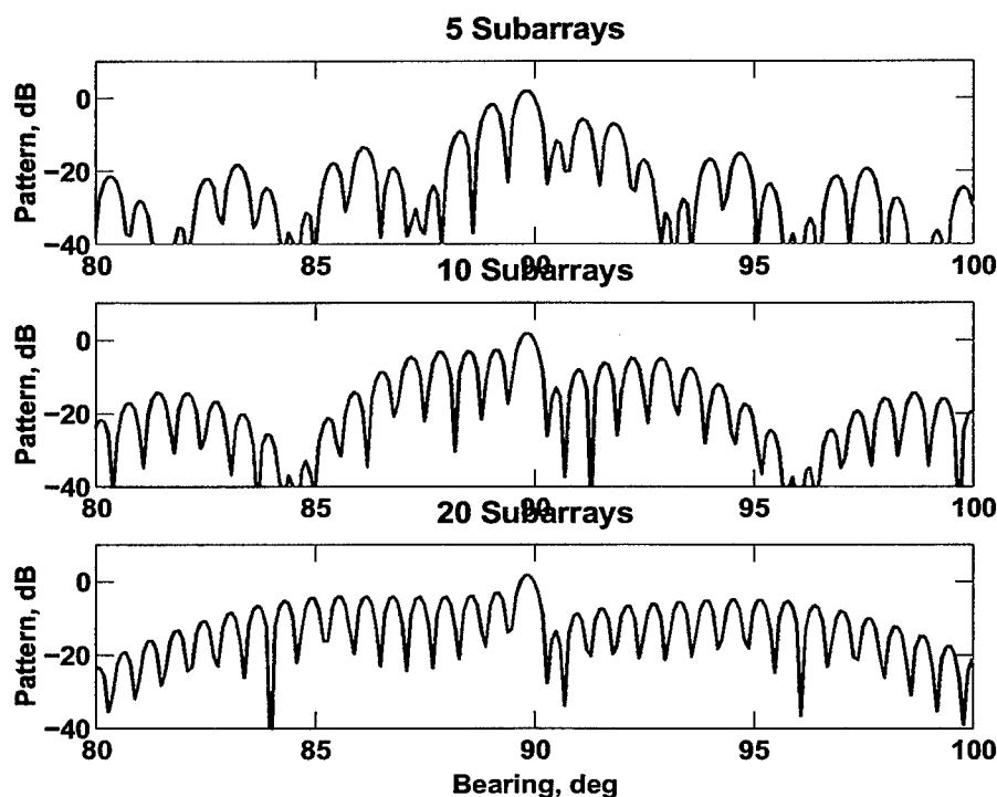
Figure 5-19: Adaptive beam patterns for 5, 10, and 20 subarray configurations. L_{cs}=L_{ci}=250 elements. High sidelobes in the vicinity of the look direction impact performance.
