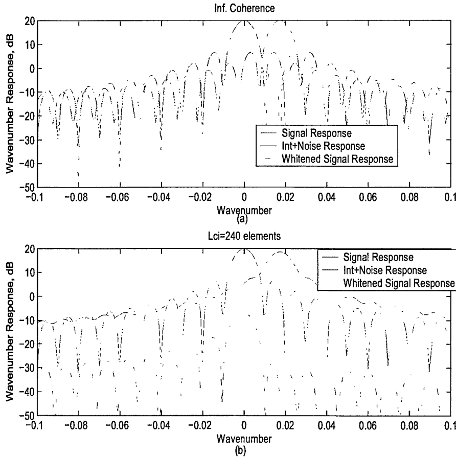
Figure 5-2: Array response to signal, interference, and whitenred response for (a) perfect interferer coherence, and (b) L_{ci}=240 elements.
