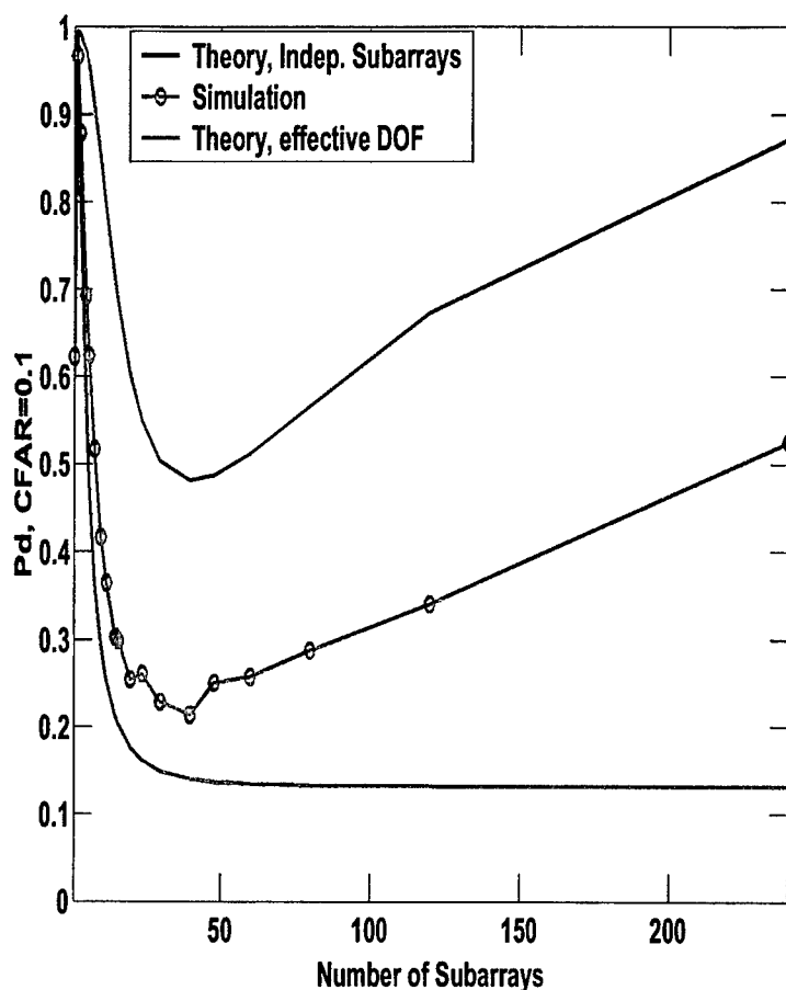
Figure 4-9: Comparison of simulated and analytical curves for AI algorithm, interference-dominated example showing improved model. L_{cs}=\text{inf} , L_{ci}=2500 elements.
