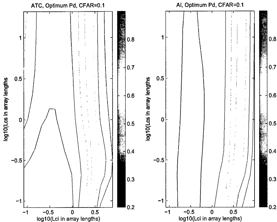
Figure 5-20: Detection performance of the ATC and AI algorithms as a function of interferer and target coherence for a loud in-beam interferer.
