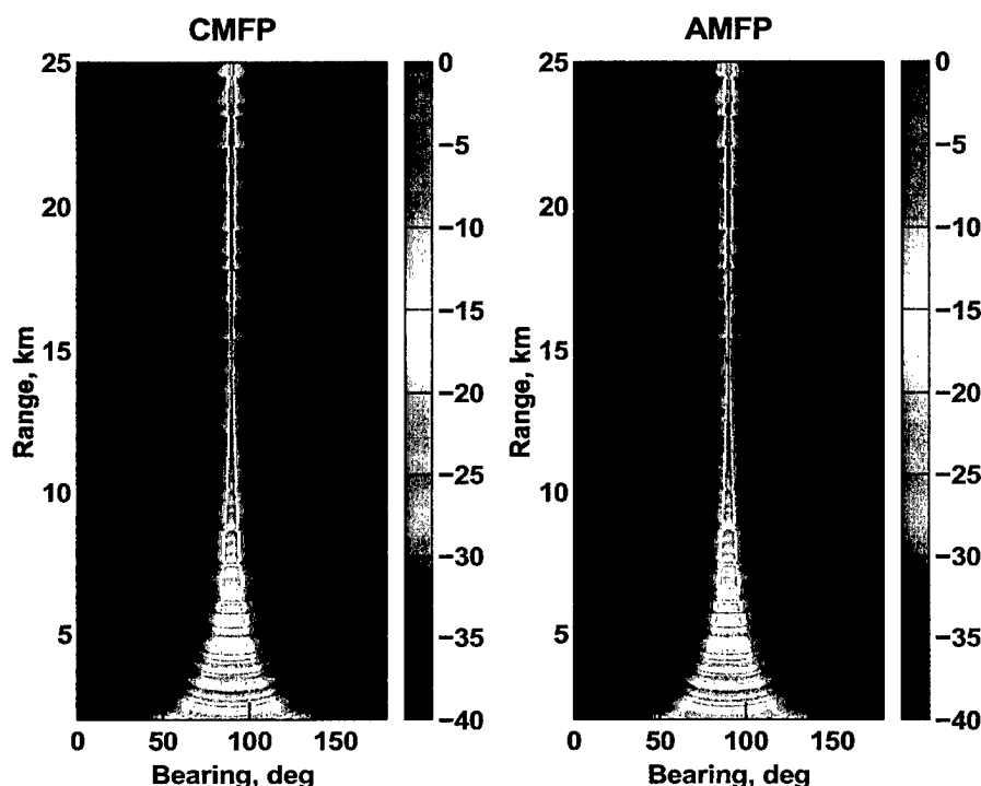
Figure 5-28: CMFP and AMFP beam pattern at interference depth for full array steered to 100m, 15km, and 90-deg.
