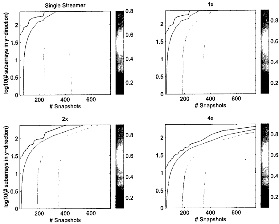
Figure 5-37: Pd vs snapshots for different subarray configurations, CTA algorithm.
