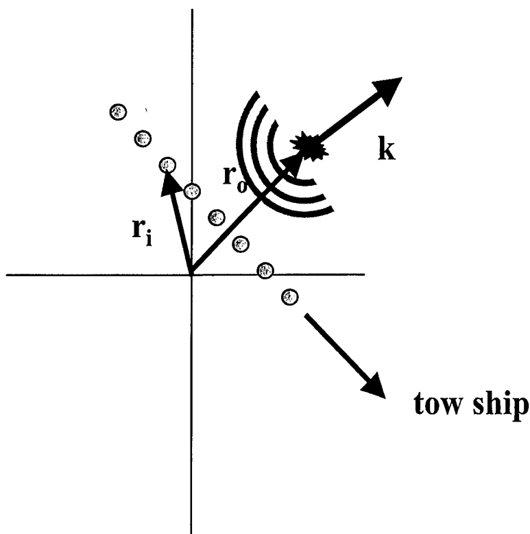
Figure 2-5: Wavefront Curvature propagation model.
