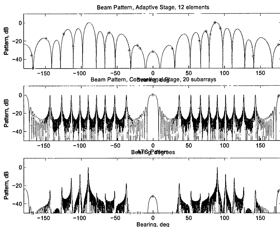
Figure 5-26: Beam patterns at the adaptive stage (top), conventional stage (middle) and composite ATC (bottom) with interferer locations superimposed.
