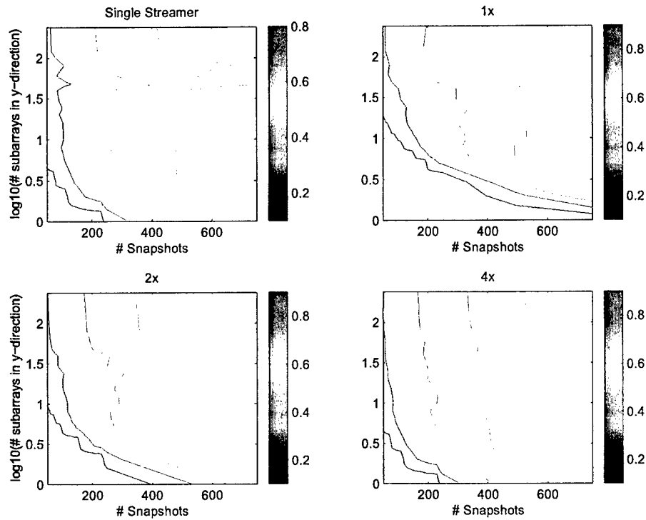
Figure 5-38: P_d vs snapshots for different subarray configurations, CTA algorithm.
