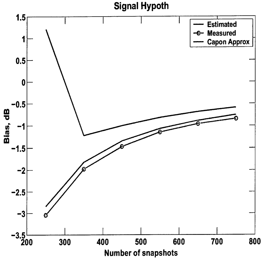
Figure 4-13: Bias predicted using a modified Capon/Goodman approximation compared to simulation when target and interferer are coherent, i.e. environment.
