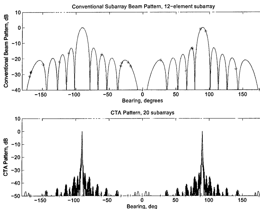
Figure 5-25: Beam patterns at the conventional stage (top) and composite CTA (bottom) with interferer locations superimposed.
