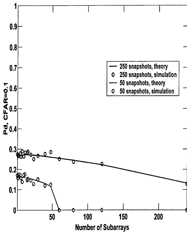
Figure 4-6: Comparison of simulated and analytical curves for CTA algorithm, interference-dominated example. L_{cs}=\infty , L_{ci}=50 elements.
