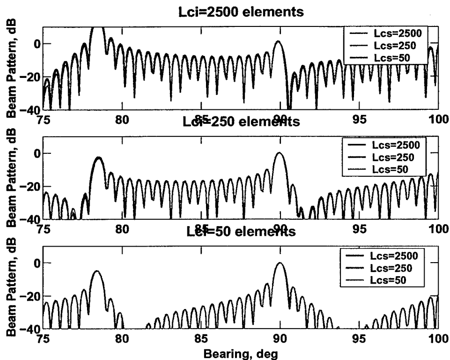
Figure 5-22: Adaptive beam-patterns for a variety of signal and interference coherences. The interference which dominates the adaptive weight computation in the ATC algorithm.
