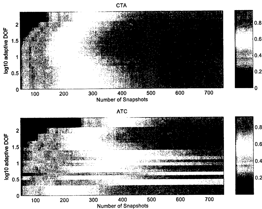
Figure 5-32: Pd vs adaptive DOF and snapshots, CTA and ATC algorithms.
