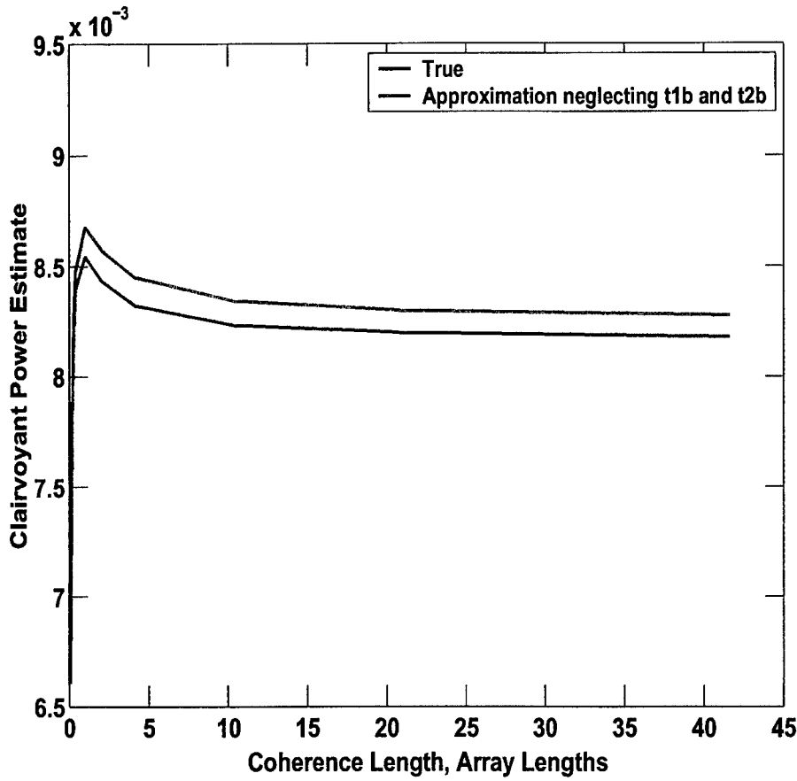
Figure 4-10: Clairvoyant ATC power estimate and approximation neglecting terms t1b and t2b for a low-energy coherence example.
