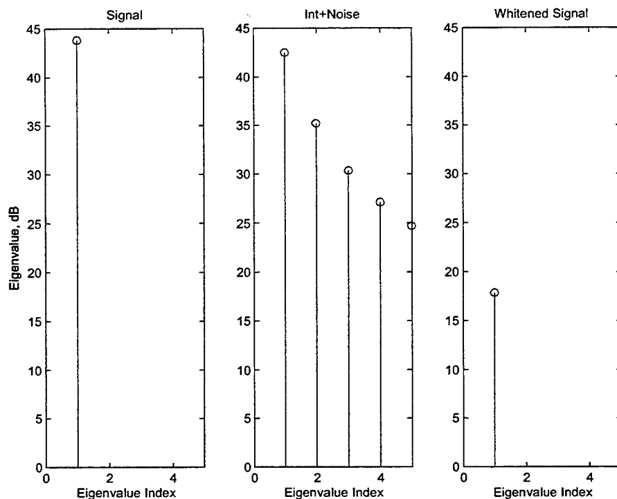
Figure 5-4: Dominant eigenvalues of the signal, interference, and whitened signal covariance for an interferer with a coherence length of 240 elements.
