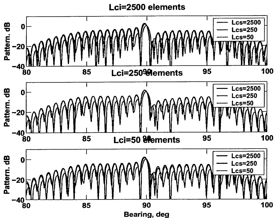
Figure 5-18: Adaptive beam-patterns for a variety of signal and interference coherences. The interference which dominates the adaptive weight computation until the target signal has experienced significant decorrelation.
