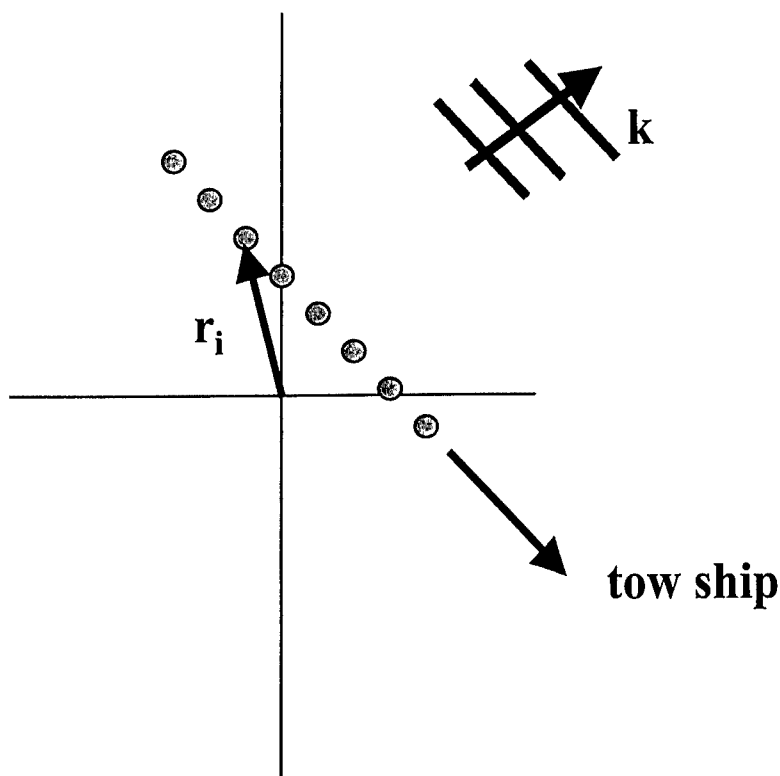
Figure 2-3: Plane wave propagation.
