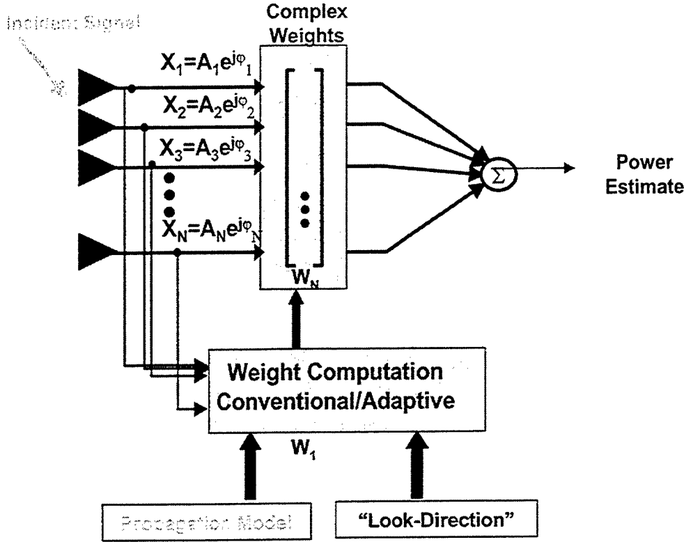
Figure 3-1: Generalized block diagram for processing stream.
