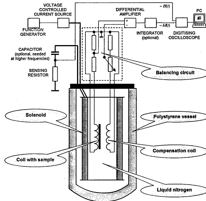
Fig. 5.2.1 The block diagram of experimental equipment.
