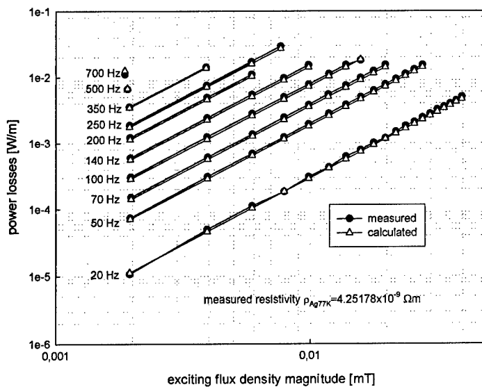
Fig. 5.2.3 The comparison of measured and calculated power losses per unit length versus the flux density magnitude at various frequencies, Ag strip sample 59x4x0.3 mm 3 , temperature 77K, sinusoidal exciting field.
