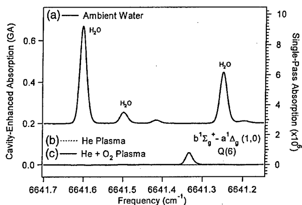
Fig. 1. Cavity-enhanced absorption (GA) measurement in the region of the Q (6) transition of the b^1\Sigma_g^+ - a^1\Delta_g (1,0) transition recorded for three different gas compositions: (a) 5-Torr ambient air, (b) flowing afterglow of a helium rf discharge, (c) discharge of (b) seeded with 5% \text{O}_2 . Spectrum (a) is offset by 0.2 absorption units.
