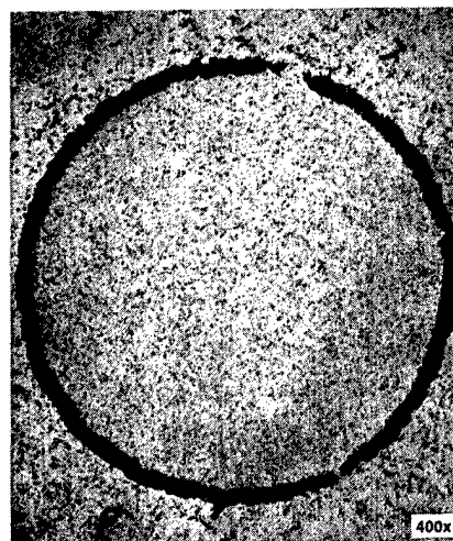
EXPOSED 921 HRS AT 1500 K
