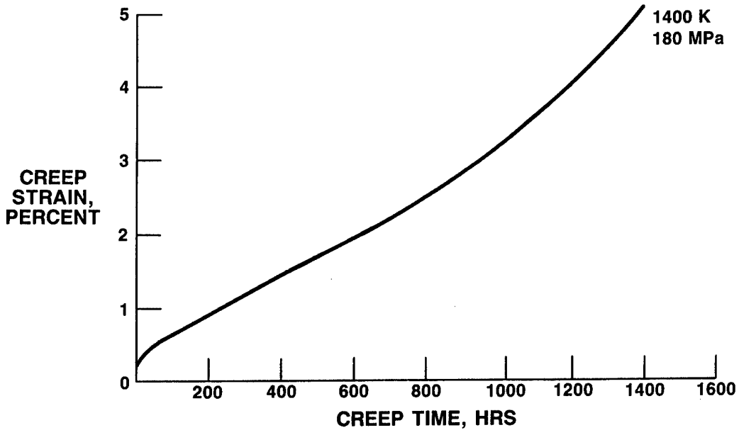
FIGURE 19. - TYPICAL CREEP CURVE FOR ST300/Nb + 1Zr COMPOSITE.
