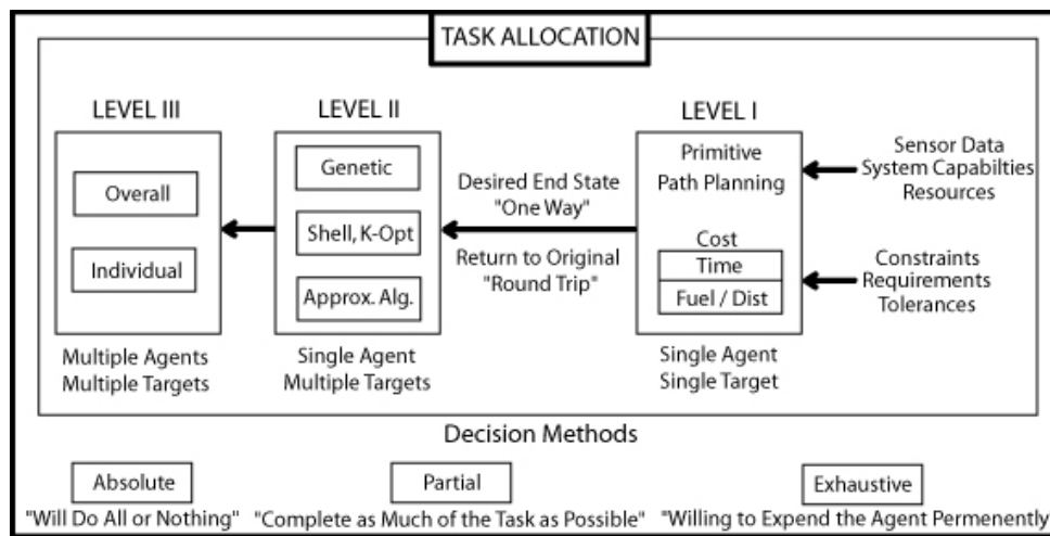
Figure 30: Three tiers of optimization for the team tasking approach based on primitives.
