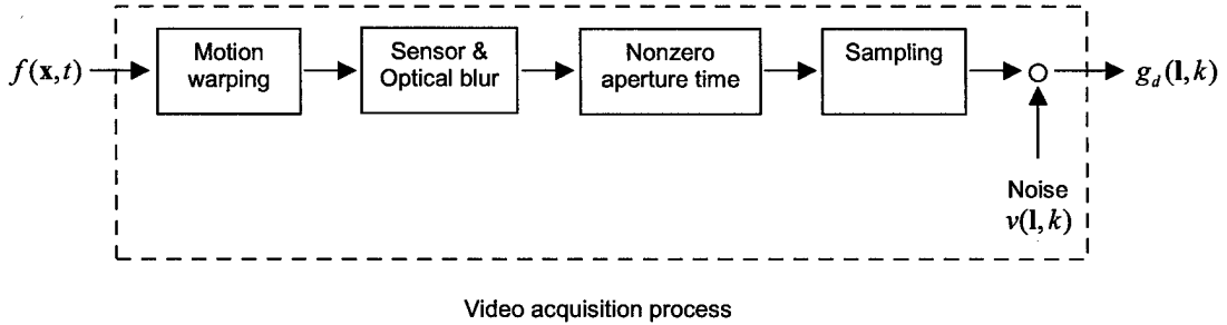
Figure 1: Video acquisition model.
