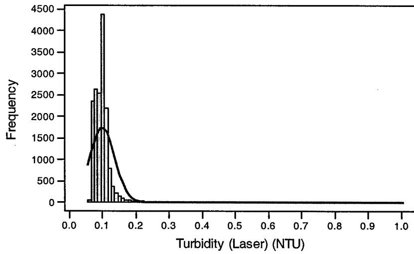
Figure B-1 Histogram of laser turbidity with normal curve.
