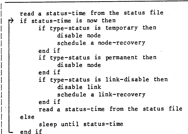
Figure 4.2.1 - Status Update Algorithm
