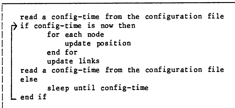
Figure 4.2.2. Configuration Update Algorithm
