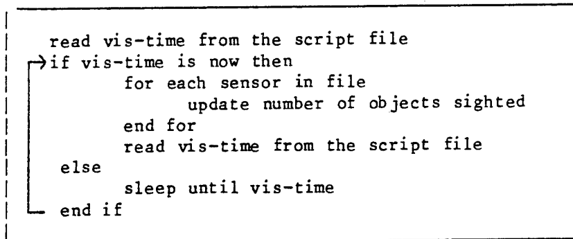
Figure 4.2.3 - Sensor Update Algorithm
