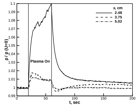
Figure 10 Effect of DC discharge on flat plate surface pressures. Pressures are normalized by undisturbed ( U=0 ) static pressures.
