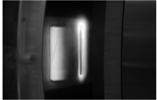
Figure 29 Plasma discharge generated across the cross stream model electrodes, the upstream electrode is the cathode, the current is 50 mA, and the magnetic field strength is -0.35 tesla.
