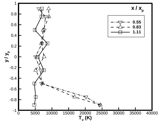
Figure 12 Electron temperature in a 50 mA discharge, no-flow case.
