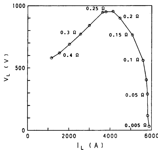
Fig. 29. From [22]. Current to voltage characteristic of non-equilibrium disk Hall generator.
