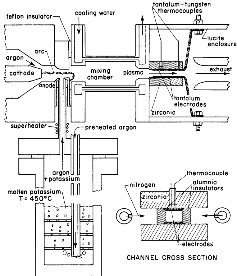
Fig. 1. From [1]. Experiment to demonstrate electron temperature elevation.
