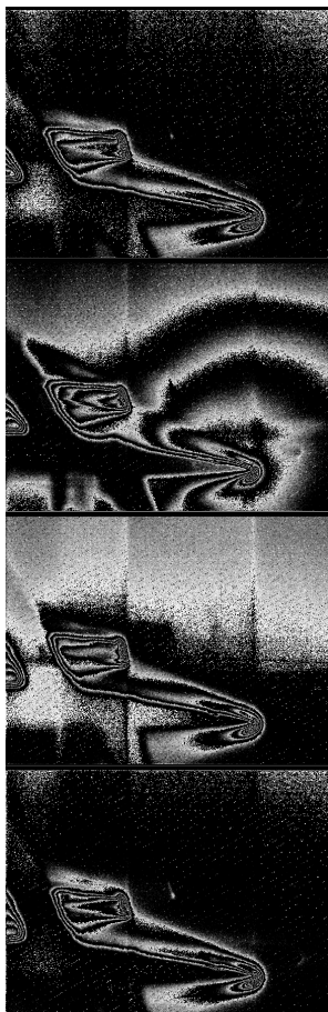
Figure 44a . Run 137 07.21.2003. The Cowl-Wedge Model, Visualization With the spectral filtering with followed digital filtering
