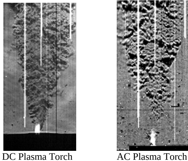
Fig. 9 Flow field structure from different plasma torches
