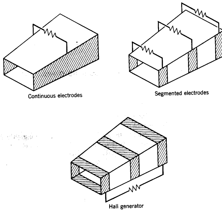
Fig. C2. From [24]. Common electrode configurations in linear channels.
