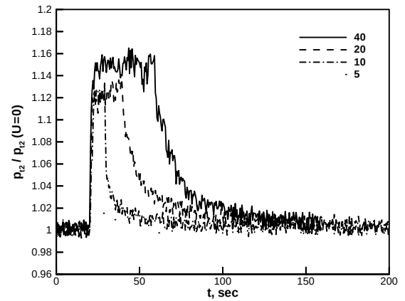
Figure 14 Ratio of average Pitot pressure during discharge to undisturbed Pitot pressure for four different discharge durations.
