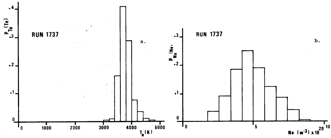
Fig. 13. From [9]. Probability distribution functions of electron temperature and electron density.
