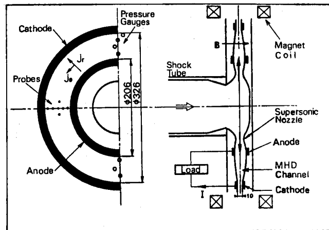
Fig. C3. From [23]. Hall disk geometry.
