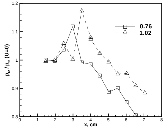
Figure 13 Average Pitot pressure during discharge normalized by undisturbed Pitot pressure as a function of distance along the model for two heights above the plate.
