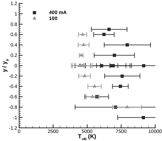
Figure 22 Vibrational temperatures for 100 and 400 mA DC discharge between plates, vertical distribution at x / x_p = 0.7 .
