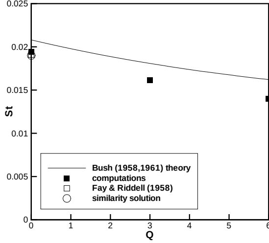
Figure 5: Effect of applied magnetic field on stagnation point heat transfer.
