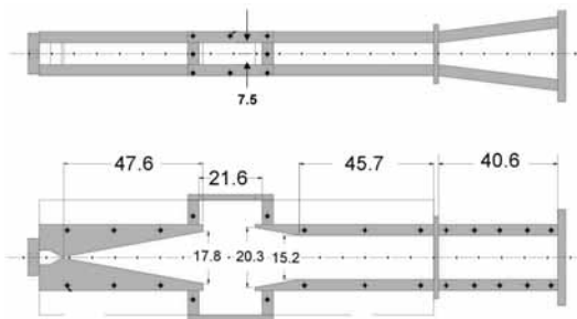
Figure 1 Schematic of the plasma channel. All dimensions centimeters. Flow is from left-to-right
