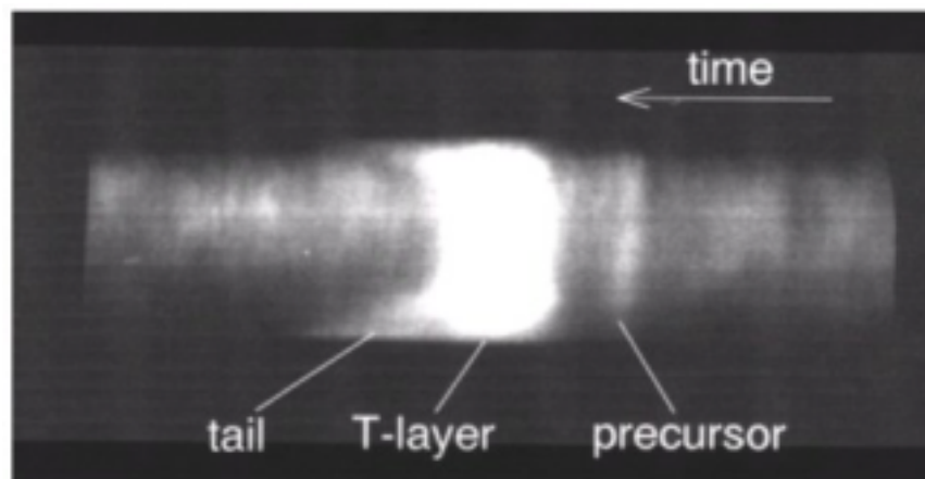
Figure 6: Streak camera picture of a T-layer in the shock tunnel experiment.
