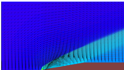
Figure 41. Pressure, flow stream lines and magnetic field vector distribution in the flow around the extended wedge.
