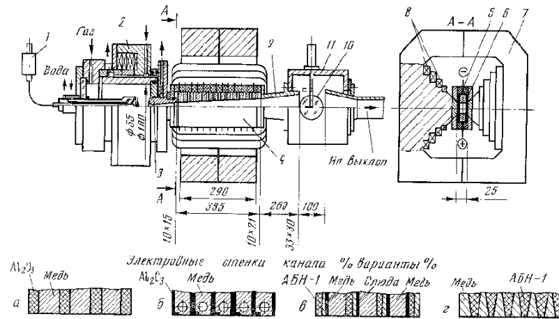
Figure 19. Schematic diagram of the TsAGI MHD WT facility.
