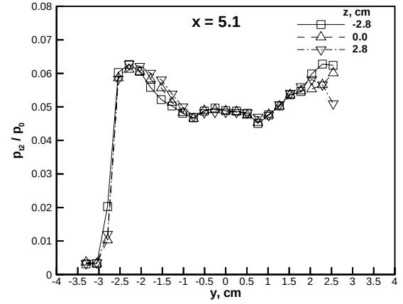
Figure 6 Pitot survey in spanwise direction at three vertical locations, x=5.1 cm.
