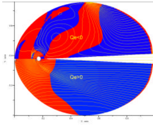
Fig.29. The electrical power released (red) and extracted (blue) from the flow for two cases: the upper – non-shortcd conditions, the bottom – shortcd conditions.
