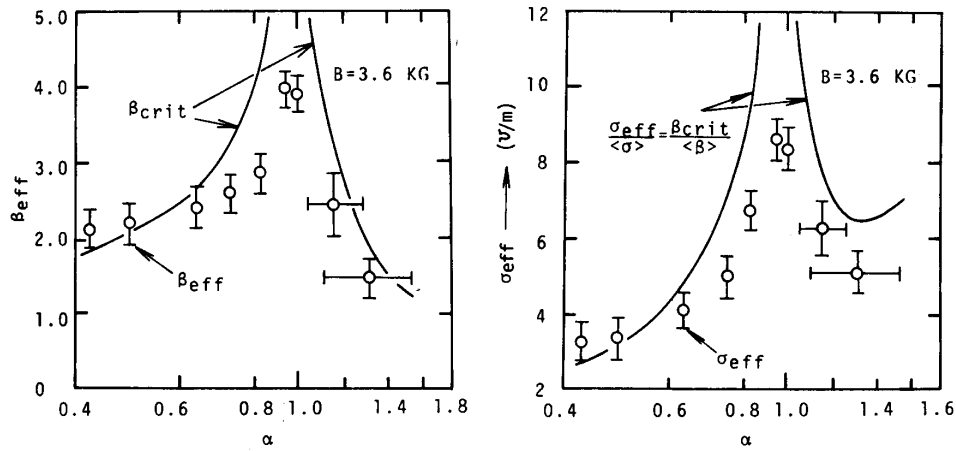
Fig. 26. From [20]. Effect of fully ionized seed on Hall parameter and electrical conductivity. Magnetic field was 3.6 Tesla.
