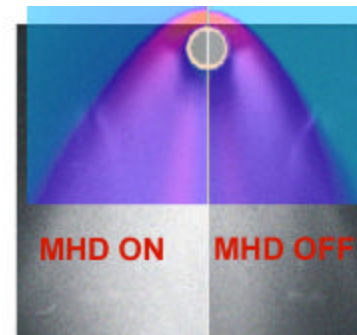
Fig.23. The visualization (b&w) and computation (colored) comparison of the wake area flow field under MHD-off and MHD-on conditions.
