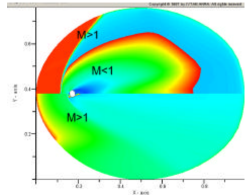
Fig.30. Comparison of the Mach number distribution in two cases. The upper half represents the non-shortcd conditions case, the bottom half – the shortcd conditions case.
