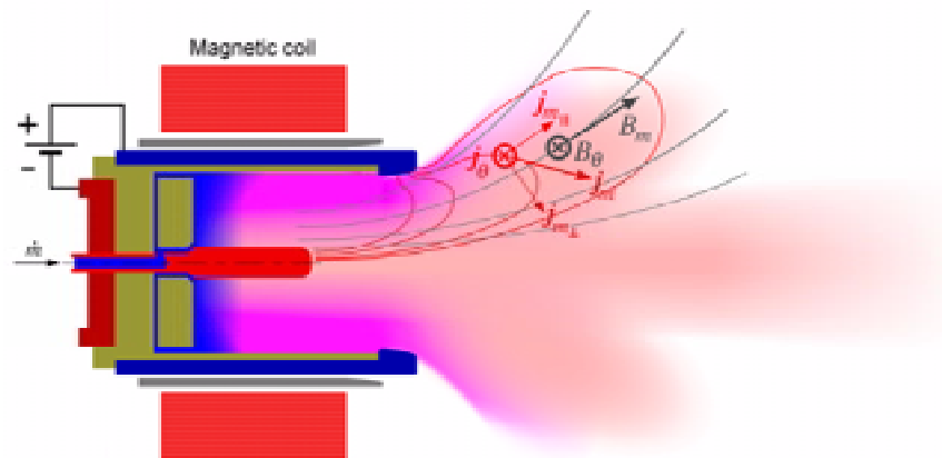
Fig. 7 General scheme of applied-field MPD thruster
