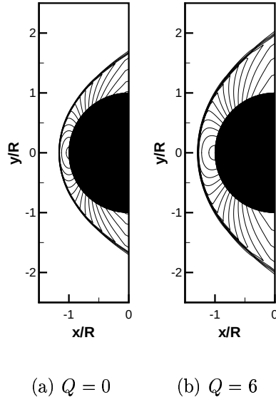
Figure 1: Pressure field p/p_\infty for inviscid flow (contour interval 2).
