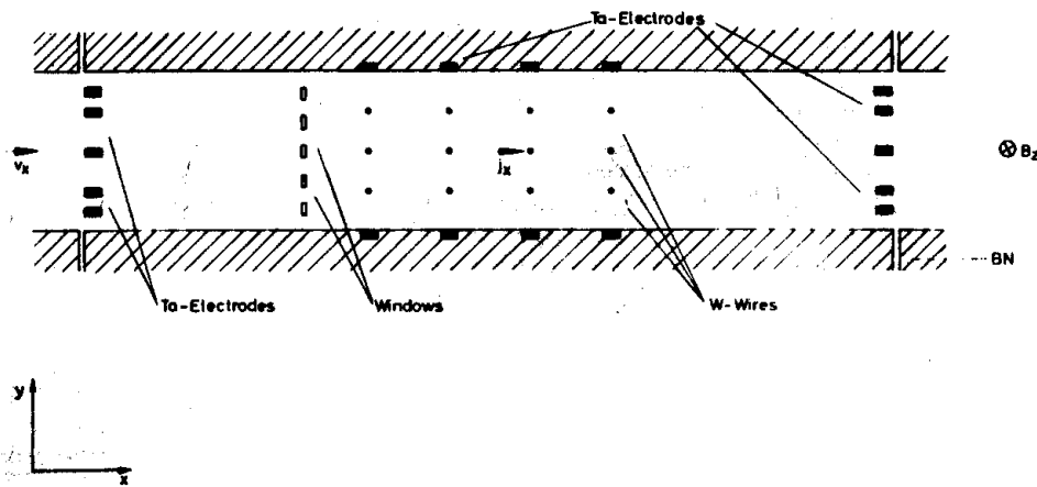
Fig. 6. From[6]. Arrangement of diagnostics in an experimental MHD channel. The wires are used as voltage probes. The channel is 100 mm long, 20 mm high and 15 mm wide. Tungsten wires were 0.5 mm in diameter
