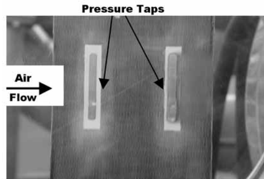
Figure 25 Crossflow-electrode model showing pressure taps.
