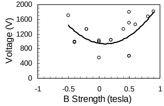
Figure 27 Voltage required to produce 50 mA current in transverse surface discharge as a function of applied magnetic field.
