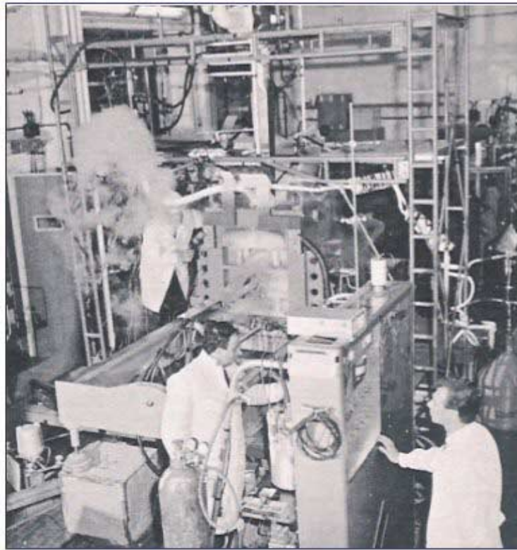
Figure 1: MHD blow-down facility in Frascati.
