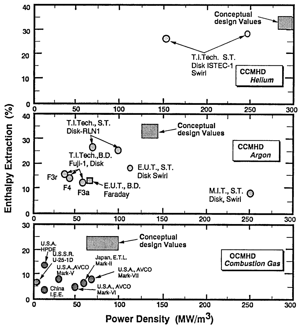
Fig. 32. From [25]. Worldwide overview of MHD generator performances.
