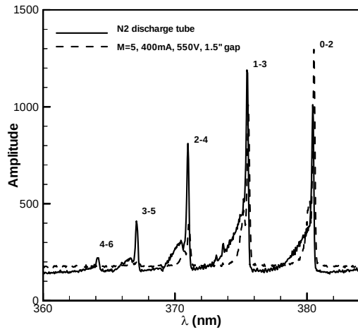
Figure 9 Nitrogen second positive group spectra for static discharge tube and Mach 5 DC glow discharge.
