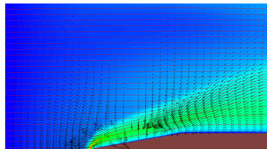
Figure 42. Temperature, flow stream lines and body force vector distribution in the flow around the extended wedge.
