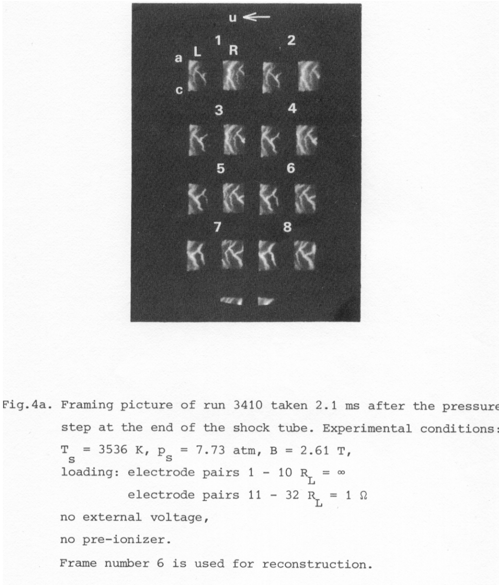
Fig. 18. From [12]. Streamers in a shock tube MHD generator. Two pictures L and R are simultaneously taken from different view points under an angle of 26.4^\circ .
