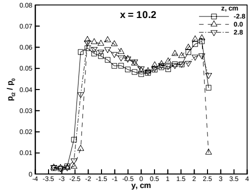
Figure 7 Pitot survey in spanwise direction at three vertical locations, x=10.2 cm.
