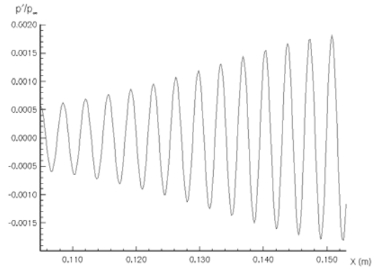
Figure 4 Instantaneous second-mode wall pressure fluctuations in a flat-plate, non-MHD, M=4.5 boundary-layer (Ref. 39).
