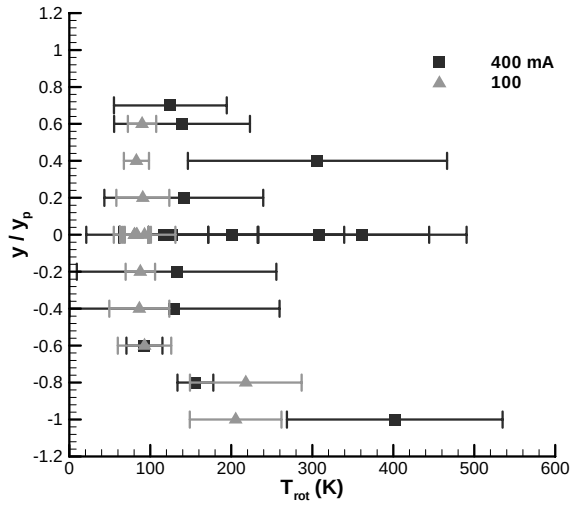
Figure 21 Rotational temperatures for 100 and 400 mA DC discharge between plates, vertical distribution at x / x_p = 0.7 .
