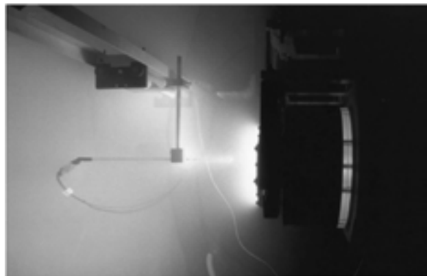
Fig. 9 An HPT applied-field thruster under test at Centropazio-Alta Laboratories
