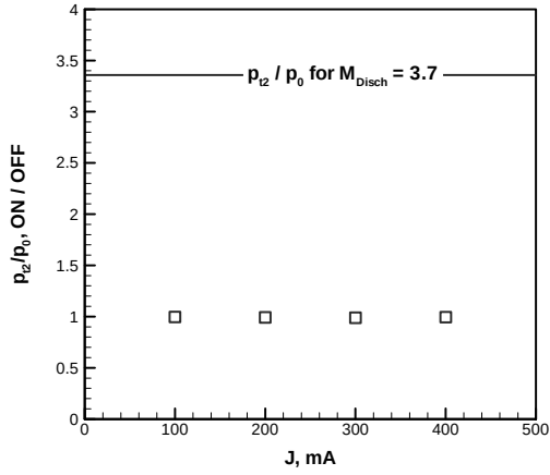
Figure 17 Ratio of current-on Pitot pressure to current-off Pitot pressure
