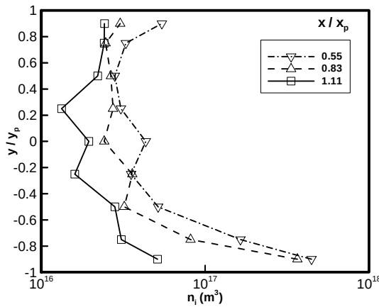
Figure 10 Ion number density in a 50 mA discharge, no-flow case. In this and next figures, spanwise location is in the center of the electrodes.
