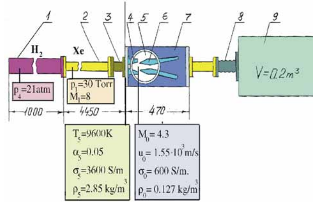
Figure 6. Scheme of the experiment at Small Shock Tube: 1 is high-pressure chamber, 2 is low-pressure chamber, 3 is measurement section of a low-pressure chamber, 4 is acceleration nozzle, 5 is optical window, 6 is diffuser model, 7 is vacuum chamber, 8 is Sylphon, 9 is exhaust tank.
