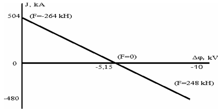
Figure 11. Loading Characteristics of a Single Section of MHD Converter.
