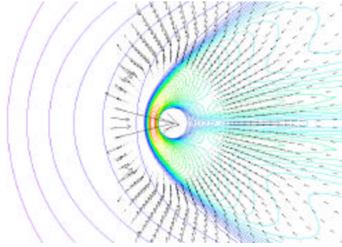
Fig.28. The planar component of the body force vector distribution in close-up cylinder area. The length of the vectors represents relative value of the physical quantity.
