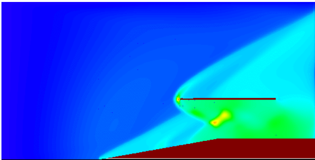
Figure48. Pressure distribution for the conditions of Run 138. Magnetic field 2.5T at the lead surface.
