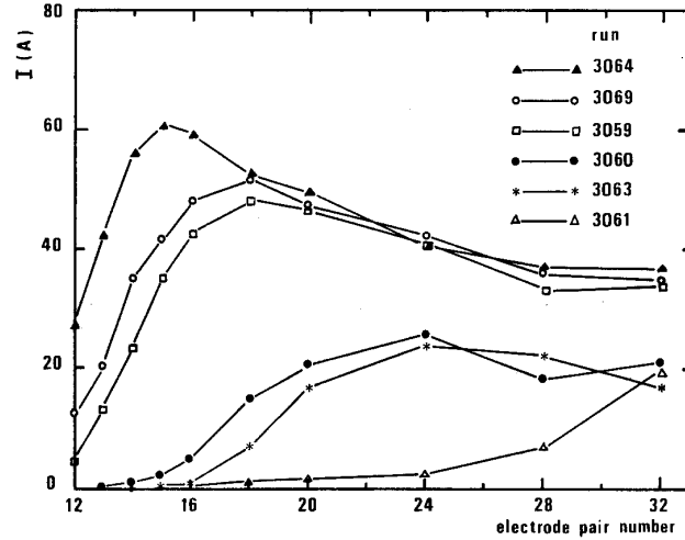
Fig. 21. From [15]. Inlet relaxation effect on current distribution. Runs represent different stagnation temperatures, increasing from 2560 K (run 3061) to 3370 K (run 3064).
