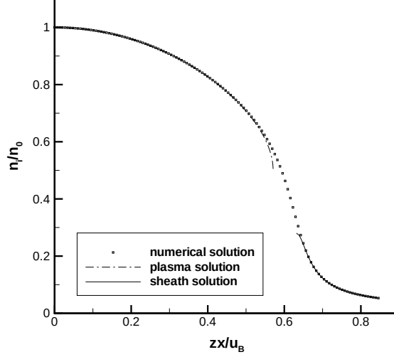
Figure 8: Ion number density predicted by analytical and numerical methods. Every fourth computational point shown. Neither analytical approximation is valid in the gap near \hat{x} \approx 0.6 .
