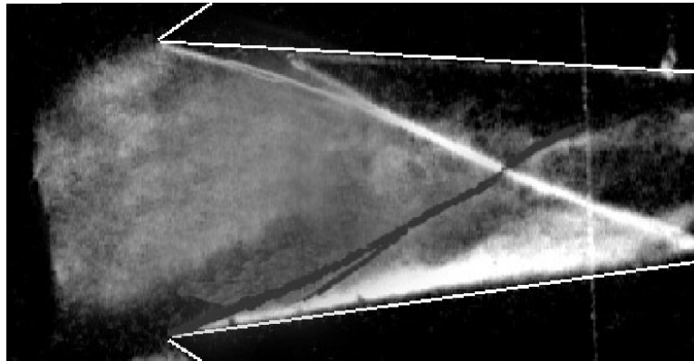
Figure 8. Examples of changes in shock-wave configurations exposed to electric and magnetic fields.
