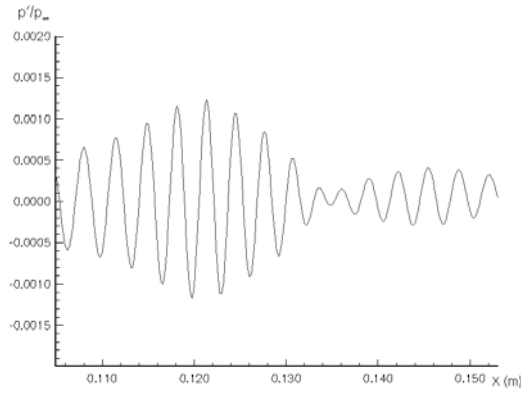
Figure 5 Instantaneous second-mode wall pressure fluctuations in a flat-plate, MHD boundary-layer flow through a 1.2 T field, M=4.5 (Ref. 39).
