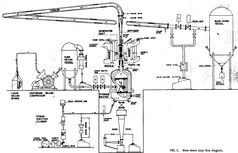
FIG. 1. Blow-down loop flow diagram.
