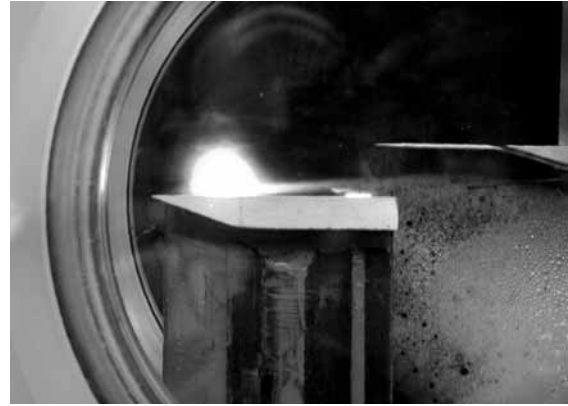
Figure 9 DC surface discharge on flat plate model. Flow is from left-to-right.
