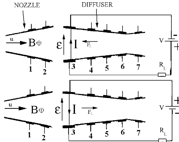
Figure 7. Scheme of current localization.
