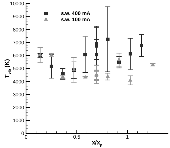
Figure 20 Vibrational temperatures for 100 and 400 mA DC discharge between plates, streamwise distribution at y/y_p = 0.0 .
