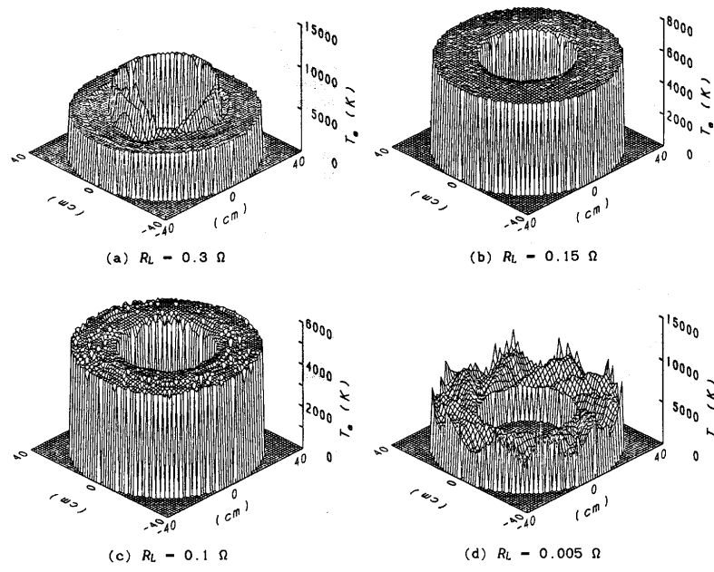
Fig. 30. From [22]. Electron density distribution in a non-equilibrium disk hall generator.
