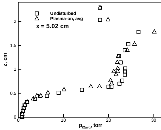
Figure 12 Pitot pressure survey above downstream electrode (anode) on flat plate.
