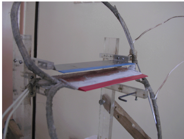
Figure 43. The Cowl-Wedge Model on the holder. The cowl (blue edge) is located above the active zone of the wedge (red edge). The external leads of magnetic system are turned counterclockwise direction to extend the observation area of the flow near the inlet.
