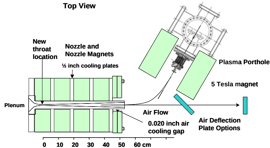
Fig. 3 Electron beam energy source in high-speed tunnel, Courtesy of Miles (Ref. 23)
