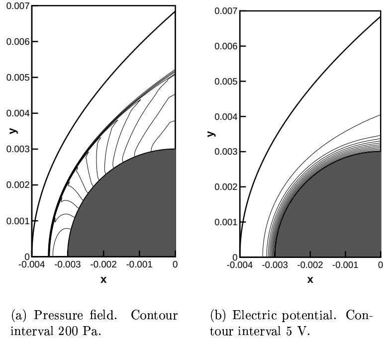
Figure 11: Numerical solution in center plane.
