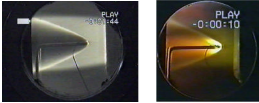
Figure 15. A model in the test section before and during the MHD acceleration
