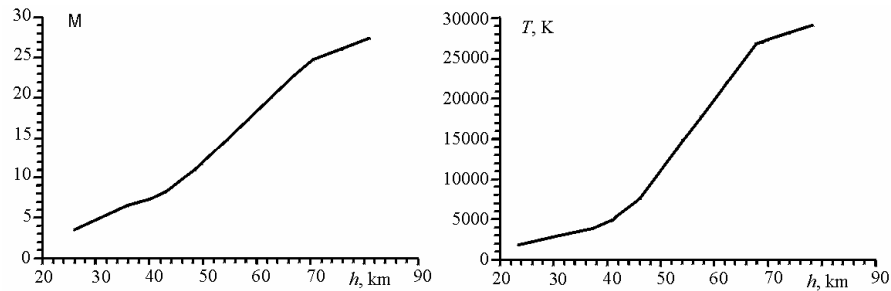
Figure 3 Mach Number and Temperature behind the Shock Wave along the Gliding Trajectory.
