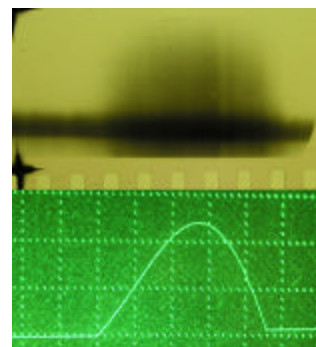
Fig. 17. The streak photography record. The time from left to right 0.4msec/div, flow
