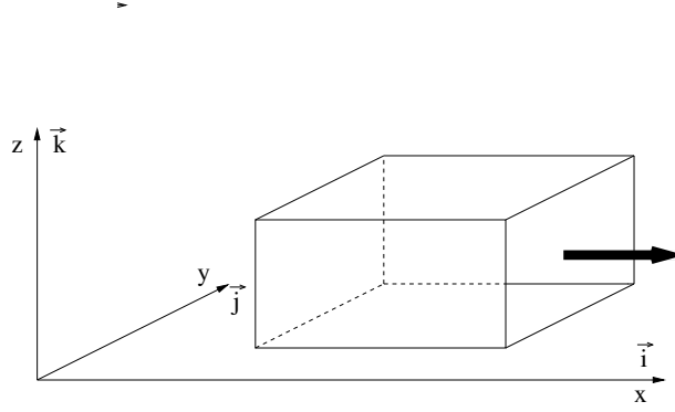
Fig. 1 One-dimensional MFD model.
