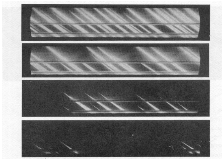
Fig. 22. From [15]. Streamer development for different stagnation temperatures, from top to bottom 3370, 3080, 2800 and 2580 K.
