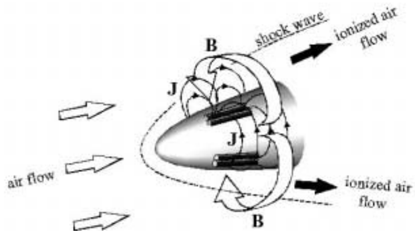
Figure 12: Scheme of the MHD interaction on an hypersonic vehicle.
