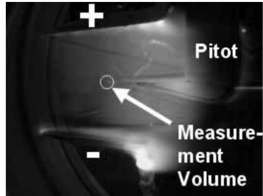
Figure 8 Photograph of discharge with Pitot probe.
