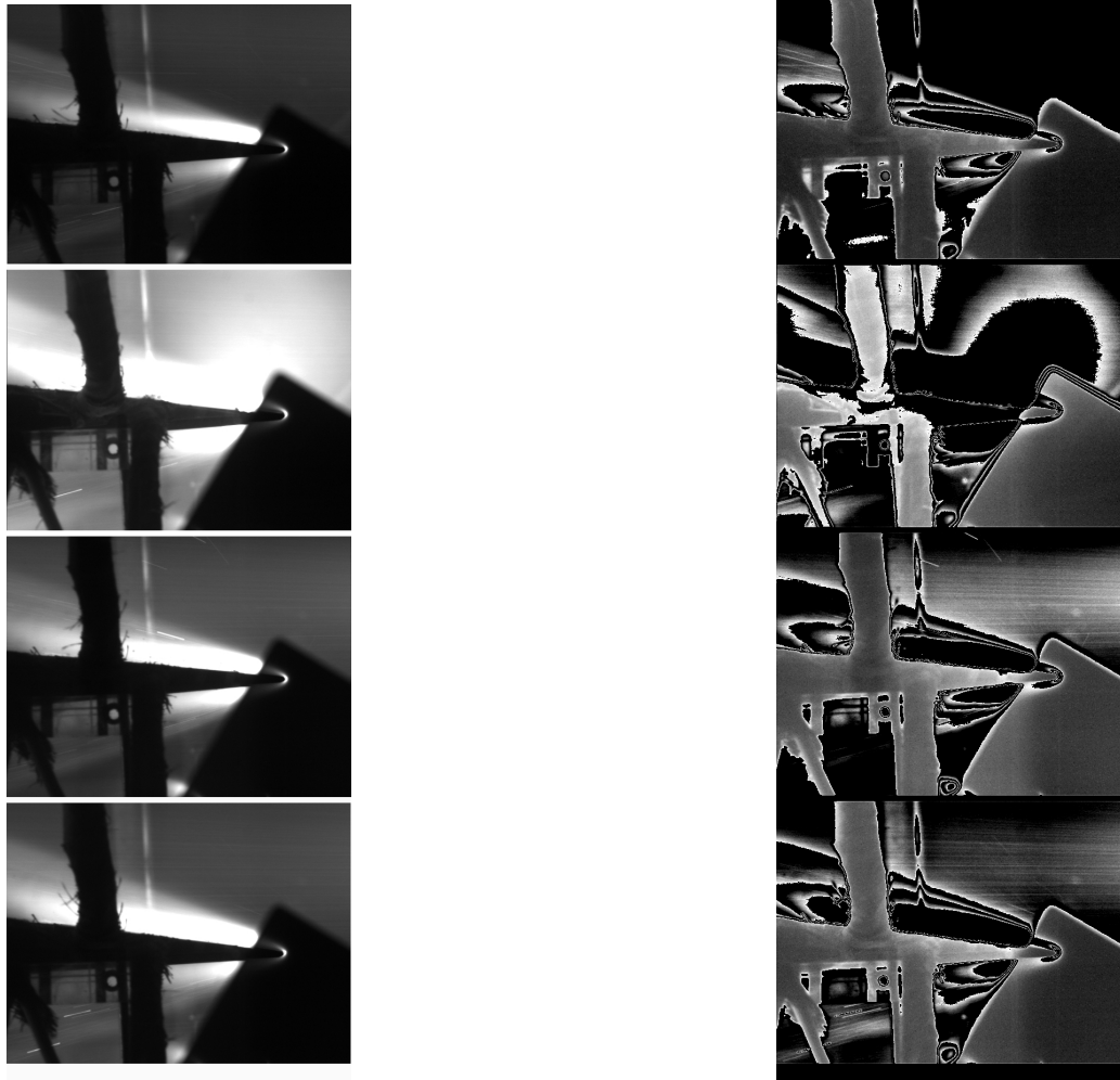
Figure 37. The visualization of flow around the wedge model. Run 132 04.24.2003. Flow from the right to the left. Four consequence frames are presented. Digital camera Pulnix-6710, 250fps, exposure time 30 mks. The left column is original imaging, the right column is the filtered image.
