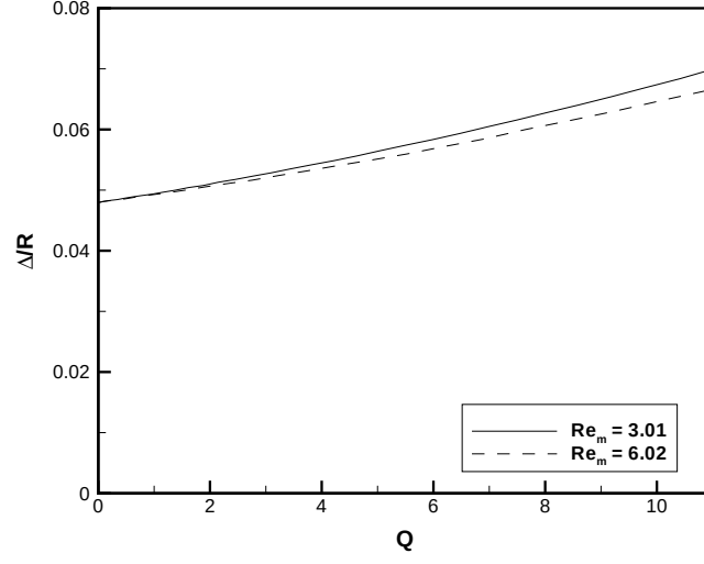
Figure 6: Effect of varying magnetic field strength on shock standoff at M = 25 .
