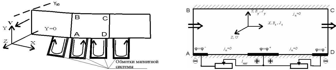
Figure 9 Geometry of MHD Generator, Numerical Simulation Domain and Boundary Conditions used in Numerical Simulation.
