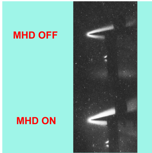
Figure 34. Visualization of flow around the wedge model.
