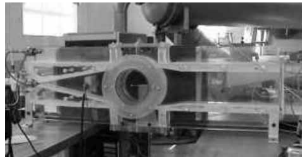
Figure 2 Photograph of the Mach 5 Plasma Channel.
