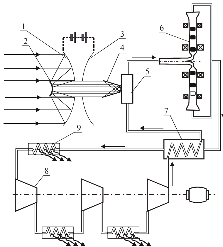
Figure 14. Scheme of power facility. 1, 2 – primary and secondary mirrors, 3 – film with surface electric charge, 4 – funnel of radiator condensor, 5 - radiation receiver, 6 – MHD generator channel, 7 – recuperative heat exchanger, 8, 9 - compression group with intermediate radiation cooling
