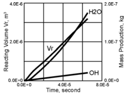
Figure 10. Reacting Volume and Mass production of H_2O and OH vs time
