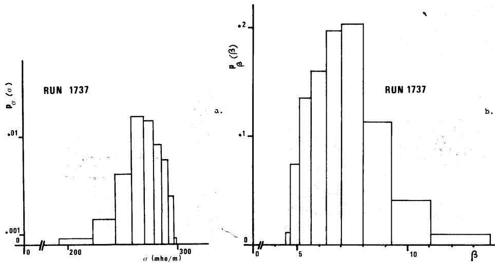
Fig. 14. From [9]. Probability distribution functions of electrical conductivity and Hall parameter.
