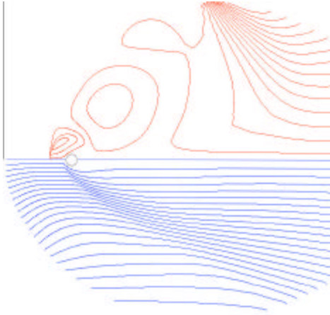
Fig.25. The electrical current stream lines are as for non-shorted (red, upper half) and shorted (blue, bottom half) conditions.
