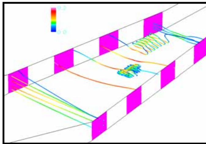
Fig. 8 Hall current in MHD Scramjet, Courtesy of Gaitonde (Ref. 53)
