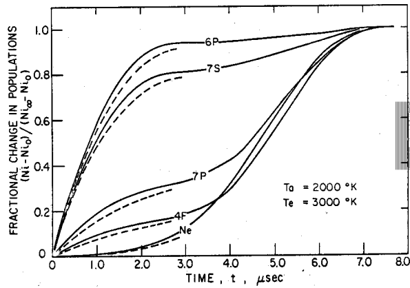
Fig. 20. From [14]. Time development of electron density and populations of excited states of cesium following a stepwise increase of the electron temperature from 2000 to 3000 K.
