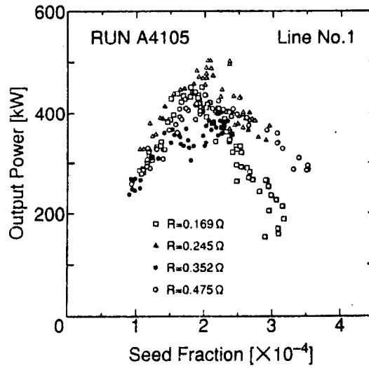
Fig. 28. From [21]. Electrical output vs. seed fraction in a non-equilibrium disk generator.
