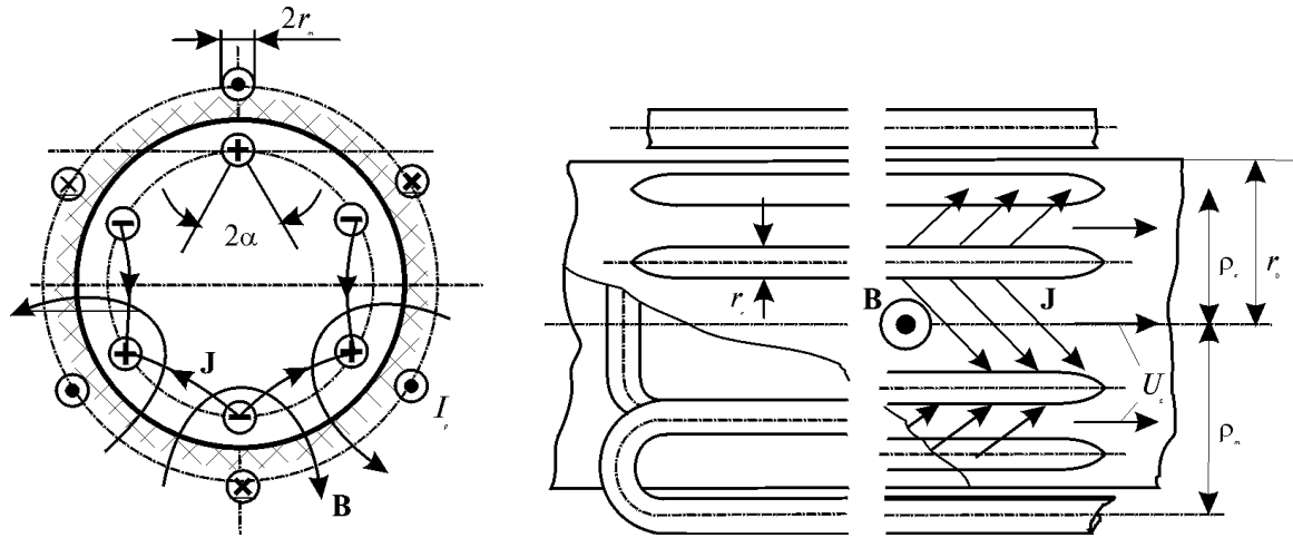
Figure 12. Schematic of Multipole MHD Generator Built-in Rocket Engine - cross-section view (left) and – side view (right)
