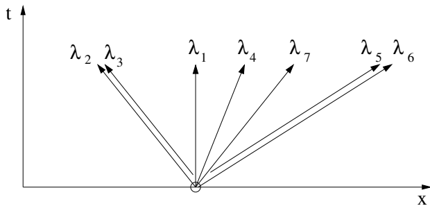
e) Characteristics pattern for the 1D MFD flow with B_x > \sqrt{\gamma p} and B_t = 0 .
