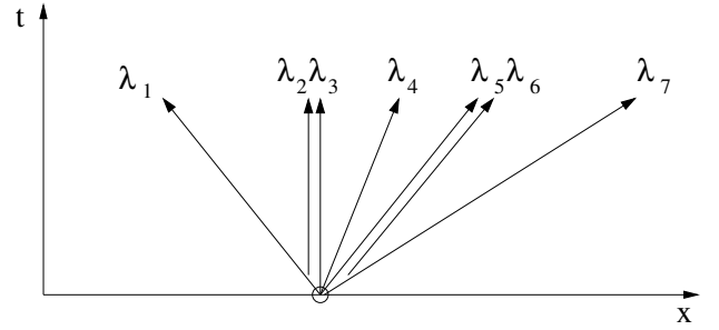
d) Characteristics pattern for the 1D MFD flow with B_x < \sqrt{\gamma p} and B_t = 0 .
