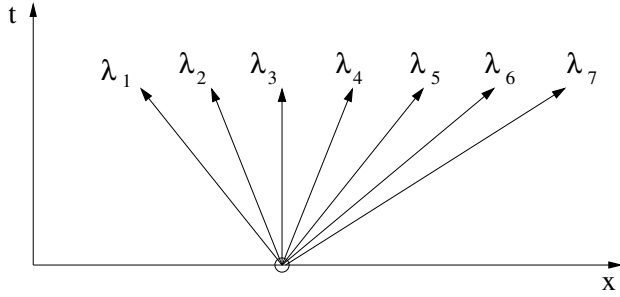
a) Characteristics pattern for the general 1D MFD flow.
