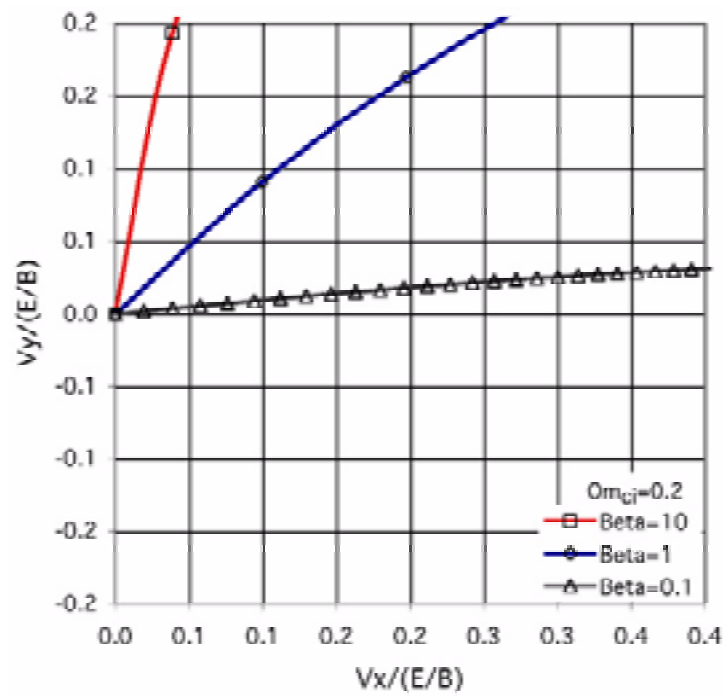
Fig. 2b Initial trends of the above solutions (magnification)
