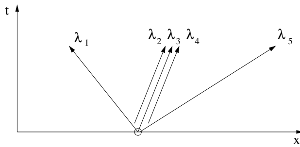
Fig. 2 Characteristics pattern for the 1D Euler flow.
