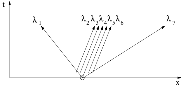
c) Characteristics pattern for the 1D MFD flow with B_x = 0 and B_t \neq 0 .
