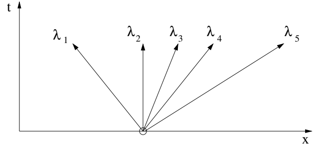
b) Characteristics pattern for the planar 1D MFD flow.
