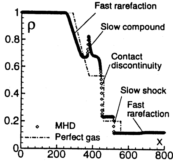
Fig. 2 Density profile in shock tube, Ref (28).
