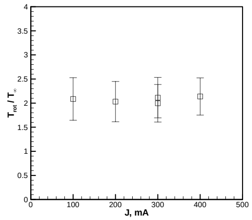
Figure 16 Rotational temperatures measured in discharge as a function of current. Error bars represent \pm 10 K uncertainty.
