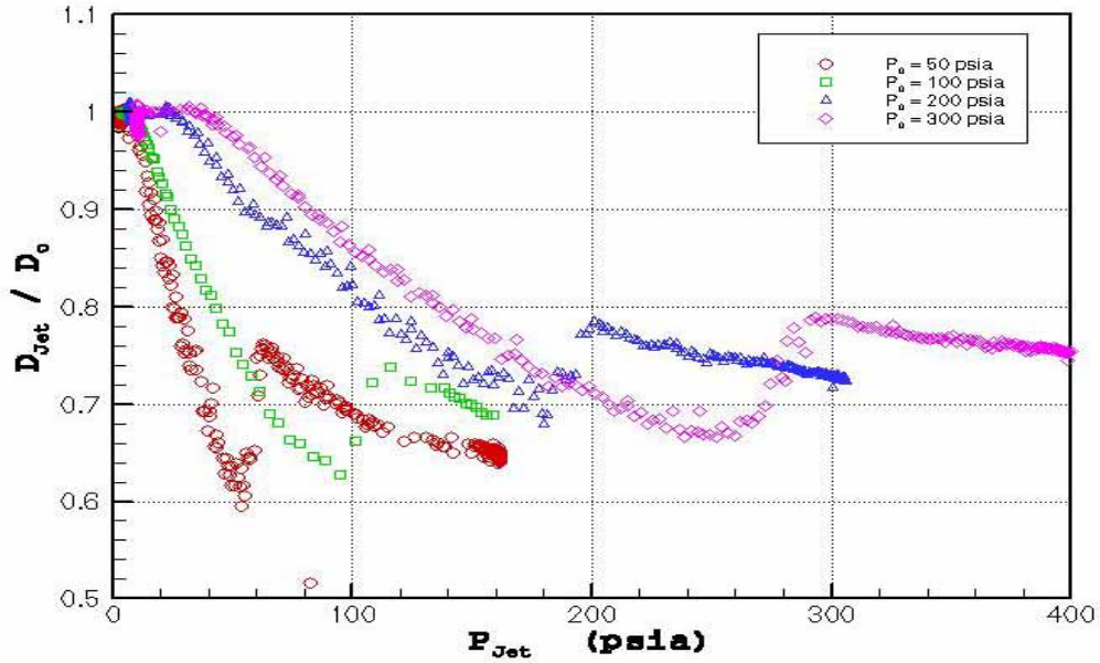
Fig. 6 Wave drag reduction by the counter-flow jet
