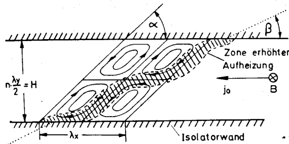
Fig. 17. From [11]. Current distribution of the ionization instability as a result of a linear calculation for a channel with insulating walls.
