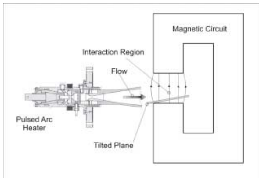
Figure 15: Scheme of the hypersonic flow-MHD interaction experiment.
