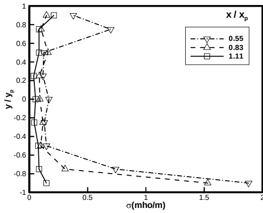
Figure 14 Plasma conductivity in a 50 mA discharge, flow-off case.
