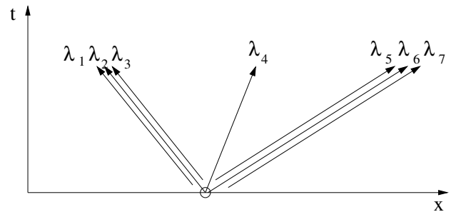
f) Characteristics pattern for the 1D MFD flow with B_x = \sqrt{\gamma p} and B_t = 0 .
