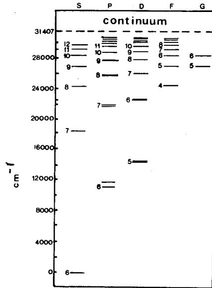
Fig. VI.6. The cesium energy level diagram.
