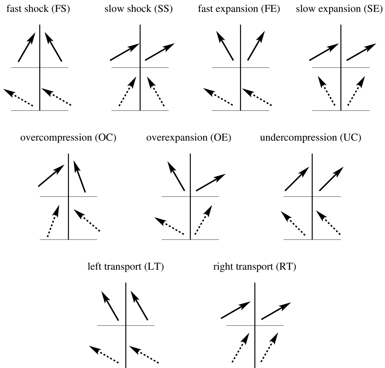
Fig. 5 Different characteristic configurations for planar 1D MFD discontinuities.
