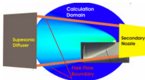
Fig. 21. The calculation domain used in the recent simulations.
