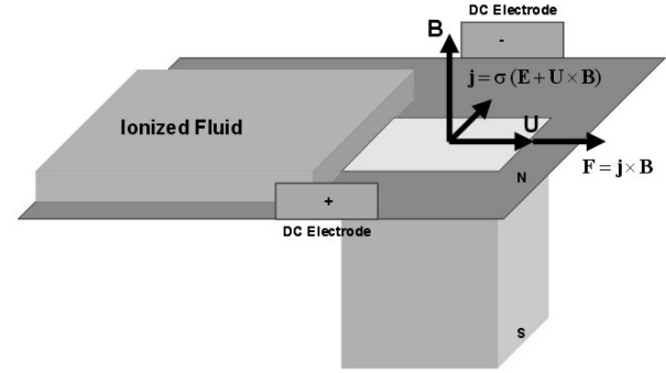
Figure 3 Forces and currents in MHD flow of ionized fluid.
