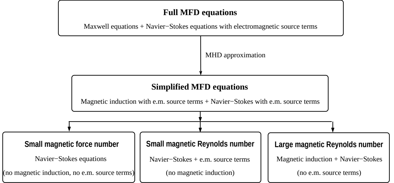
Fig. 1 Schematic view of the MFD physical models.
