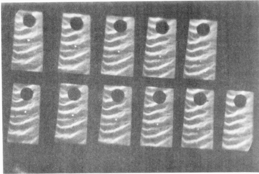
Fig. 19. From [13]. Framing photograph showing a spark surrounded by streamers. In the picture the flow velocity points vertically down. Exposure time of each frame: 1\ \mu\text{s} . Inter-frame time 5\ \mu\text{s} . Approximate size of the window: 10 \times 20\ \text{cm}^2 . Time sequence of the pictures: first from top to bottom, then from left to right.
