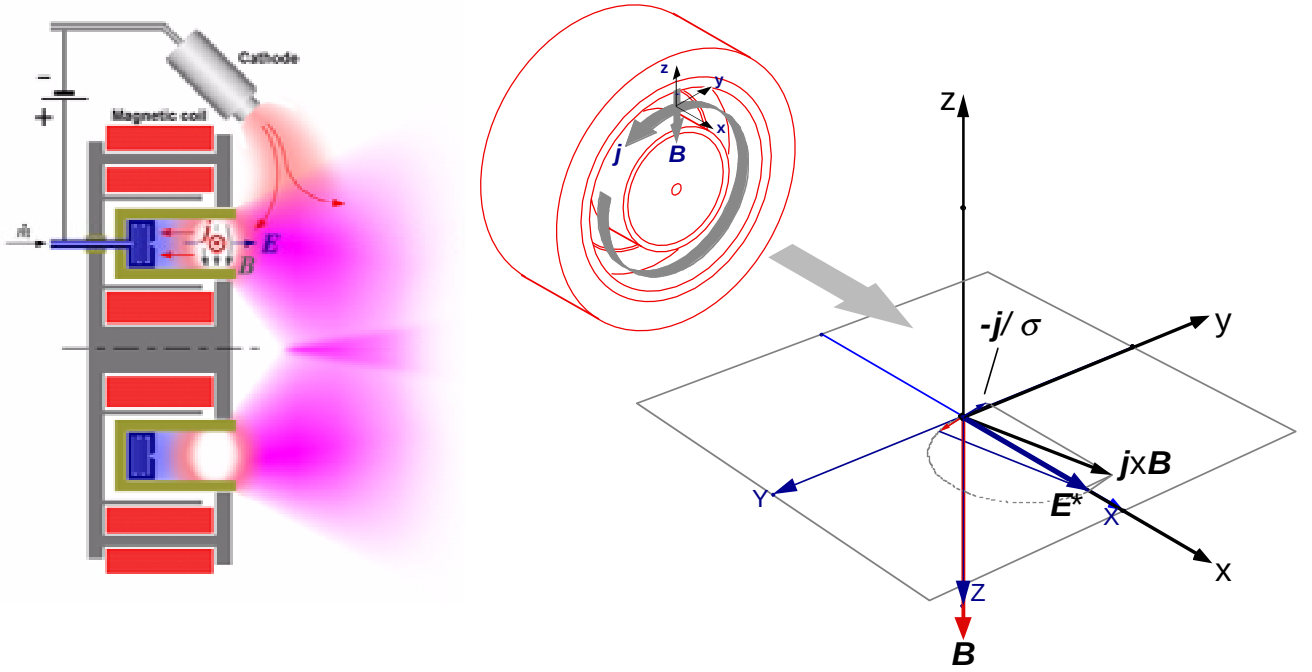
Fig. 3 General scheme of Hall effect thruster
