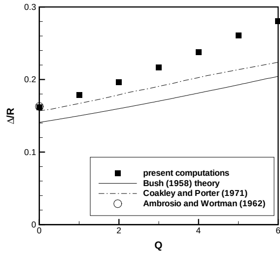
Figure 2: Effect of applied magnetic field on shock standoff.
