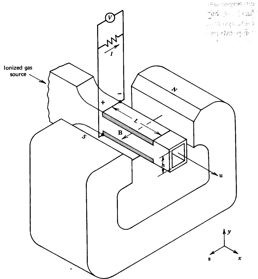
Fig. C1. From [2]. Schematic of the general MHD generator configuration.
