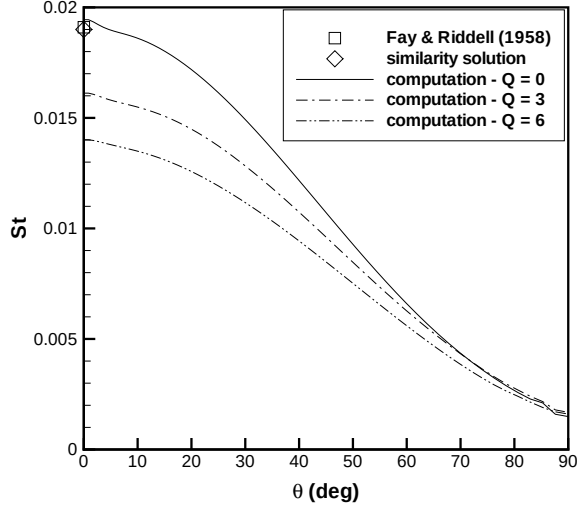
Figure 4: Effect of applied magnetic field on surface heat transfer profile.
