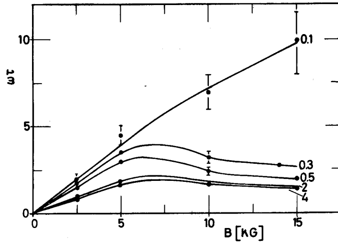
Fig. 11. From [6]. Hall parameter vs. magnetic induction for several values of current density [A/cm²]
