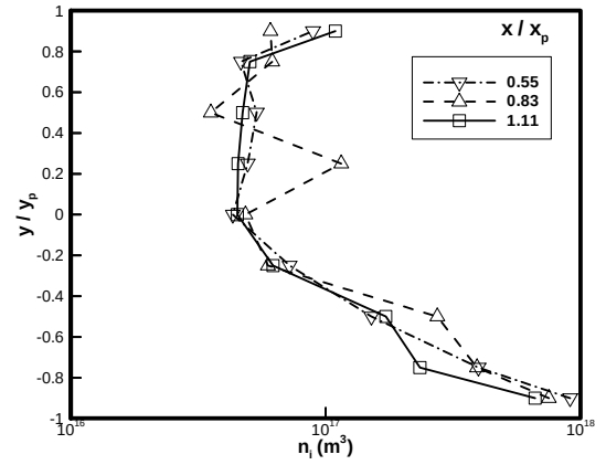
Figure 11 Ion number density in a 50 mA discharge, flow-on.
