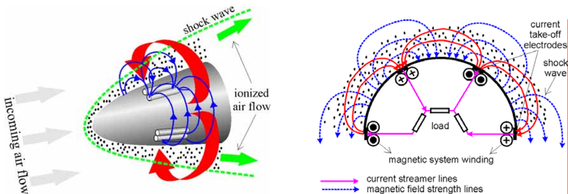
Figure 11. The schematic of the multi-pole magnetic system installed on a hypersonic spacecraft.
