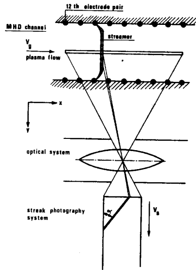
Fig. D1. From [17]. Set-up for streak photography.
