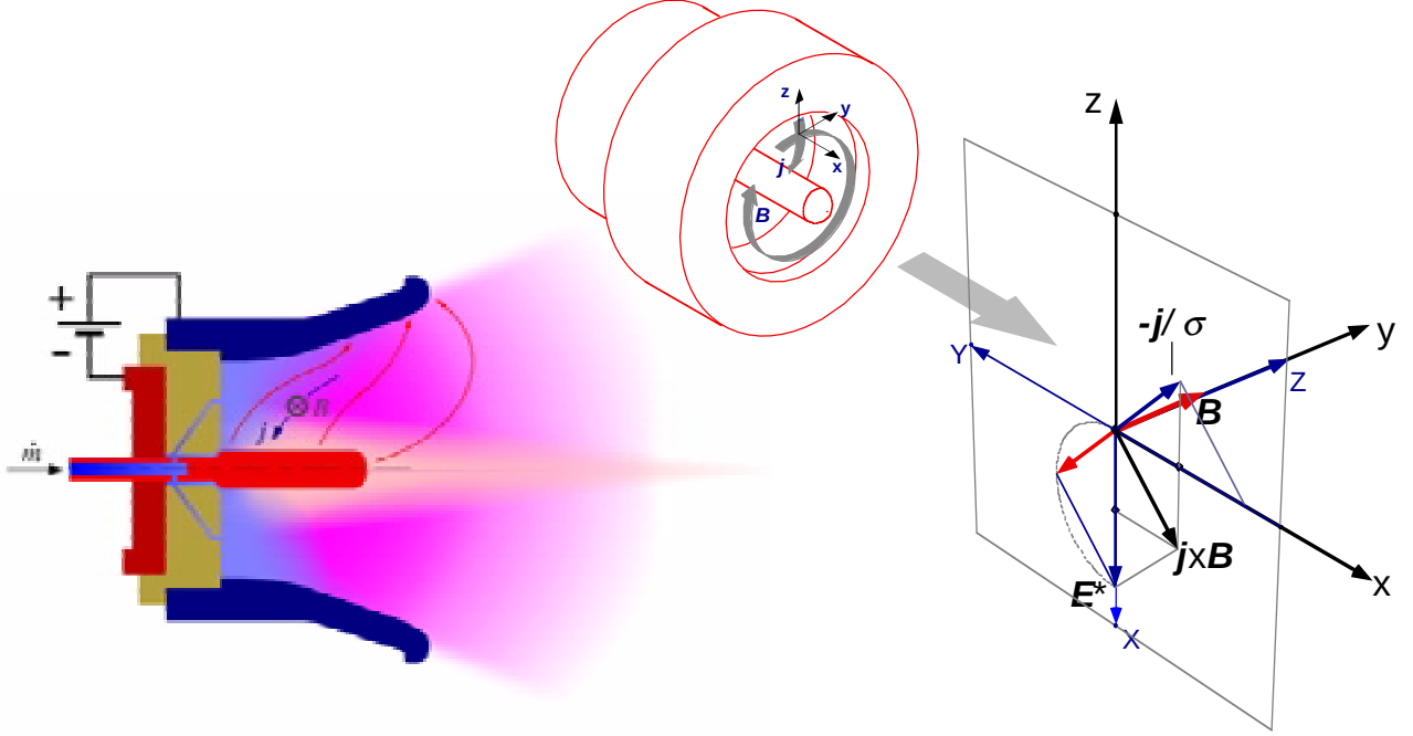
Fig. 5 General scheme of self-field MPD thruster
