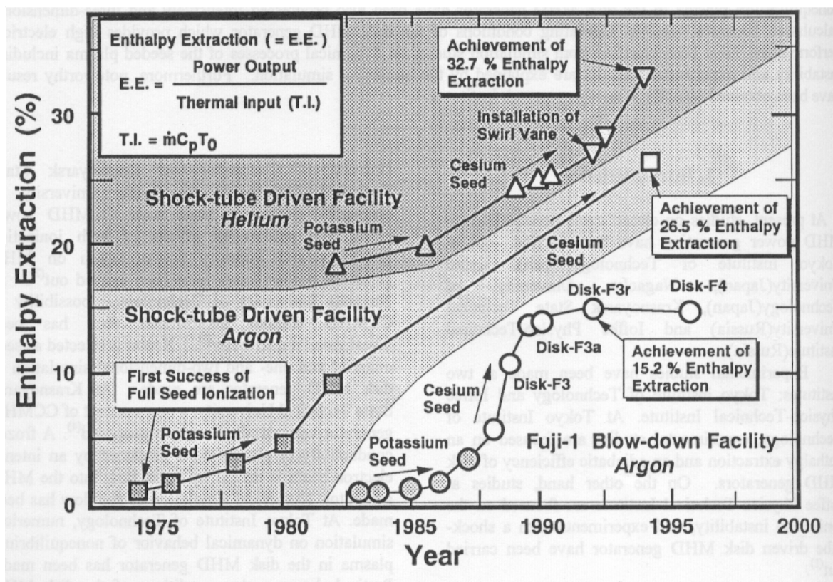
Fig. 31. From [25]. Performance of non-equilibrium generator experiments at Tokyo Institute of Technology, mostly with FIS.
