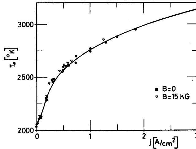
Fig. 9 From [6]. Electron temperature vs. current density with and without magnetic field.
