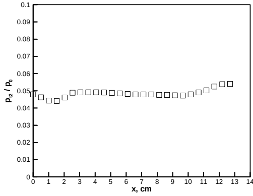
Figure 3 Ratio of Pitot to stagnation pressure along channel centerline. x = 0 corresponds to the nozzle exit.
