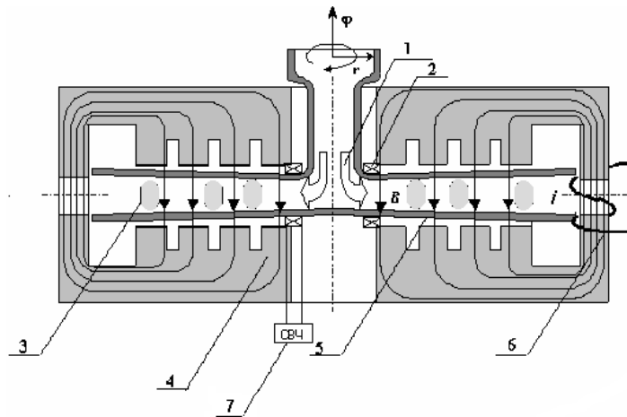
Figure 15. Inductive MHD Generator
