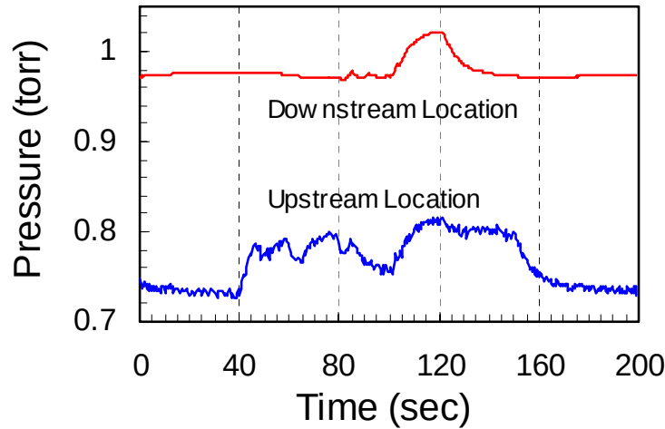
Fig. 5 Static pressure log of magneto-aerodynamic interaction Ref. [42]
