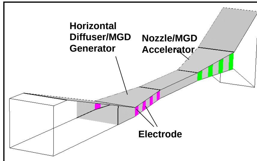
Fig. 8 Sketch of the MFD Scramjet bypass
