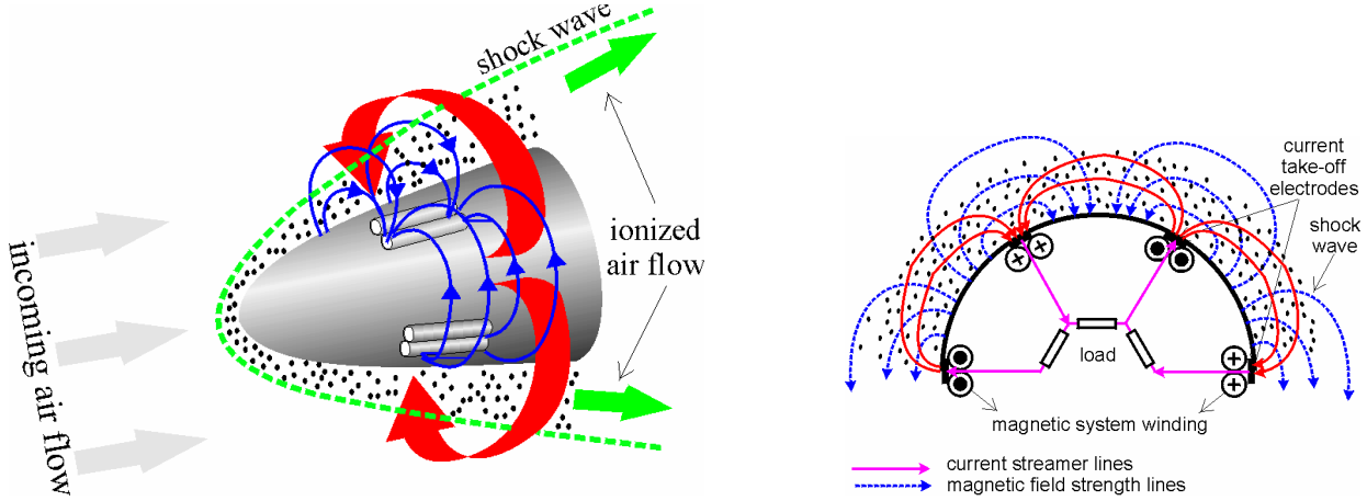
Figure 8 The schematic of the multipole magnetic system installed on a hypersonic spacecraft.
