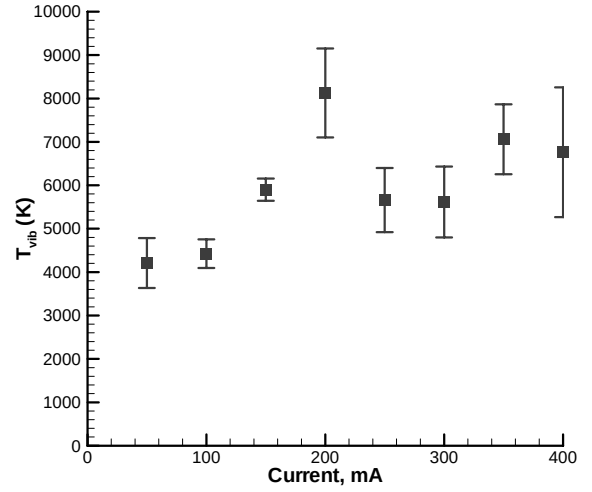
Figure 23 Vibrational temperatures for DC discharges between plates, at x / x_p = 0.7 , y / y_p = 0.0 as a function of discharge current.
