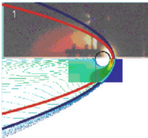
Fig.18. The comparison of the visualization of the flow during MHD interaction (upper) with 2D calculated temperature distribution and Billig' correlation (1 - M=15 and 2 –
