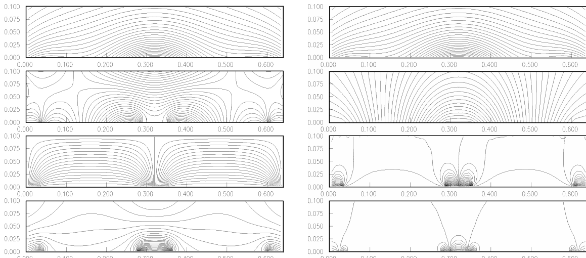
Figure 10. Magnetic Field Strength Lines, Electrical Potential, Electrical Current Stream lines (, and Body Force Distributions. Open Circuit Condition (left) and Short Circuit Condition (right).
