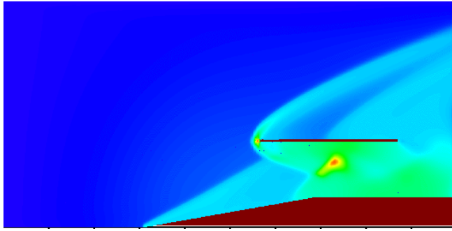
Figure47. Pressure distribution for the conditions of Run 138. Magnetic field 1.75T at the lead surface.
