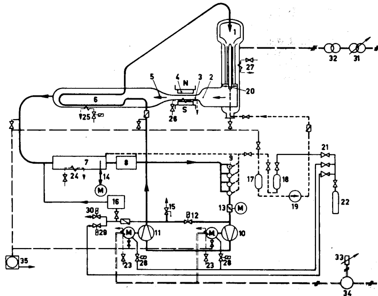
Fig. 4. From [4]. CNEN blow down facility.
