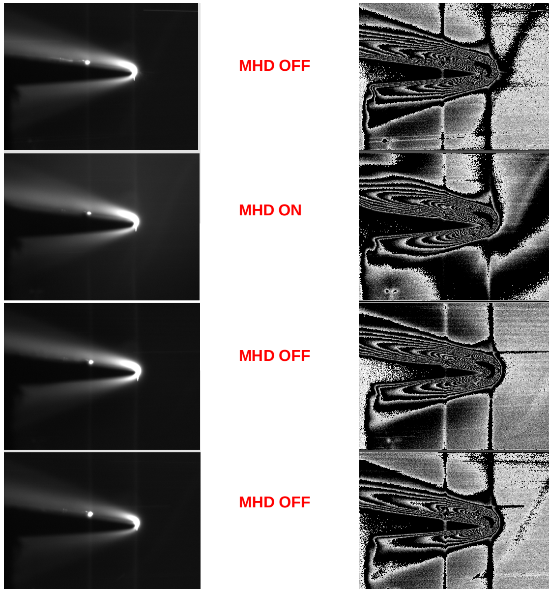
Figure 35. The visualization of flow around the wedge model. Run 131 04.24.2003. Flow from the right to the left. Four consequence frames are presented. Digital camera Pulnix-6710, 250fps, exposure time 30 mks. The left column is original imaging, the right column is the filtered image.
