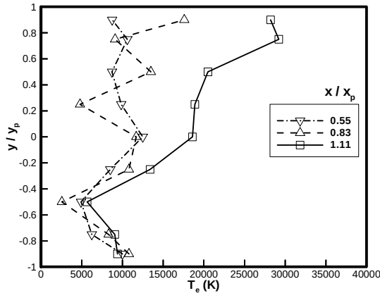
Figure 13 Electron temperatures measured in a 50 mA discharge, flow-on case.
