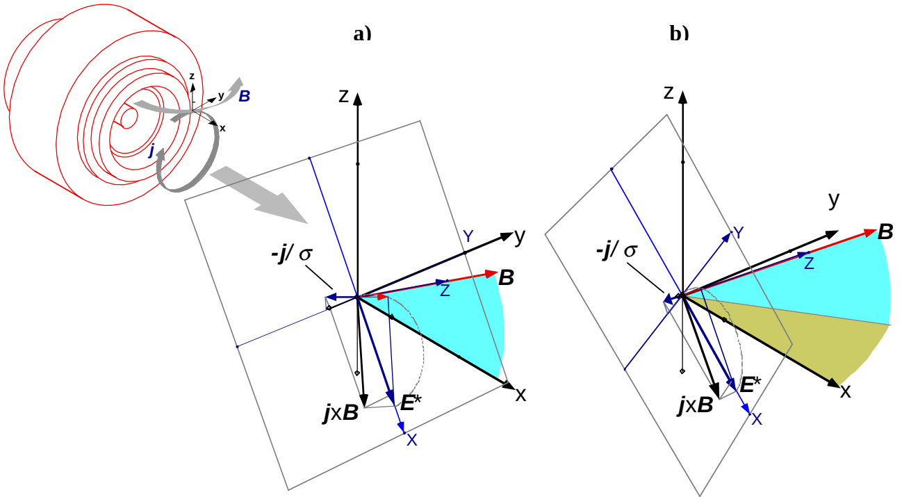
Fig. 8 Vector diagrams for applied-field MPD thruster
