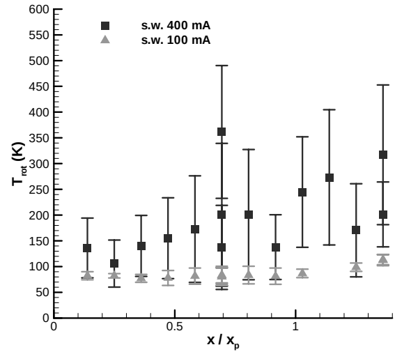
Figure 19 Rotational temperatures for 100 and 400 mA DC discharge between plates, streamwise distribution at y/y_p = 0.0 .
