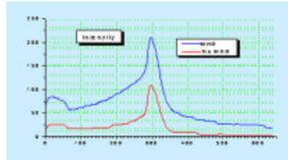
Fig.20. Intensity distribution along the flow direction for non-MHD (lower) and MHD (upper) cases. The maximum intensity is located up-stream of the leading edge of the cylinder. The leading and tailoring edges locations can be recognized from well visible curve broken.
