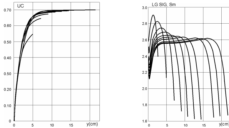
Figure 6. Relative Velocity Profile and Electrical Conductivity across Shock Layer for 10 Different Location along Streamline. Conditions: U=10\text{km/s} , H=80\text{km} , j=45^\circ , R=0.4\text{m} .
