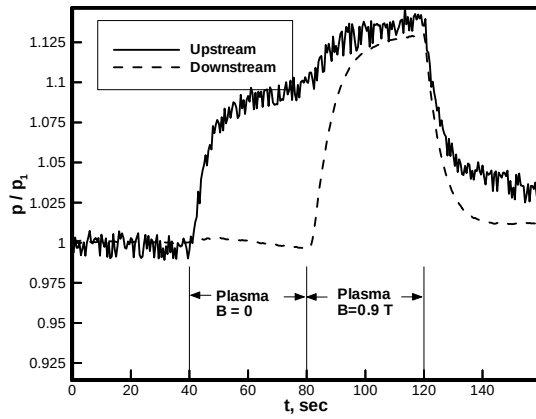
Figure 26 Surface pressures between crossflow electrodes for a 50 mA discharge.
