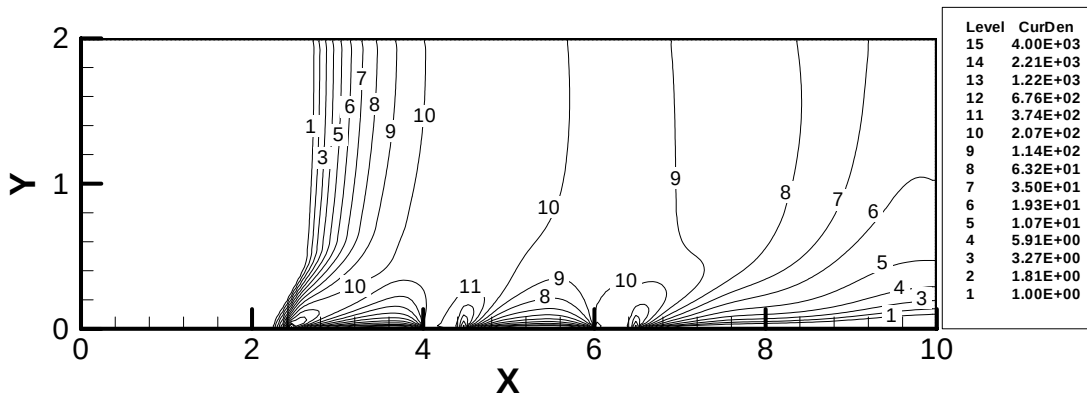
Fig. 4 Computed current density in 2-D discharge channel with segmented electrodes
