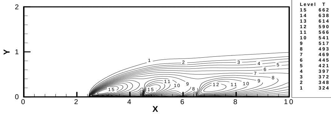
Fig. 5 Temperature distribution in 2-D discharge channel with segmented electrodes
