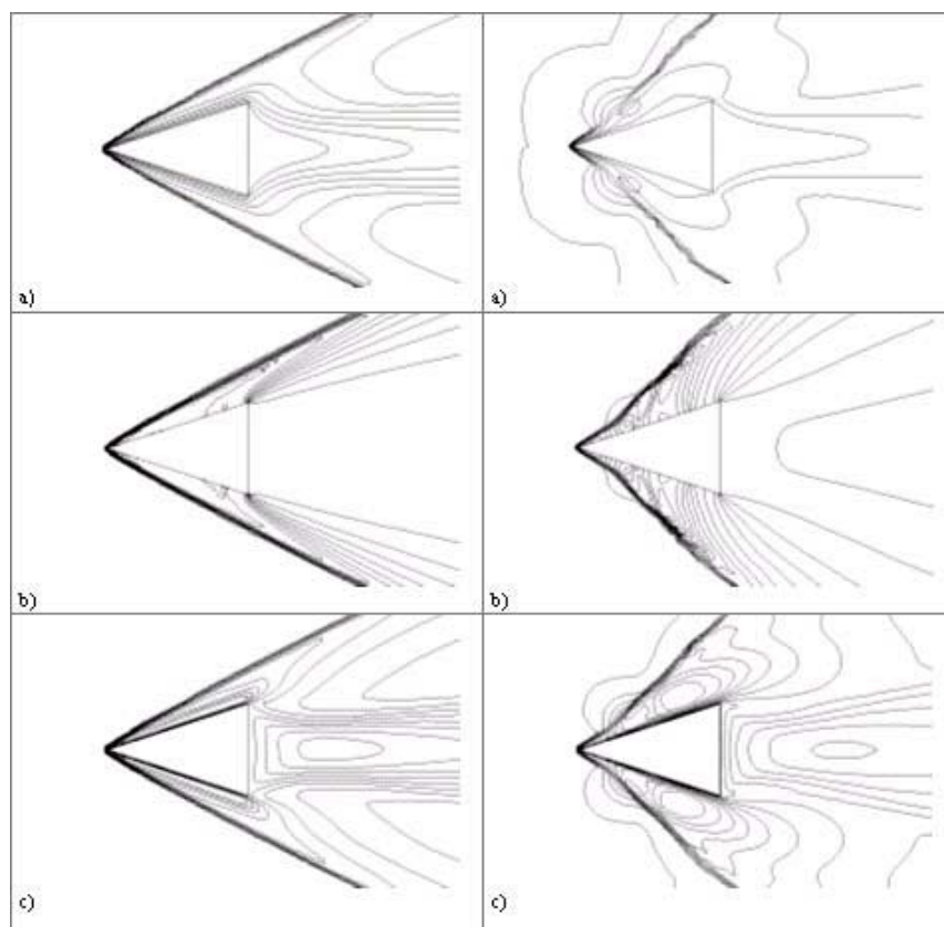
Figure 13: MHD interaction of a wedge body in an hypersonic flow.
