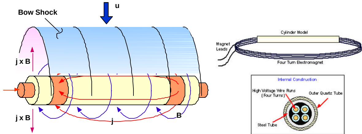
Figure 13 Schematic of MHD flow over the circular cylinder with axial electric current and the model design concept.
