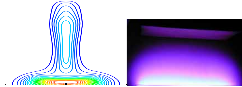
Fig. 6 Computed glow discharge and experimental results
