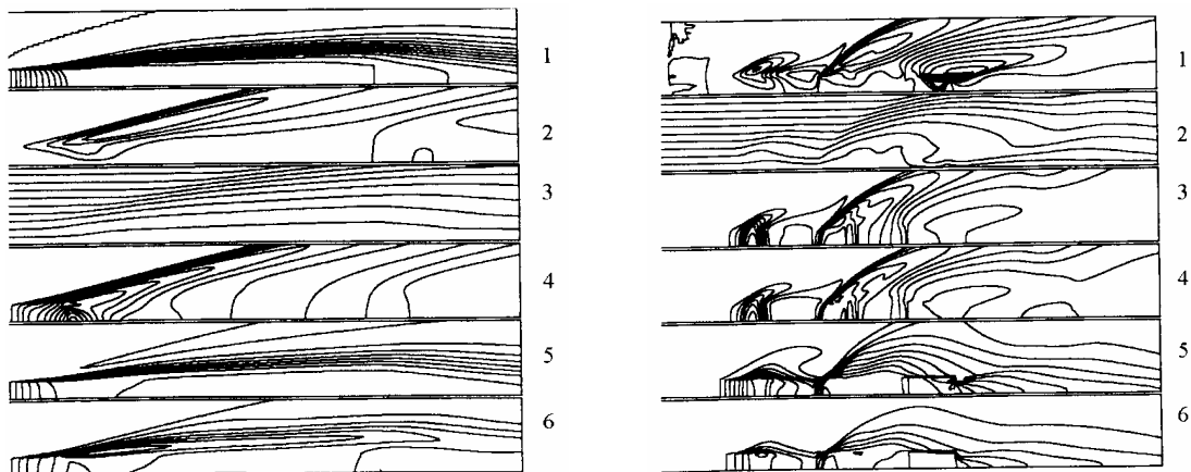
Figure 12. Flow Field Numerical Simulation Results . "Shock free case".(left) "Multi Shock case".(right).
