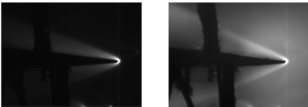
Figure 4 Flow over a wedge. MHD-off (left), MHD-on (right)
