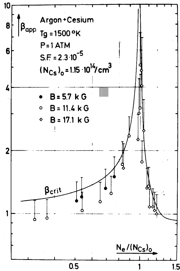
Fig. 24. From [19]. Effect of fully ionized seed on Hall parameter.
