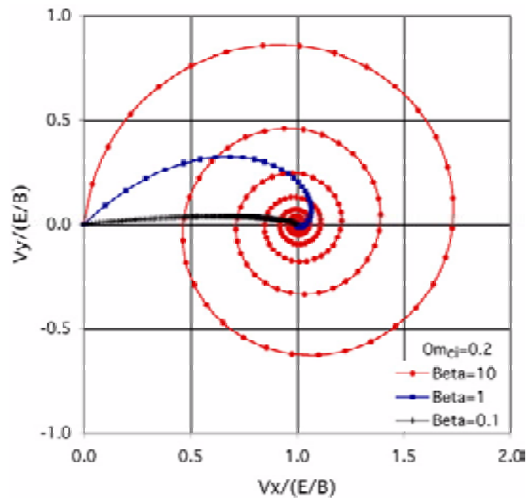
Fig. 2a Representative solutions of electromagnetic equations
