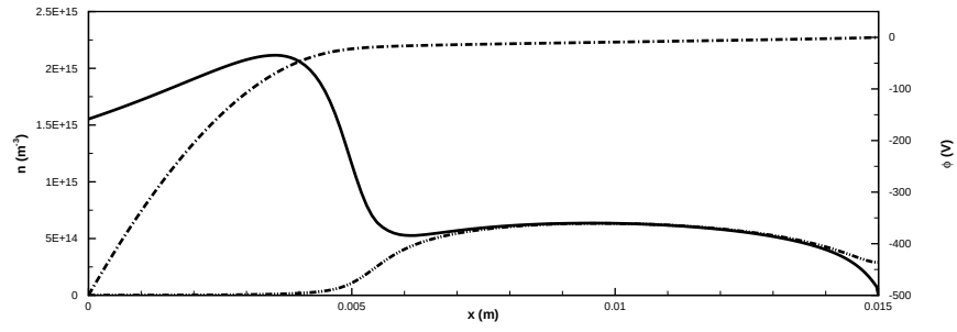
(b) Applied potential 500 V.
