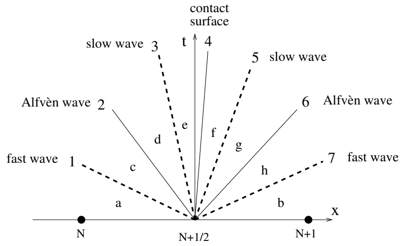
Fig. 8 Riemann problem for the MFD system.
