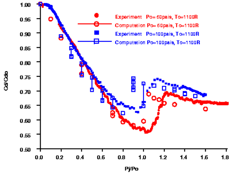
Fig. 4. Comparison of drag reduction via plasma injection
