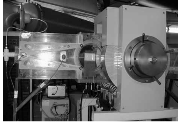
Figure 24 Electromagnet installed around channel.
