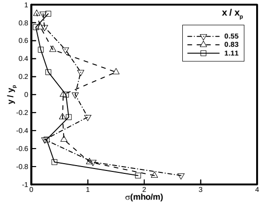
Figure 15 Plasma conductivity measured with the Langmuir probe in a 50 mA discharge, flow-on case.
