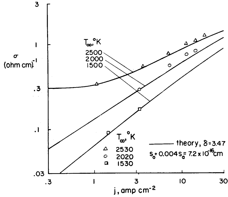
Fig. 2. From [1].Electrical conductivity vs. current density, demonstrating the effect of electron temperature elevation.
