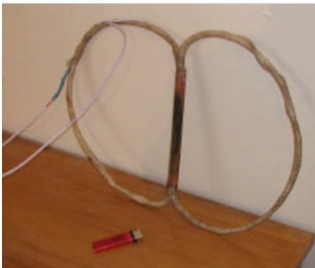
Fig16. The modified Double-Oval model
