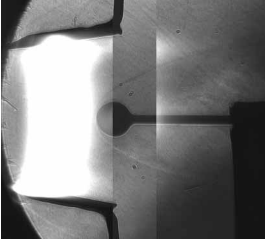
Figure 18 Schlieren image of shock produced by a sphere in the presence of a DC discharge. Luminosity from the discharge is evident between the plate electrodes on the left. The darker vertical strip in the middle is the superimposed schlieren image in the absence of a discharge.
