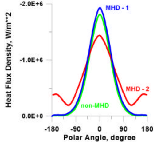
Fig.32. Heat Flux Density vs polar angle for three cases: non-MHD stands for reference case of a conventional flow; MHD-1 presents the result for the shorter conditions case; and MHD-2 – for the non-shorter conditions case.
