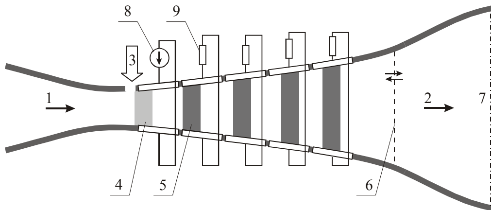
Figure 13. Scheme of MHD generator. 1 – stationary flow of unseeded noble gas; 2 – working medium flow with periodical disturbances; 3 – electron beam; 4 – weakly ionized plasma clot; 5 – recombining plasma layer; 6 – shock wave; 7 – outlet cross section with constant stagnation pressure; 8 – high voltage source; 9 – load.
