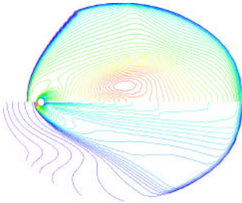
Fig.31. Temperature distributions for the conditions of Fig.30.
