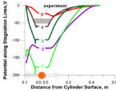
Fig.24.. The stagnation line electrical potential distribution for different ionization degrees in oncoming flow. 1 - 10^{-4} ; 2 - 10^{-2} ; 3 - 10^{-4} ; 4 - 5 \cdot 10^{-3} ; 5 - 10^{-2} .
