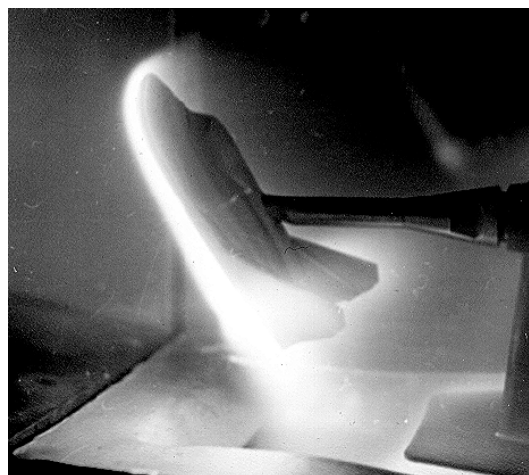
Figure 20. An example of visualization of the hypersonic viscous shock layer- on a TAV model.
