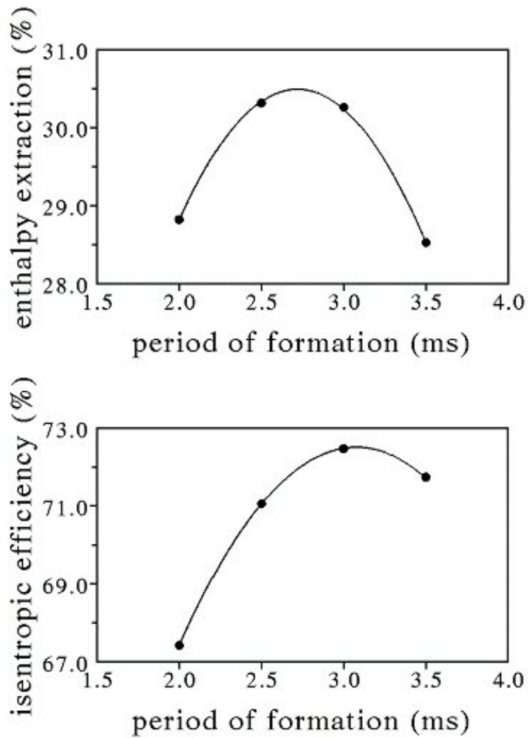
Figure 5: Enthalpy extraction and isentropic efficiency vs. T-layer formation period.
