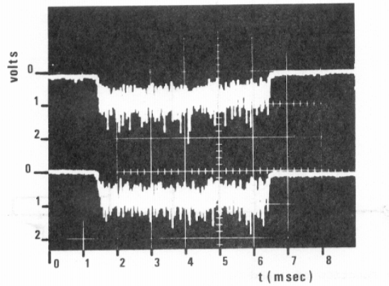
4.3.1.1 Fig. 12. From [9]. Time resolved recombination radiation signals
