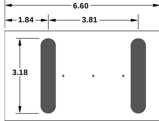
Figure 8 Schematic of flat plate model. All dimensions cm. Electrodes are 0.64 cm wide. Pressure taps are spaced 1.27 cm, starting at x = 2.48 cm.
