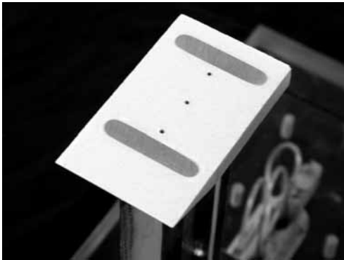
Figure 7 Flat plate model with electrodes and pressure taps
