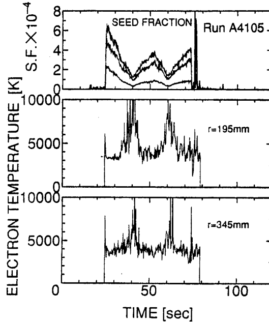
Fig. 27. From [21]. Variation of seed fraction and electron temperature during a blow-down run
