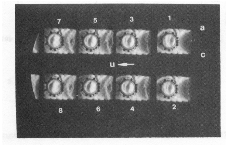
Fig. 23. From [16]. Framing pictures of the inlet relaxation region, showing initial breakdown.
