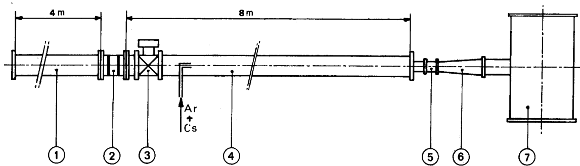
Fig. 3. From [3]. Schematic of shock tube facility. 1) driver section 2) diaphragm section 3) ball valve 4) test section 5) preionizer 6) generator 7) vacuum tank.
