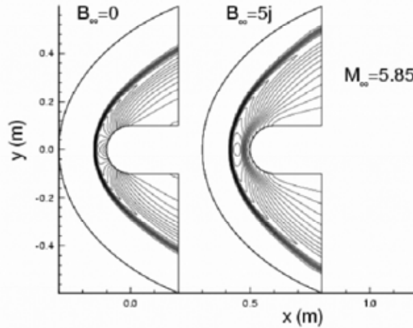
Fig. 1 Blunt body standoff distances in electromagnetic field, (Ref. 20)
