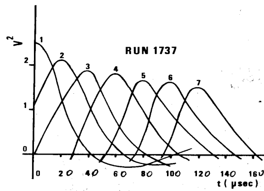
Fig. 15. From [9]. Cross correlation between electrode currents.
