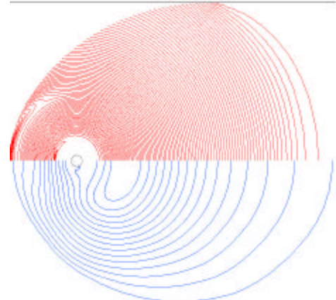
Fig.26. The equipotential lines are as for non-shorted (red, upper half) and shorted (blue, bottom half) conditions.
