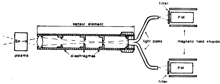
Fig. 8. From[8]. Set-up for recombination radiation measurement.
