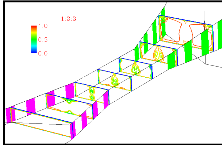
Fig. 7 Cross-flow in MHD scramjet flow path, Courtesy of Gaitonde (Ref.53)
