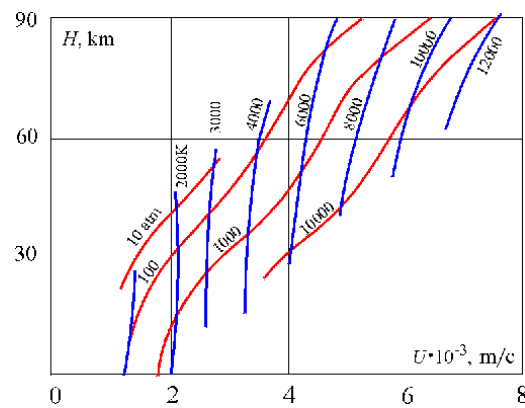
Figure 18. Inlet wind tunnel parameters needed for modeling flight conditions and calculated for adiabatic nozzle expansion
