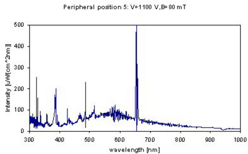
Figure 9: Emission spectra of the plasma of the MPD thruster.
