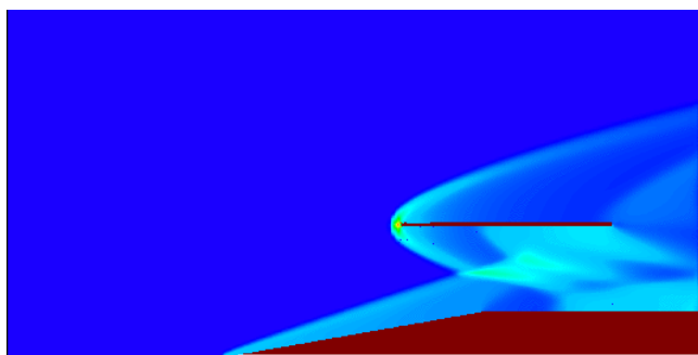
Figure 46. Pressure distribution with no Magnetic field under conditions of the Run 138.
