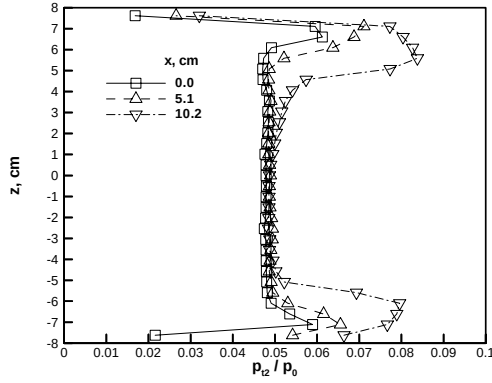
Figure 4 Vertical survey of Pitot pressure, normalized by stagnation pressure, at three axial stations.
