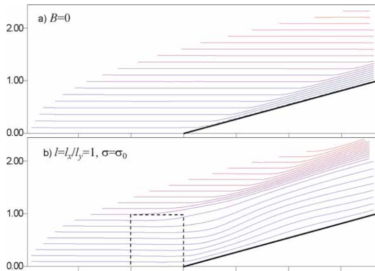
Figure 5 Streamlines for N=0.23 (b) compared to the flow over the wedge without MHD effects (a); \sigma_0=1.15 S/m.
