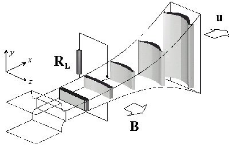
Figure 3: T-layer MHD generator.
