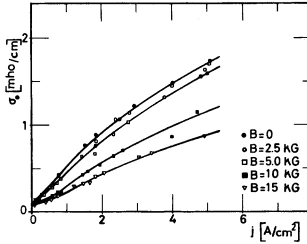
Fig. 10. From [6]. Electrical conductivity vs. current density for several values of magnetic induction.
