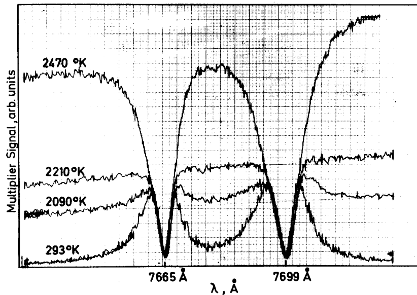
Fig. 7. From [7]. Line reversal measurement set-up and result.
