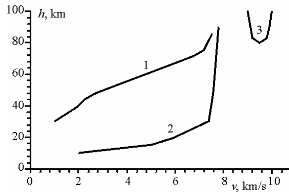
Figure 1 Typical Spacecraft Trajectories.
