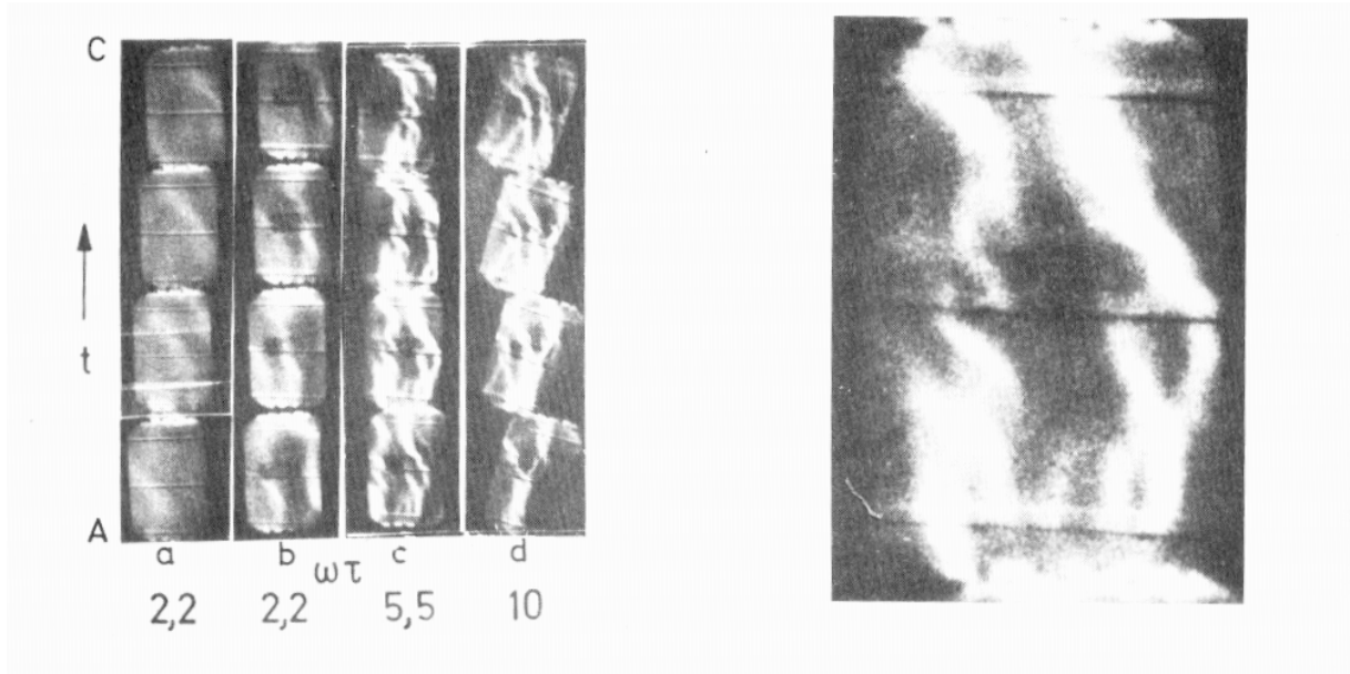
Fig. 16. From [10]. Image converter pictures of streamers.
