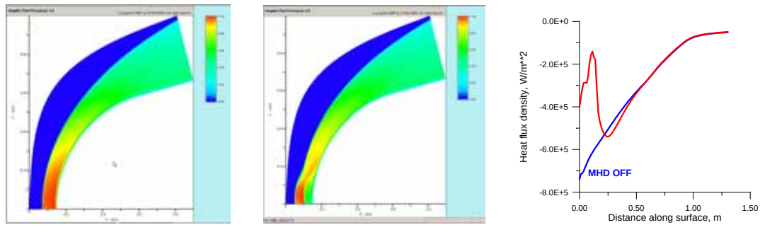
Figure 3 Re-Entry MHD Interaction Evaluation. Temperature Distribution for MHD-off (left) and MHD-on (center) operation; Corresponding Heat Flux Distribution along the Flow (right).
