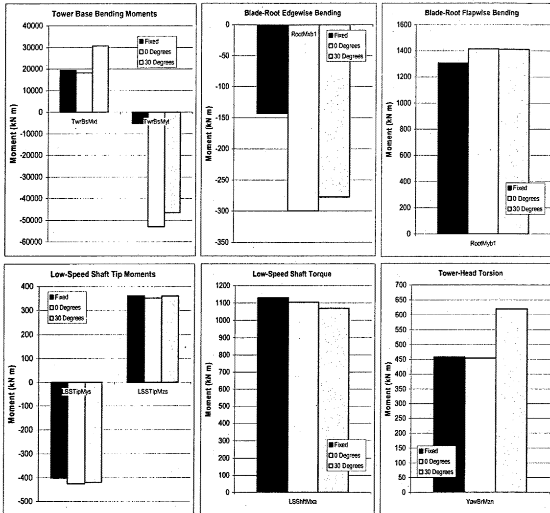
Figure 9.17 Maximum wind turbine loads during extreme wave tests. Wind turbine secured. Blade pitch = 90^\circ . Reference speed of 20 m/s. Incident wave amplitude = 10.68 m. Incident wave period = 11.62 seconds. 1) Fixed base (only wind loading), 2) floating (incident wave angle = 0^\circ ), and 3) floating (incident wave angle = 30^\circ )
