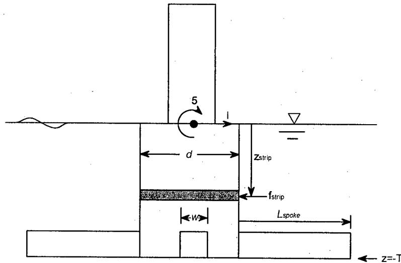
where a_{strip} is the acceleration of the strip being analyzed due to both translation and rotation at the point around which the added mass is being determined. The two dimensional added mass term for a cylindrical strip is equal to the volume displaced. Next the contribution of the spokes is added to the surge added mass.
