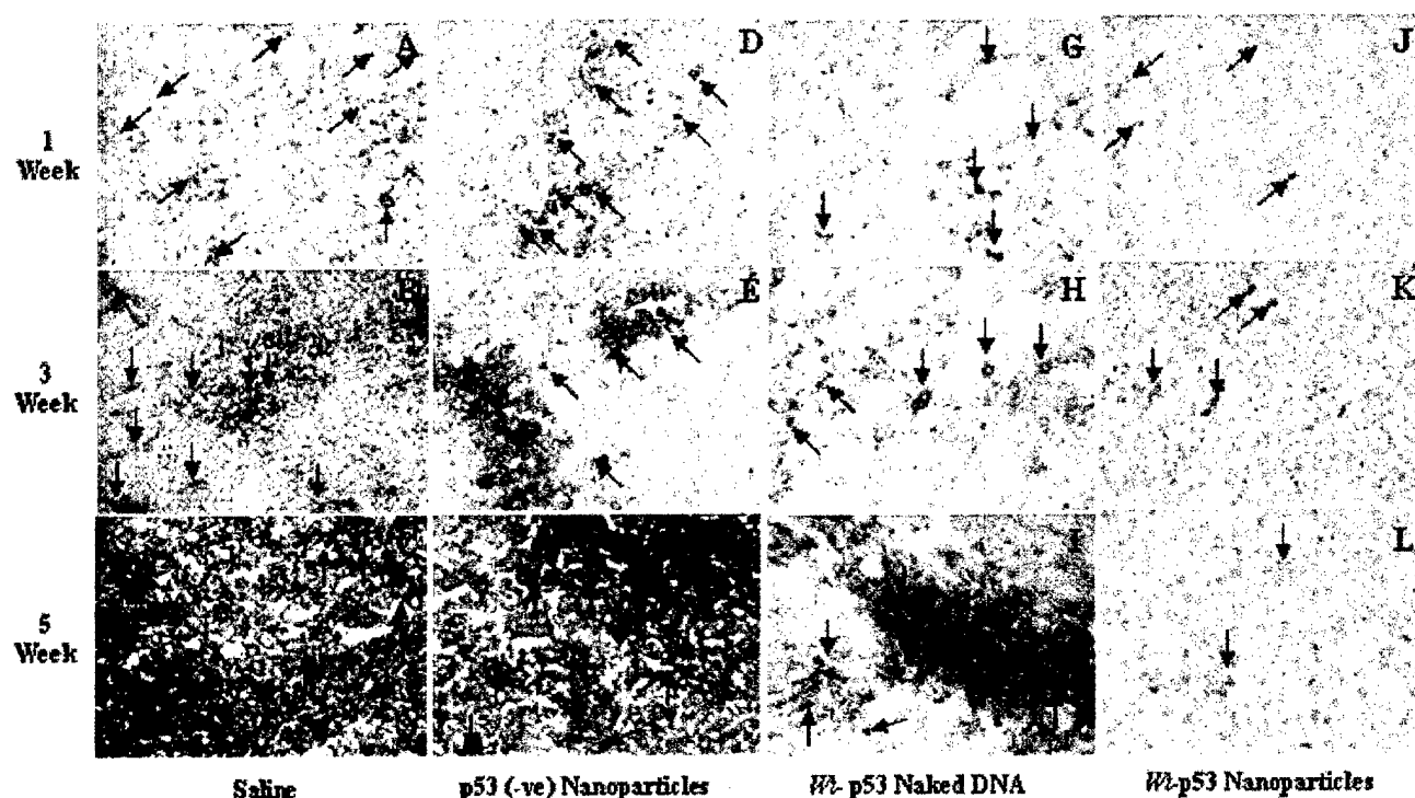
Figure 11. CD-31 staining to determine effect of various treatments on angiogenesis in tumor tissue. A, D, G and J represent 1 week data for respective groups. B, E, H and K represent 3 week data for respective groups and C, F, I and L represent 5 week data for respective groups. Arrows indicate the blood vessels
