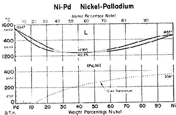
Fig. 1 Phase diagram for Nickel-Palladium alloy. Also shown is the Curie temperature that can be controlled by controlling the Nickel composition in the alloy.
