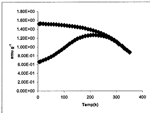
Fig 6. FC and ZFC curves for Ni-Pt (CTAB= 0.1M) after heating at 700 0 C.
