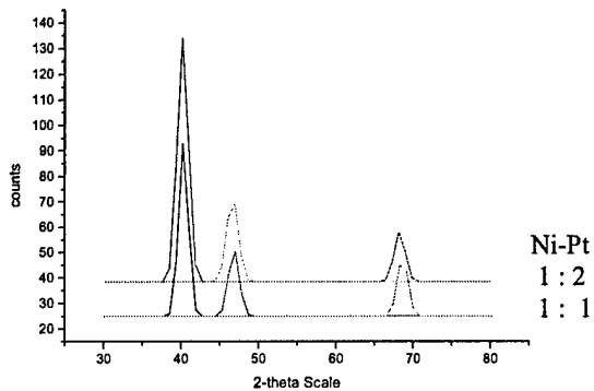
Fig 1. XRD patterns for Ni-Pt nanoalloy
