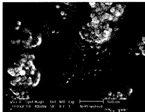
Fig 2. SEM for Ni-Pt (1:2) nanoalloy
