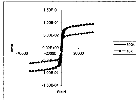
Fig 7. Hysteresis loop at 10K and 300K for Ni-Pt (CTAB=0.1 M) nanoalloy, after heating at 700 0 C.
