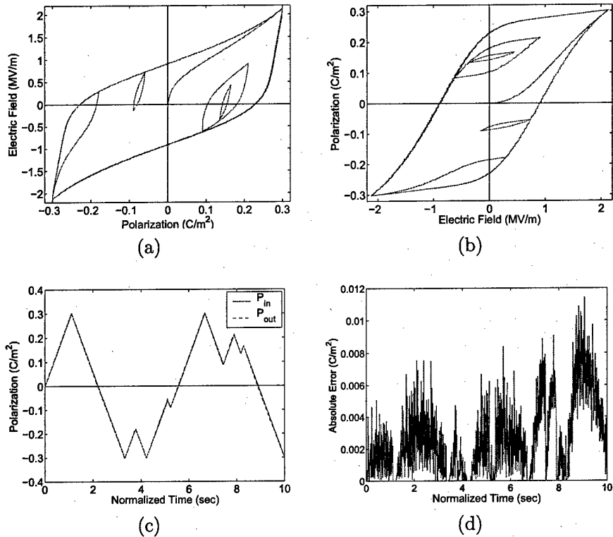
Figure 4: (a) Inverse relation P_{in}-E_{out} , and (b) forward relation E_{out}-P_{out} . (c) Comparison between P_{in} and P_{out} , and (d) absolute error |P_{in} - P_{out}| for complete inversion process.
