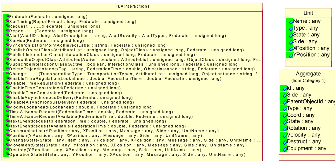
Figure 2: MSCombat FOM Class Diagram.
