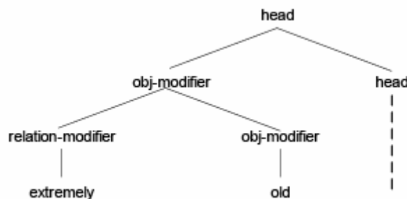
Figure 14 Integrating a relation modifier with an object modifier
