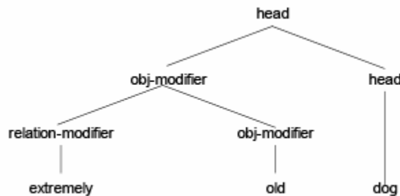
Figure 15 Integrating a head with an object modifier
