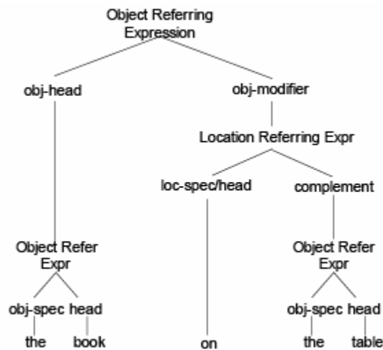
Figure 2 An object referring expression with a post-head modifier
