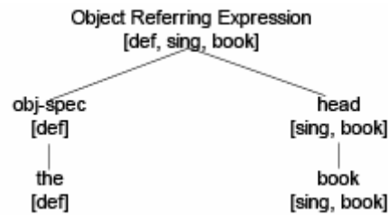
Figure 10 More specific conceptual features
