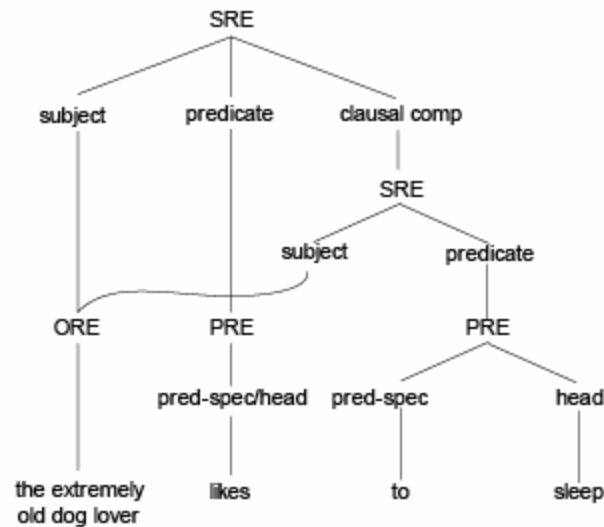
Figure 21 Integrating two relational head schemas
