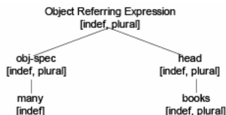
Figure 6 Overlapping grammatical features
