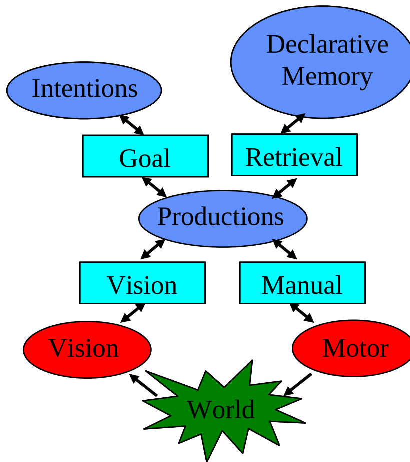
Figure 24 The ACT-R Architecture
