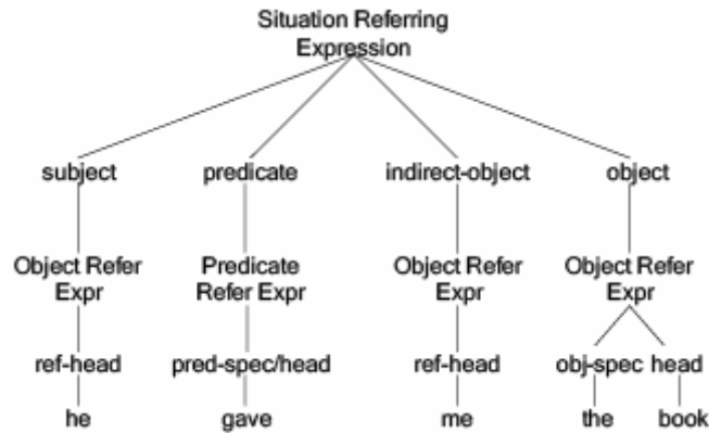
Figure 1 A situation referring expression with multiple complements
