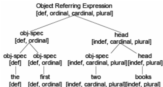
Figure 5 Adding grammatical features to the representation
