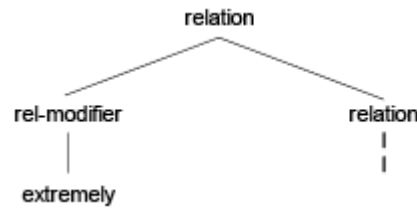
Figure 12 A relation modifier schema
