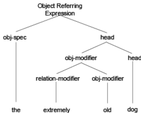
Figure 16 Integrating a specifier with a head
