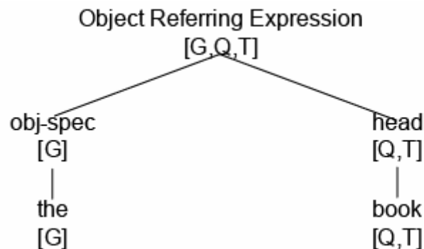
Figure 9 Adding abstract conceptual features
