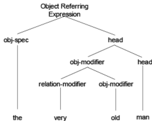
Figure 3 An object referring expression with a pre-head modifier
