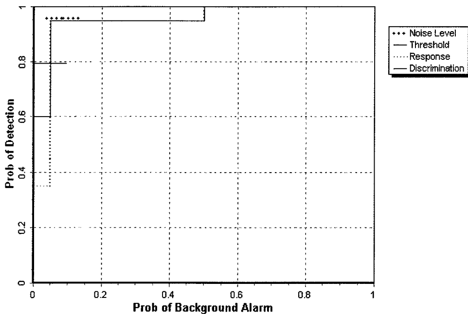
Figure 5. EM61 MKII blind grid probability of detection for response and discrimination stages versus their respective probabilities of background alarm for all ordnance larger than 20-mm.
