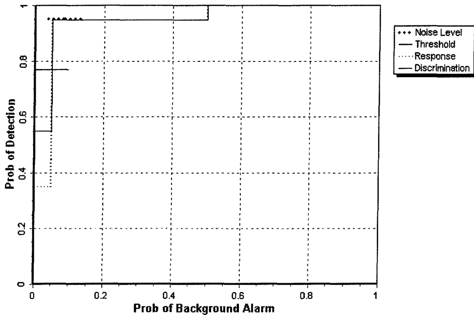
Figure 3. EM61 MKII blind grid probability of detection for response and discrimination stages versus their respective probability of background alarm over all ordnance categories combined.
