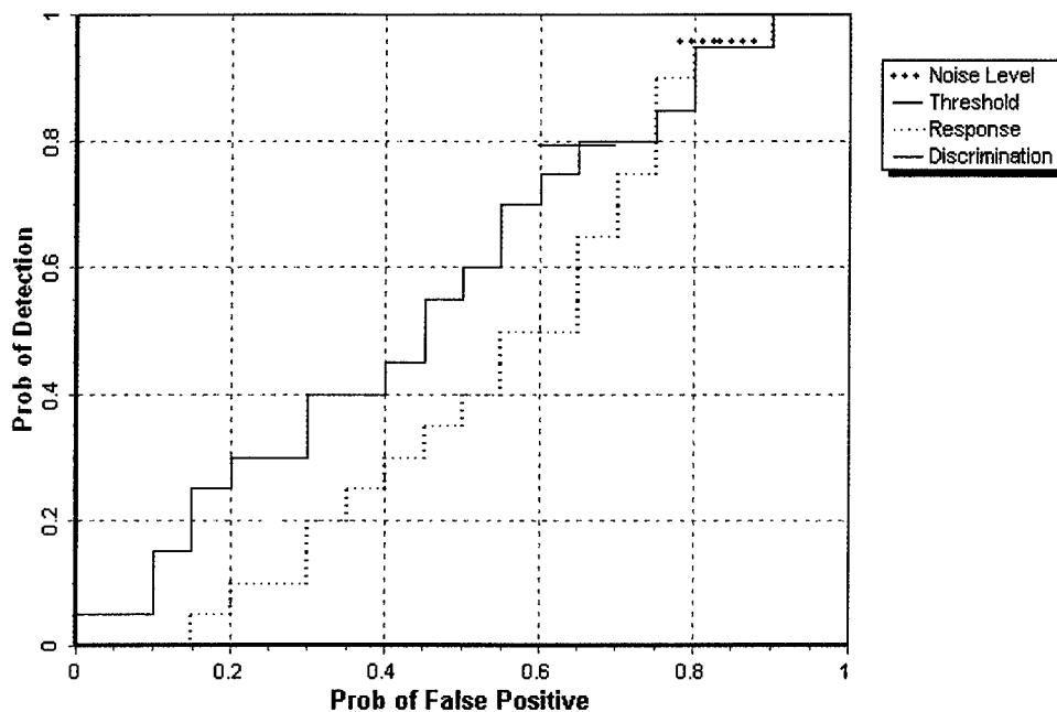
Figure 4. EM61 MKII blind grid probability of detection for response and discrimination stages versus their respective probability of false positive for all ordnance larger than 20-mm.
